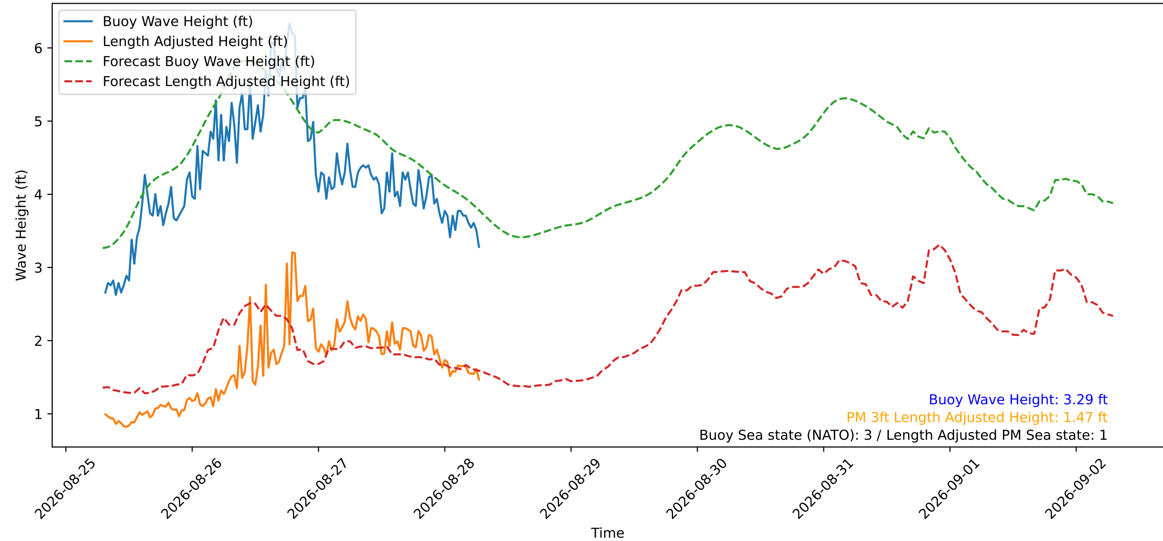
Wave Heights over Time for Green Beach at 2026-08-28 07:11:12
