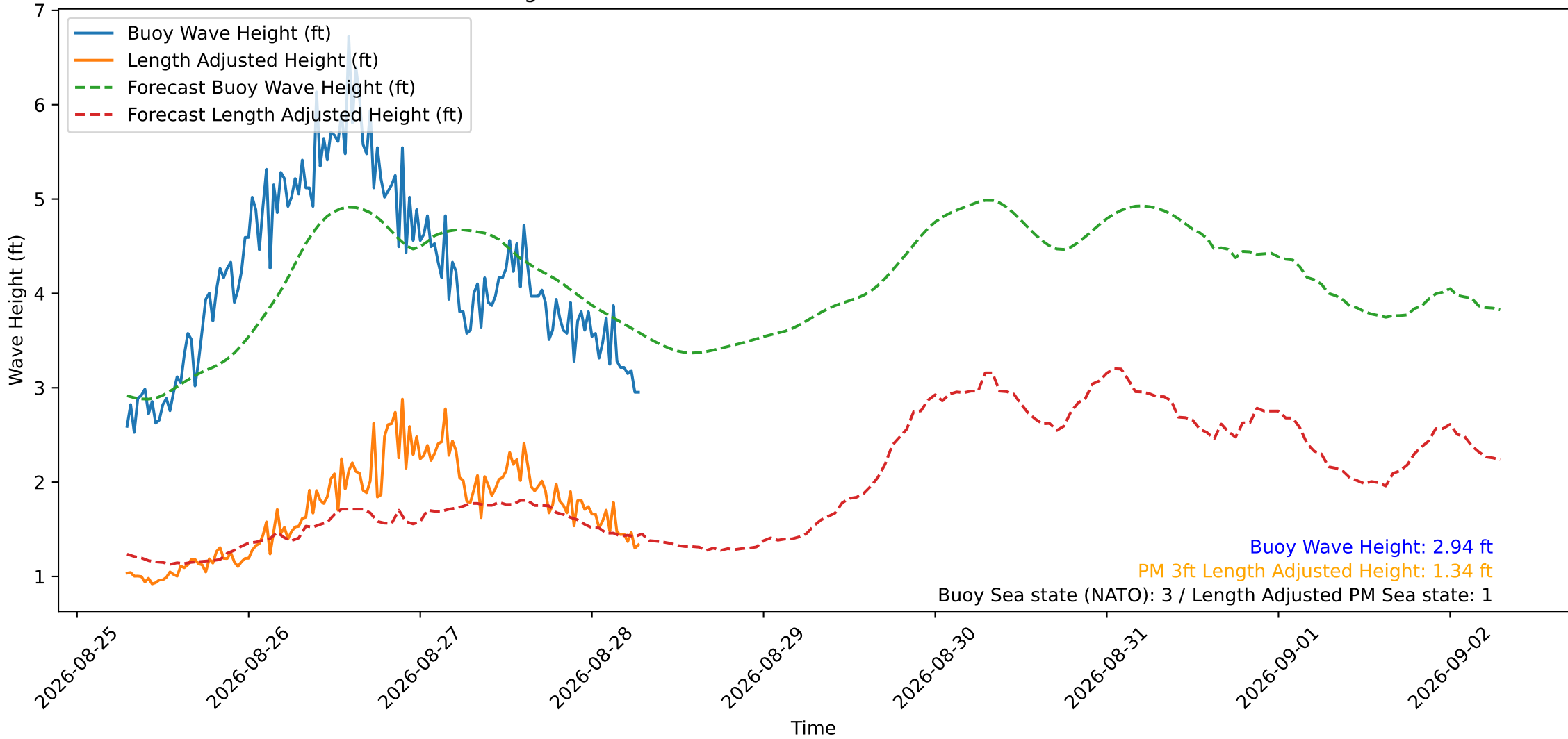
Wave Heights over Time for Oceanside Harbor at 2026-08-28 07:10:30
