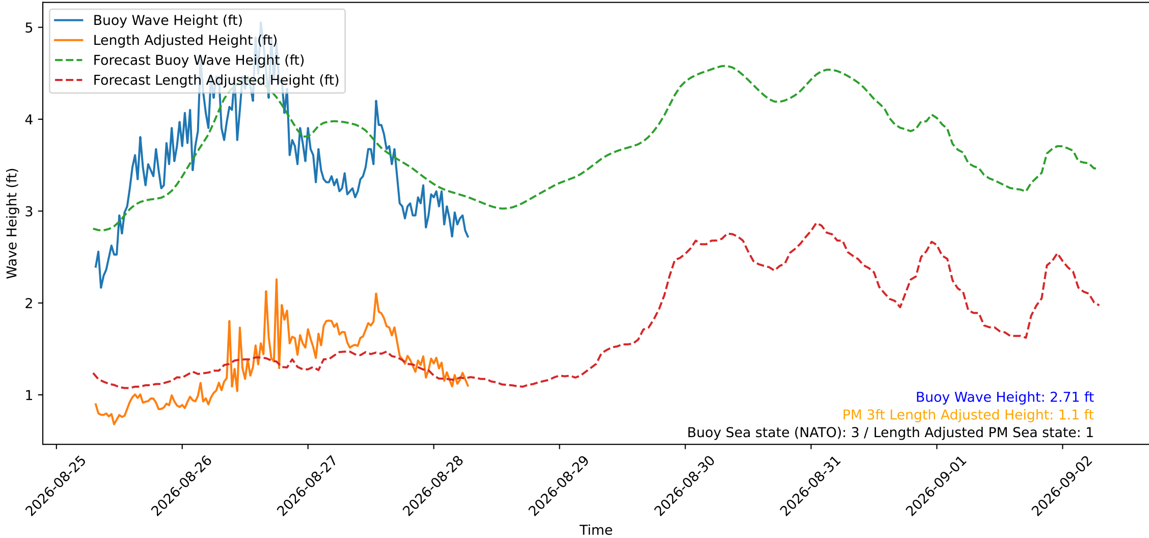
Wave Heights over Time for Red Beach at 2026-08-28 07:10:49
