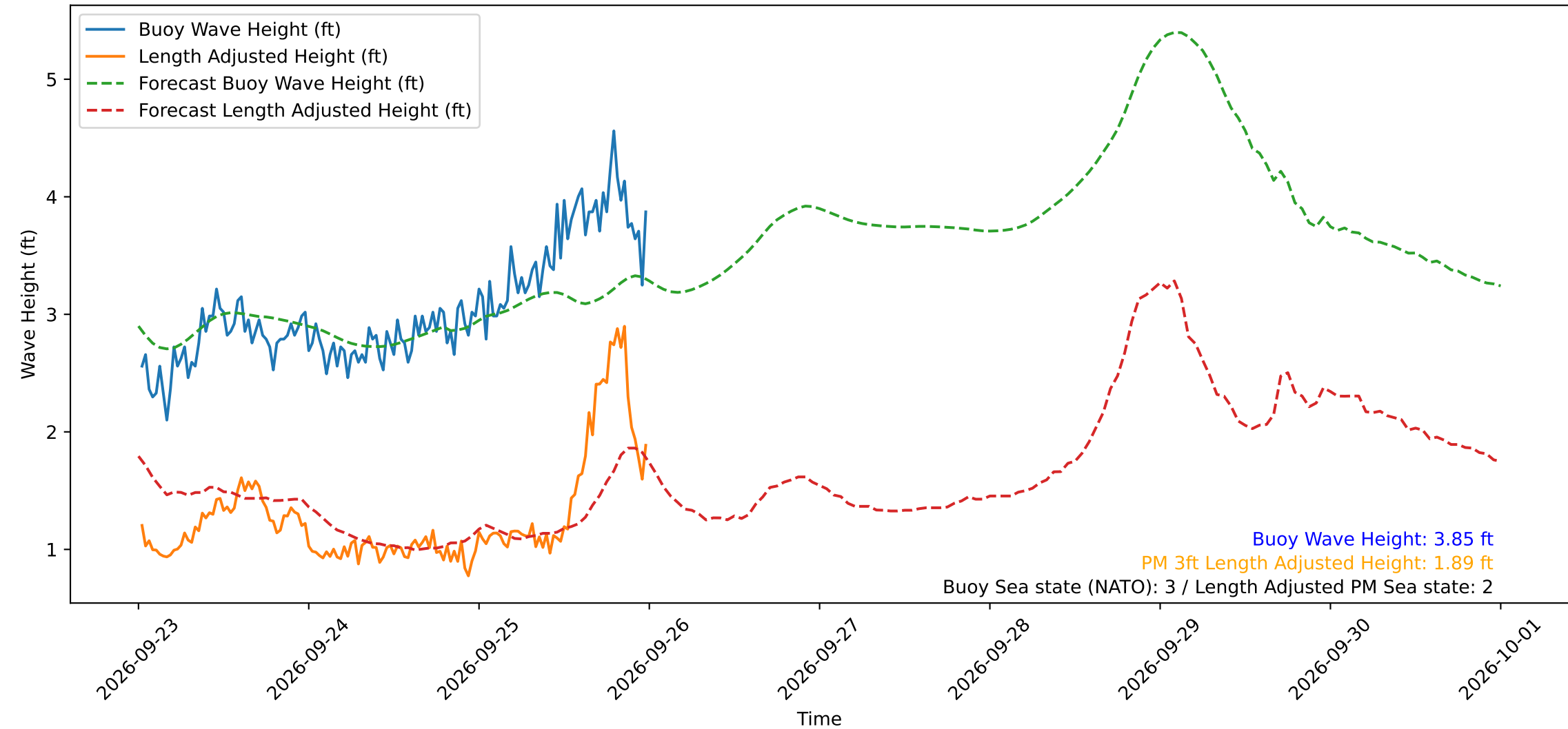
Wave Heights over Time for Green Beach at 2026-09-26 00:21:15
