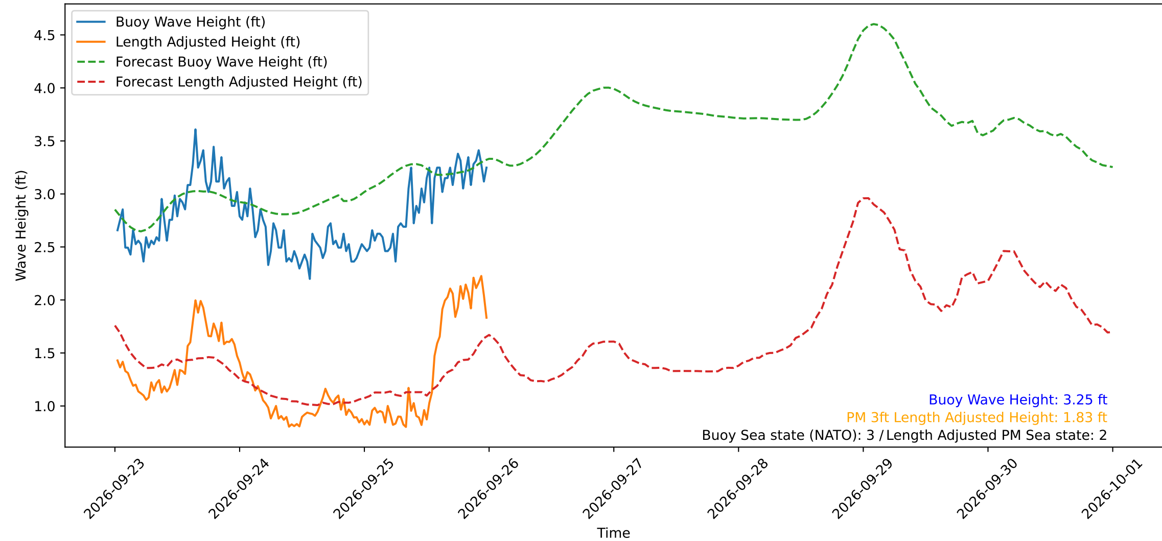
Wave Heights over Time for Oceanside Harbor at 2026-09-26 00:20:29
