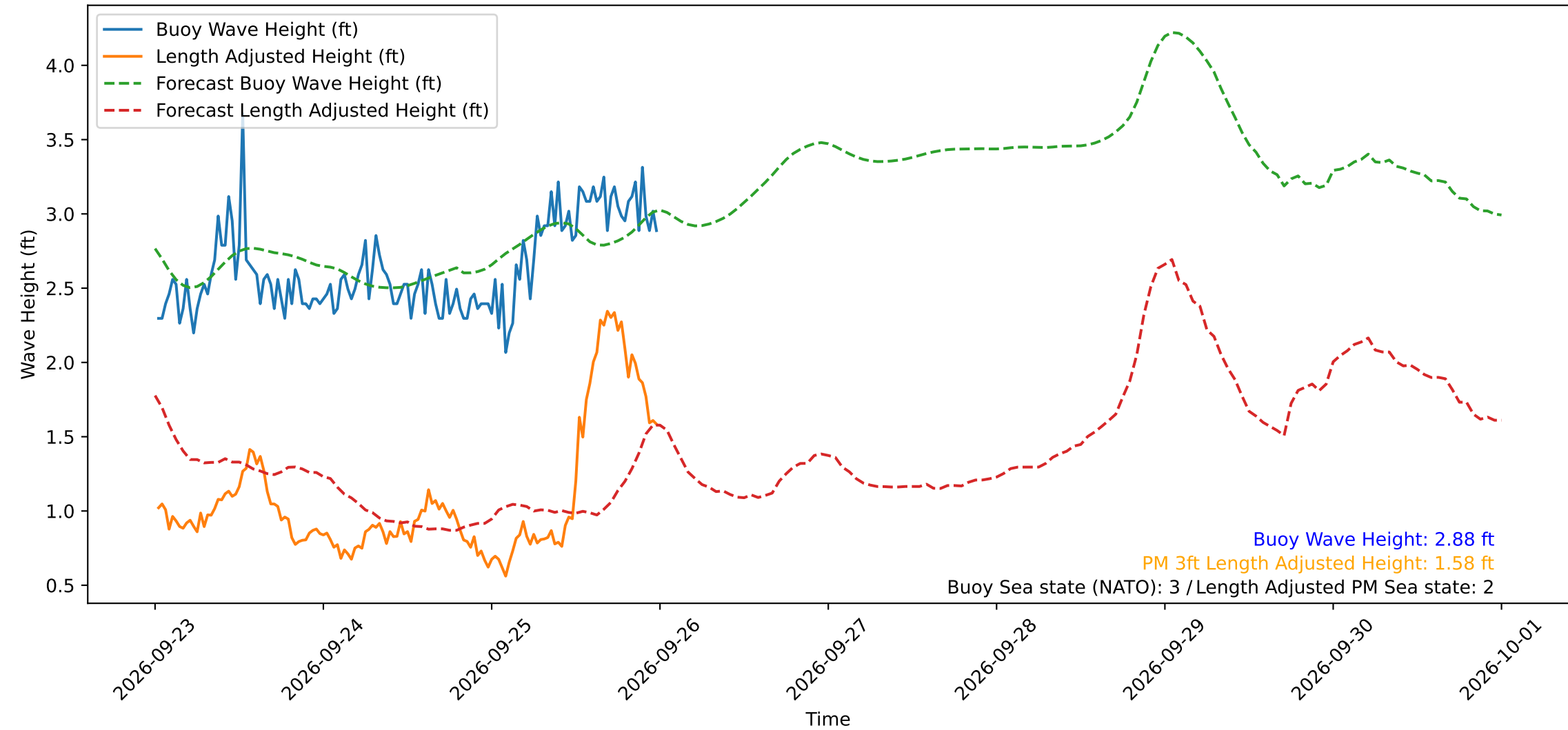
Wave Heights over Time for Red Beach at 2026-09-26 00:20:50
