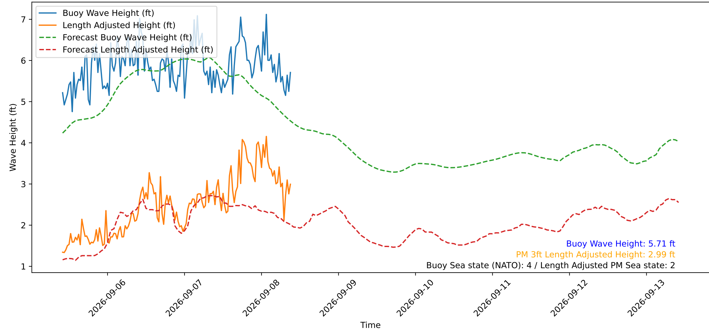
Wave Heights over Time for Oceanside Harbor at 2026-09-08 09:50:30
