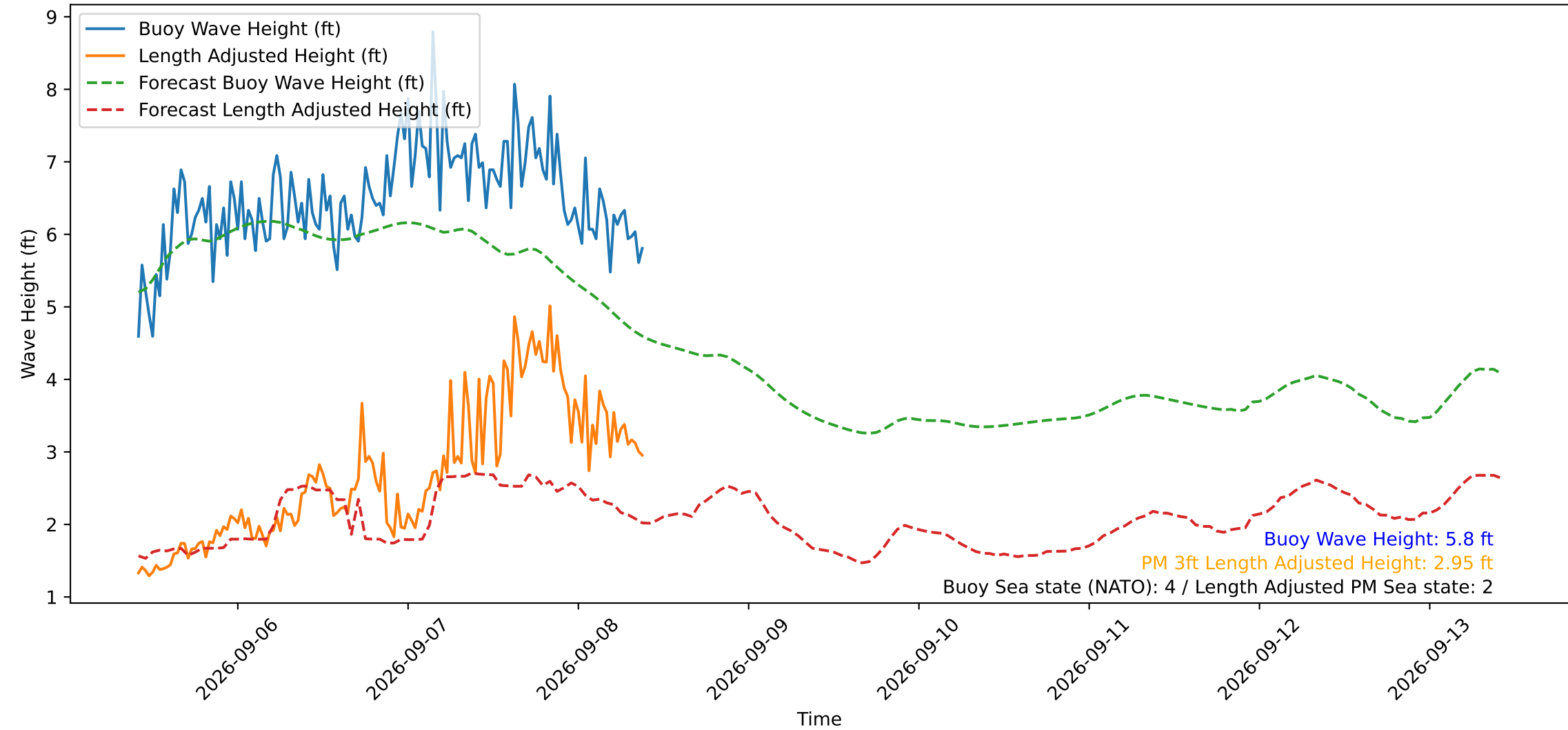
Wave Heights over Time for Green Beach at 2026-09-08 09:51:14
