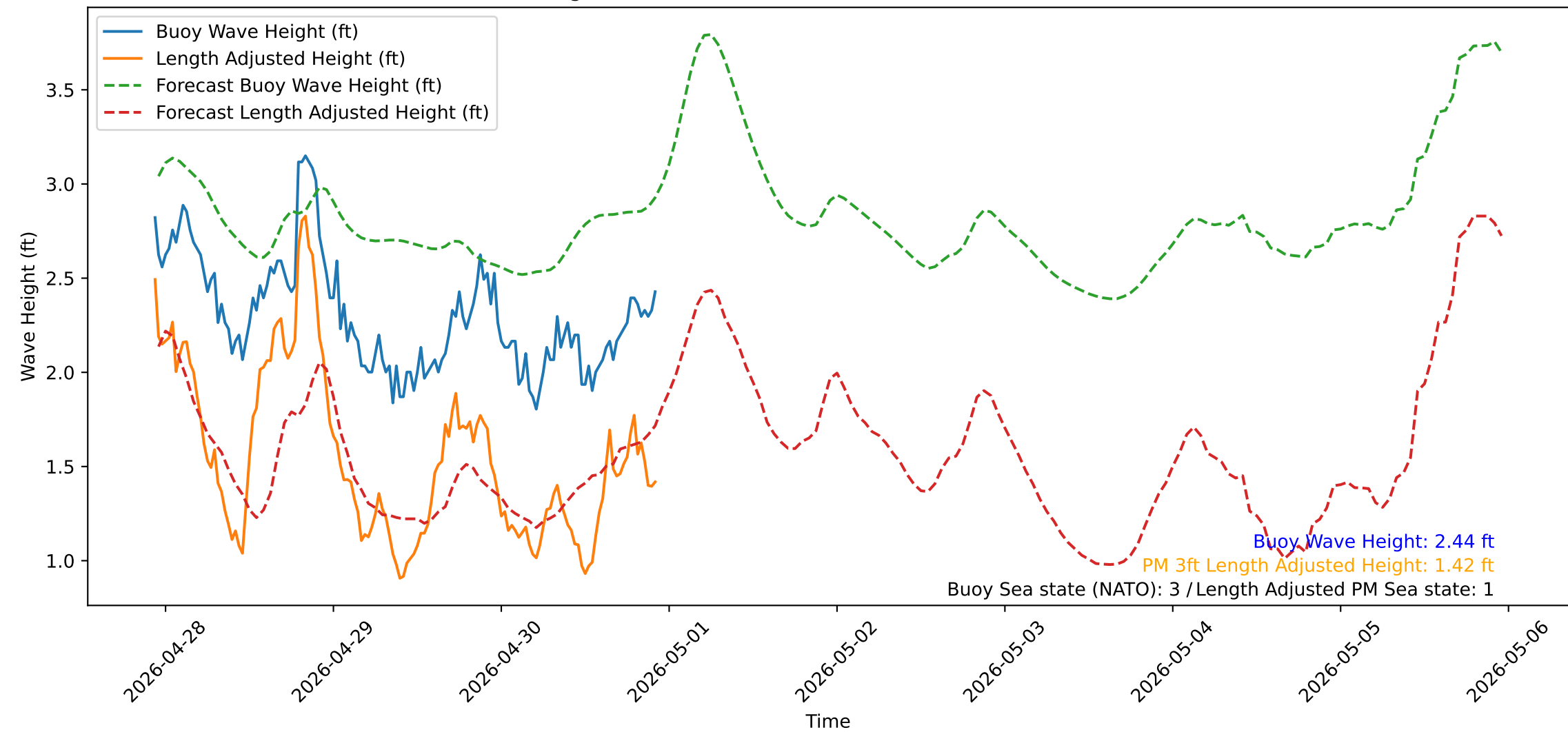
Wave Heights over Time for Green Beach at 2026-04-30 22:41:13
