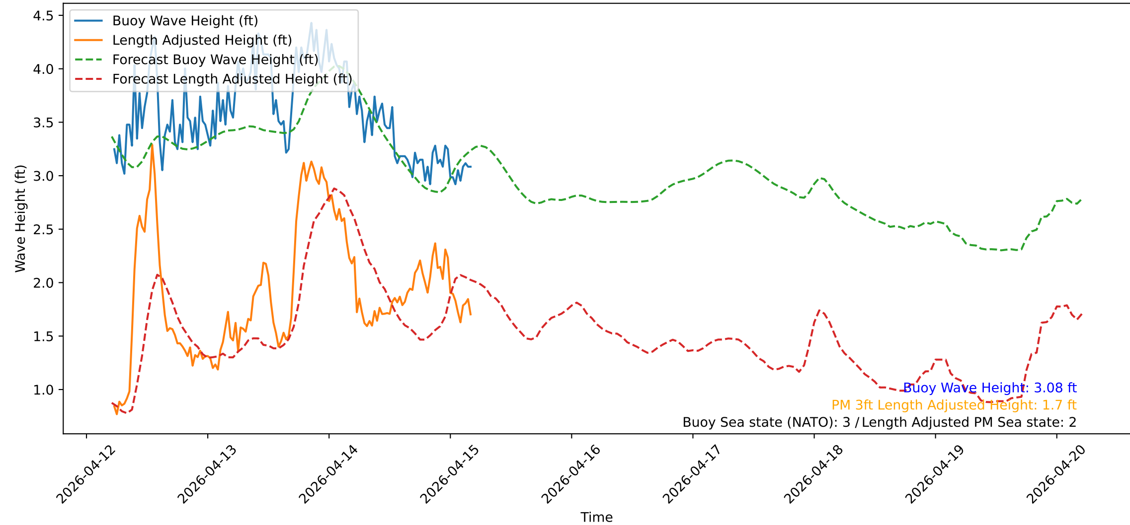
Wave Heights over Time for Red Beach at 2026-04-15 05:00:50
