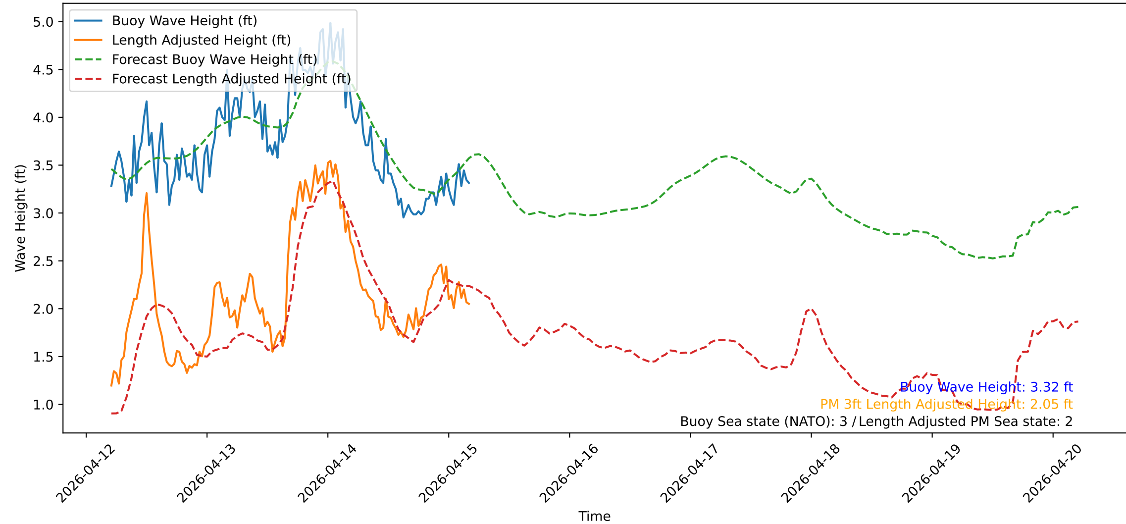
Wave Heights over Time for Green Beach at 2026-04-15 05:01:12
