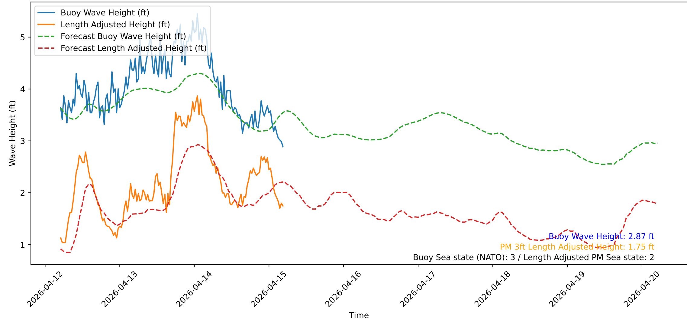
Wave Heights over Time for Oceanside Harbor at 2026-04-15 05:00:32
