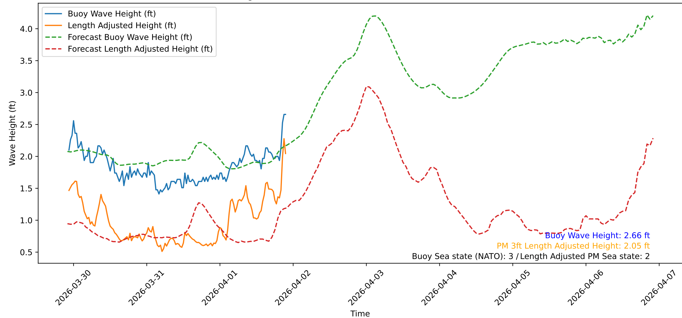
Wave Heights over Time for Green Beach at 2026-04-01 22:21:09
