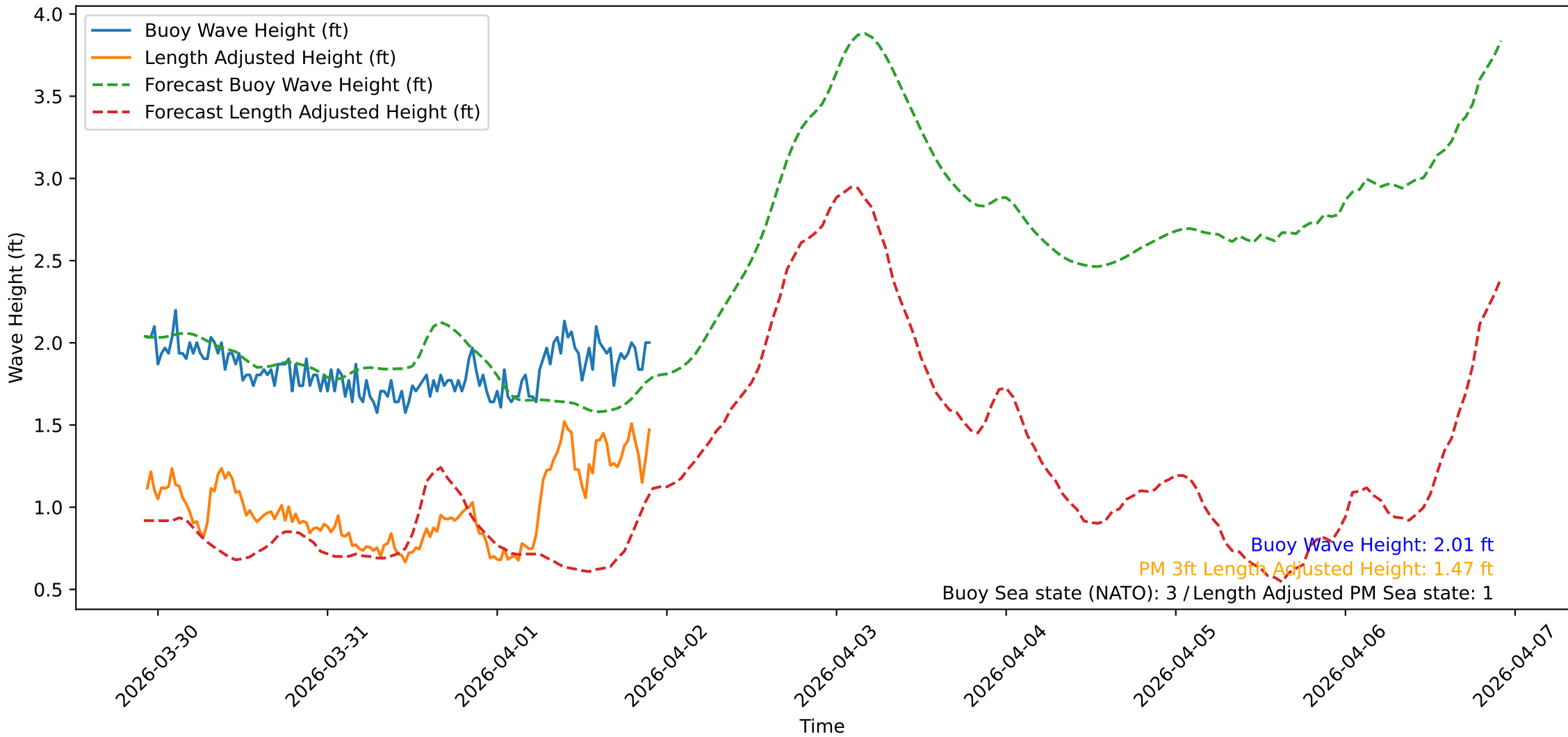
Wave Heights over Time for Oceanside Harbor at 2026-04-01 22:20:31
