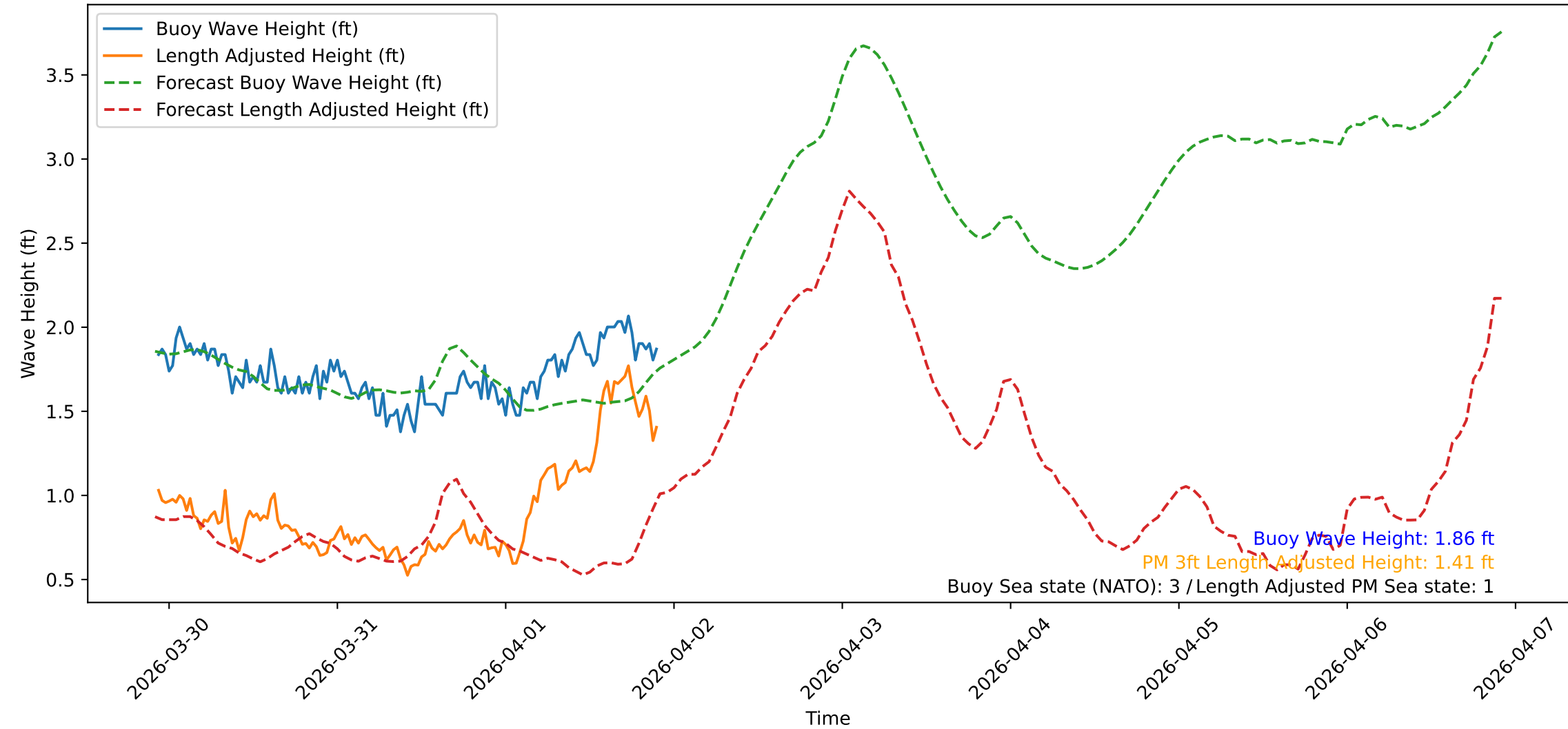
Wave Heights over Time for Red Beach at 2026-04-01 22:20:47
