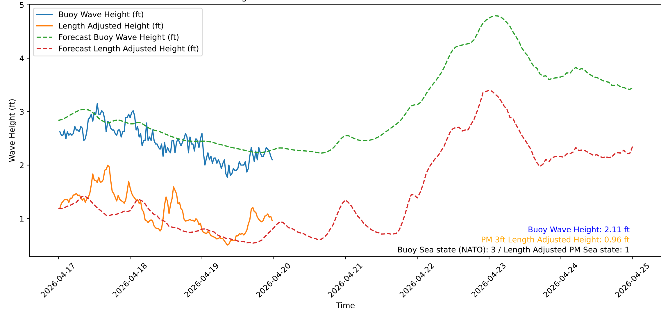
Wave Heights over Time for Red Beach at 2026-04-20 00:20:52
