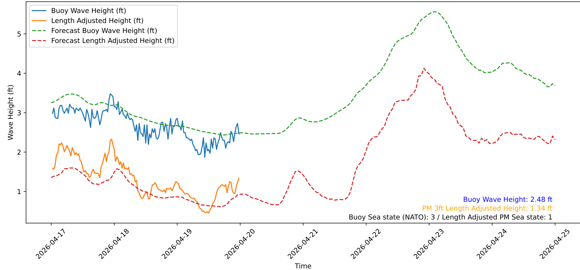
Wave Heights over Time for Green Beach at 2026-04-20 00:21:14
