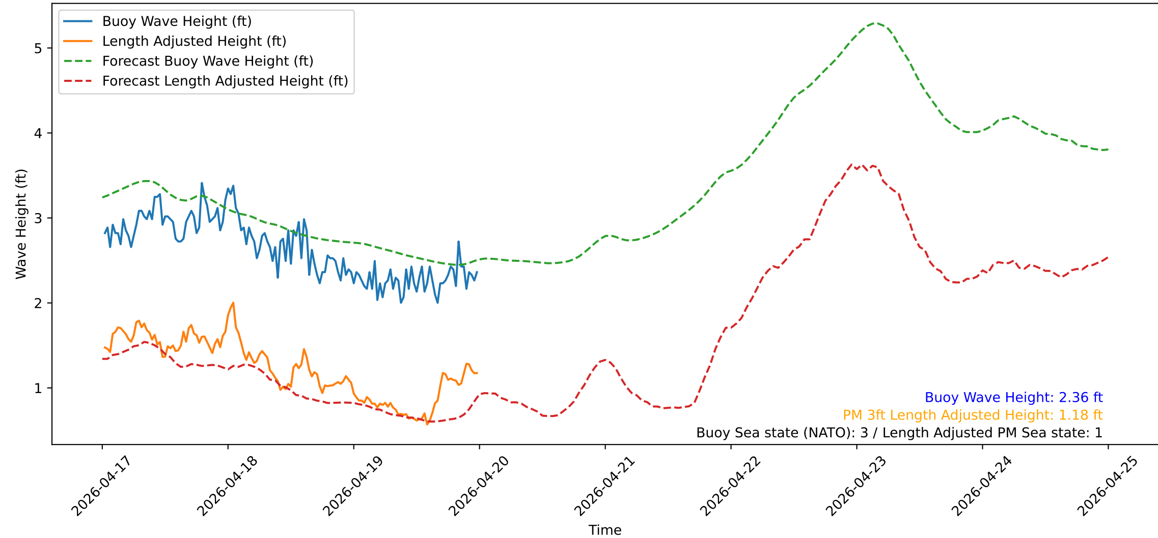
Wave Heights over Time for Oceanside Harbor at 2026-04-20 00:20:32
