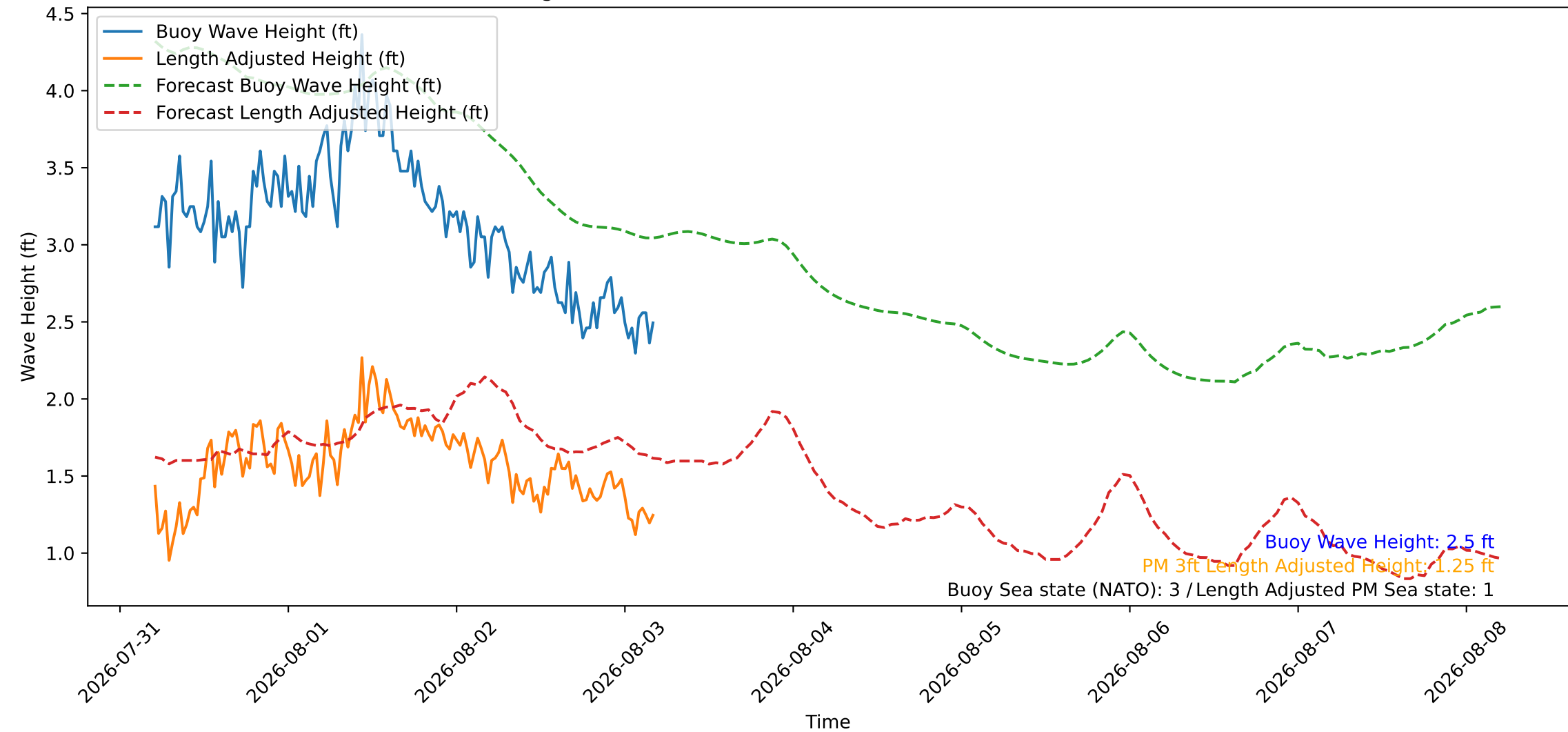
Wave Heights over Time for Oceanside Harbor at 2026-08-03 04:50:26
