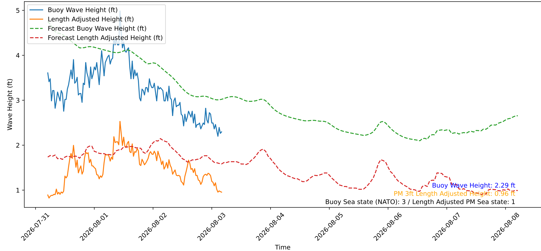
Wave Heights over Time for Green Beach at 2026-08-03 04:51:10
