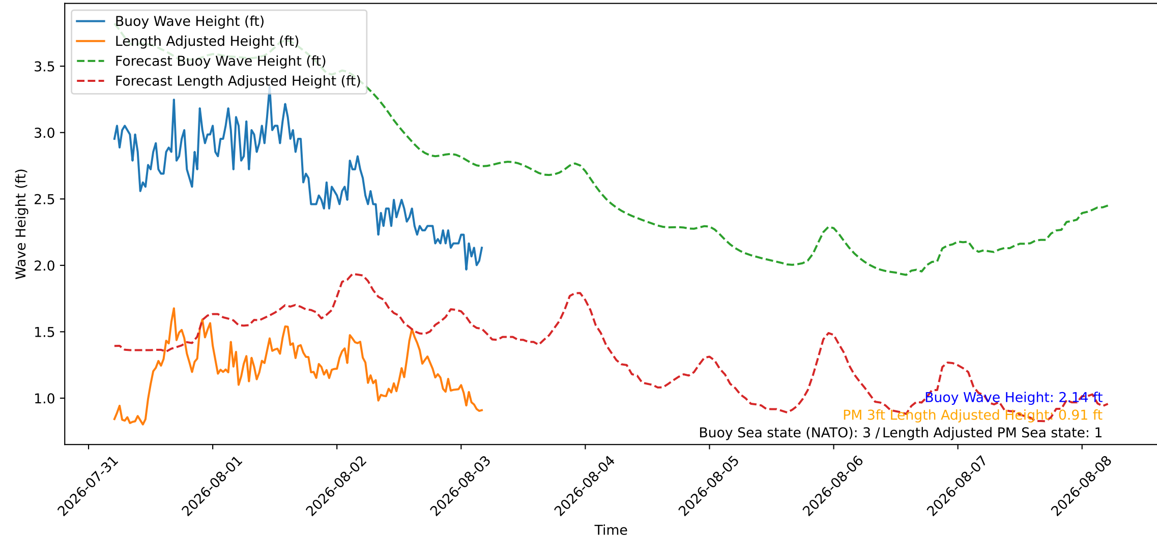
Wave Heights over Time for Red Beach at 2026-08-03 04:50:47
