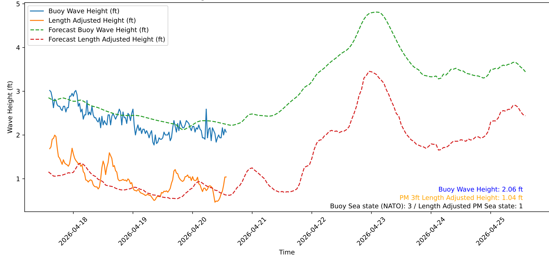
Wave Heights over Time for Red Beach at 2026-04-20 14:10:51
