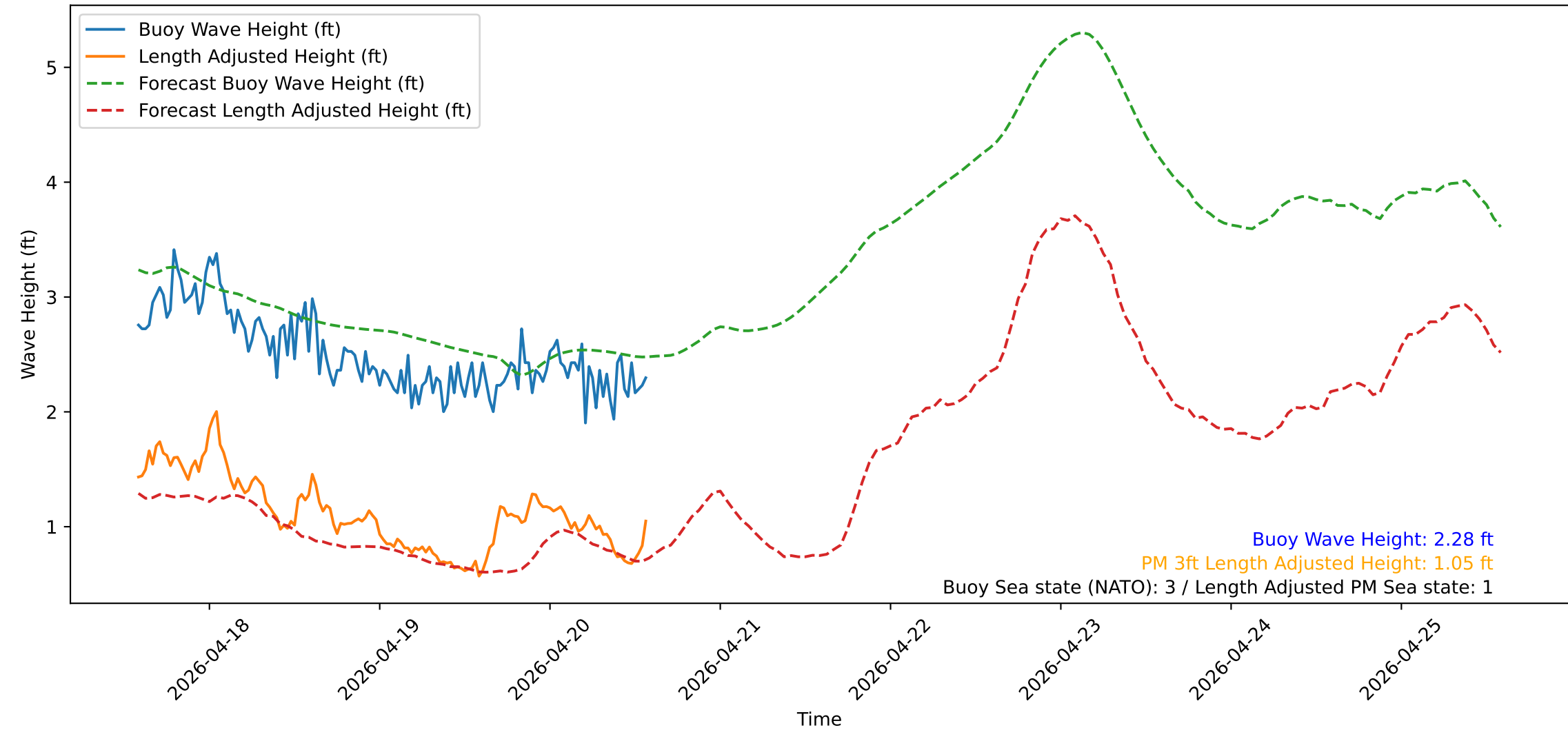
Wave Heights over Time for Oceanside Harbor at 2026-04-20 14:10:31
