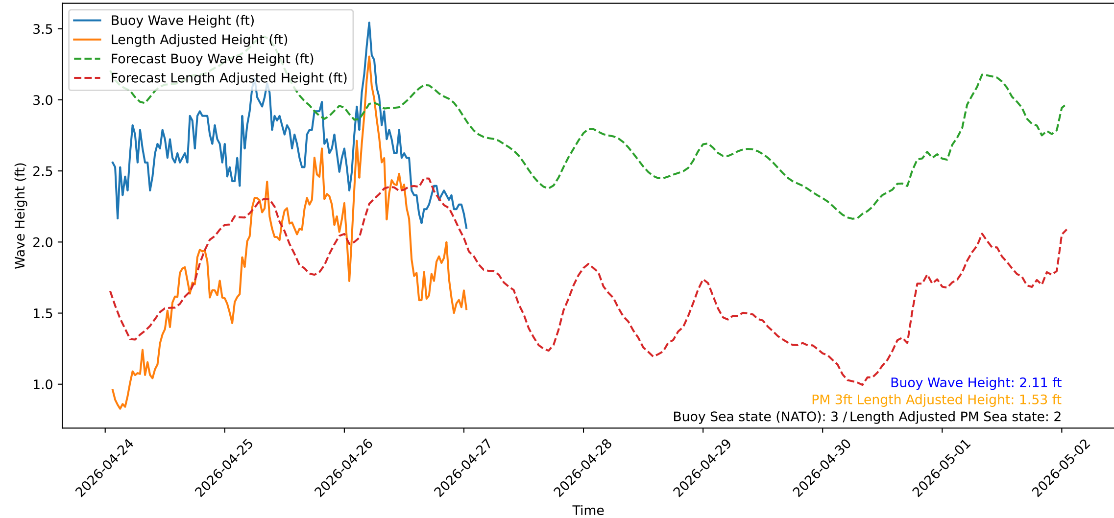
Wave Heights over Time for Red Beach at 2026-04-27 01:20:51
