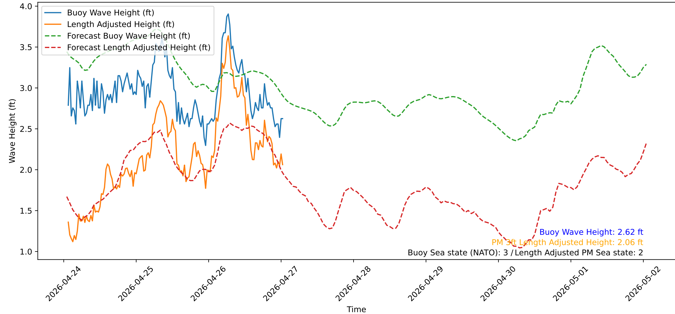
Wave Heights over Time for Oceanside Harbor at 2026-04-27 01:20:31
