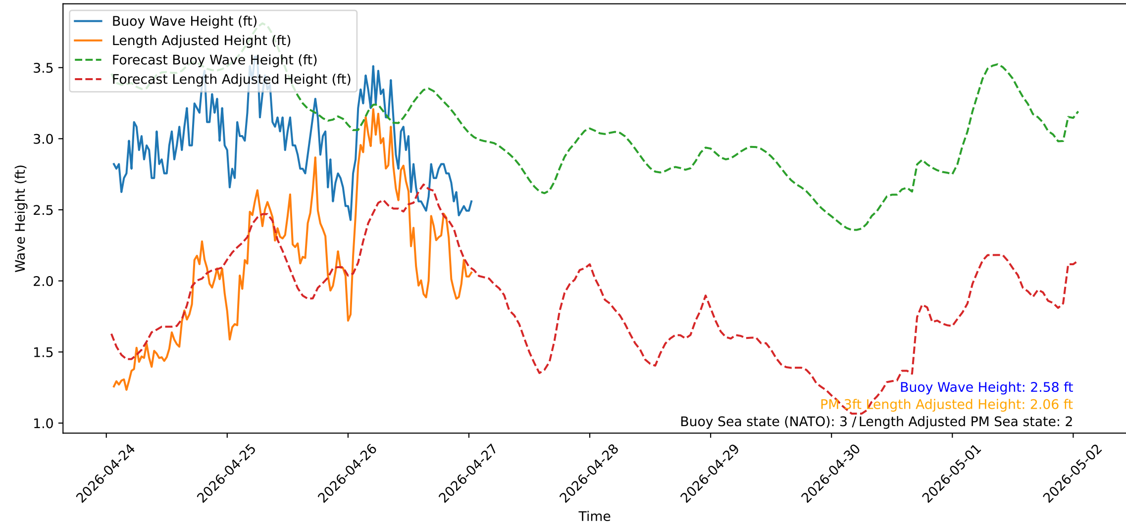
Wave Heights over Time for Green Beach at 2026-04-27 01:21:13
