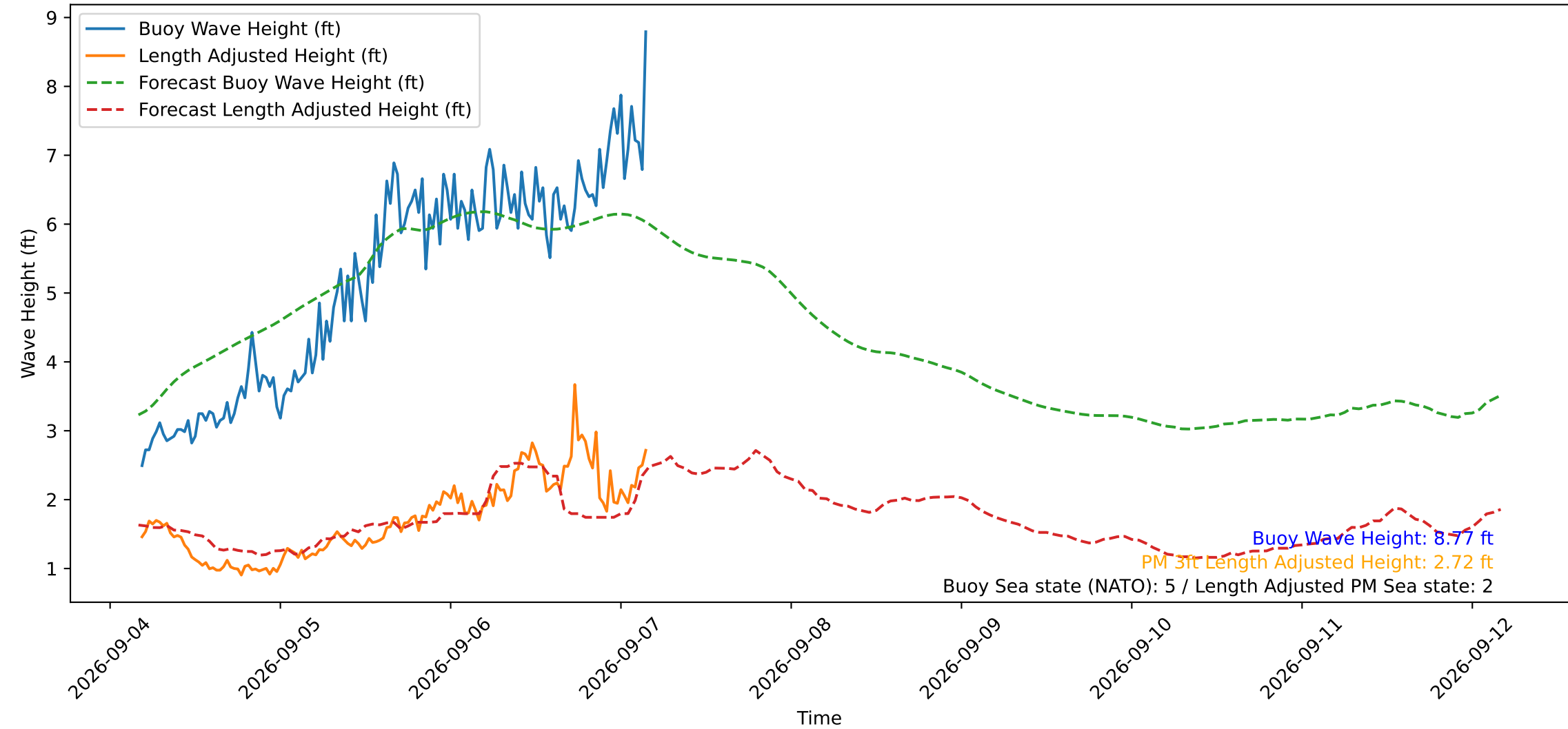
Wave Heights over Time for Green Beach at 2026-09-07 04:11:12
