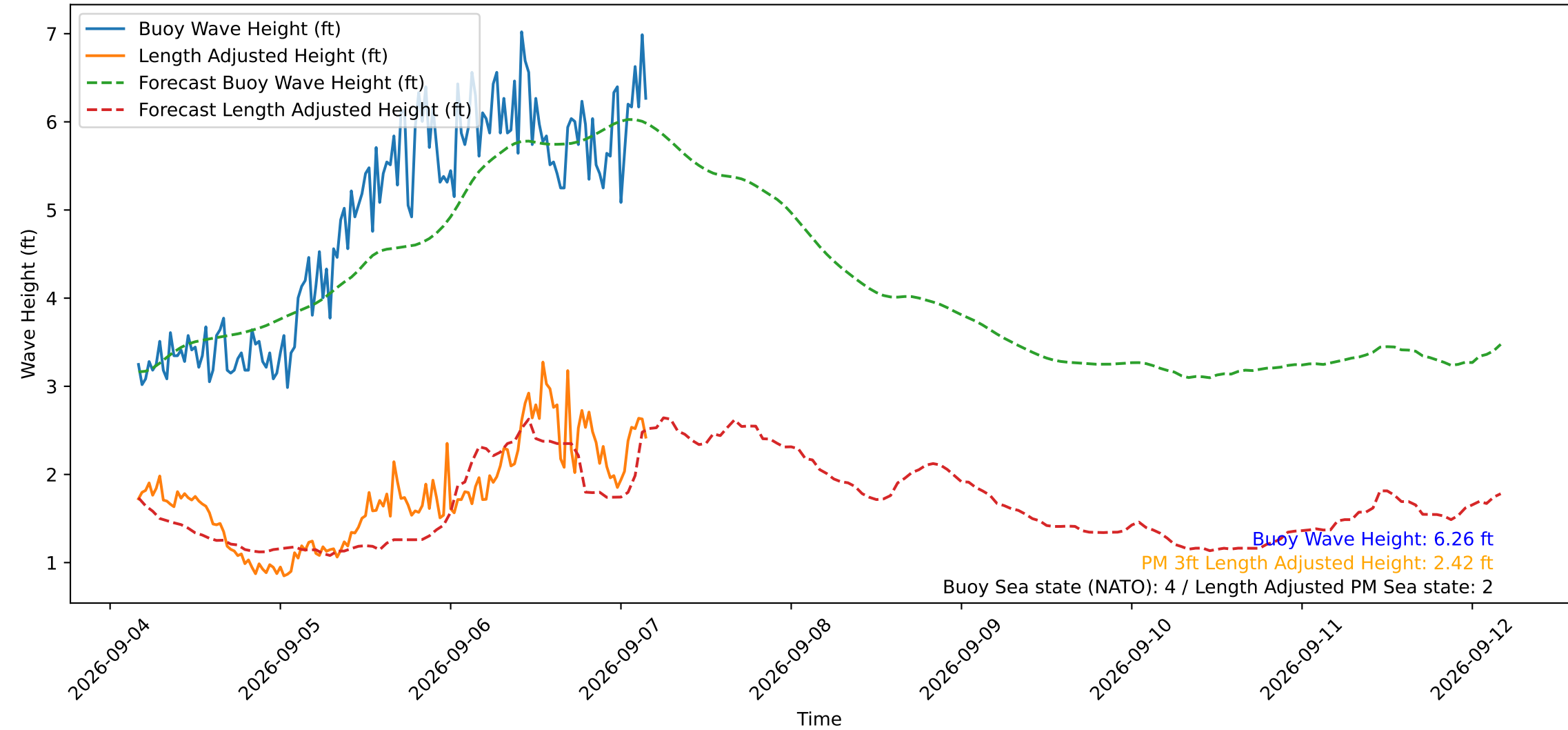
Wave Heights over Time for Oceanside Harbor at 2026-09-07 04:10:30
