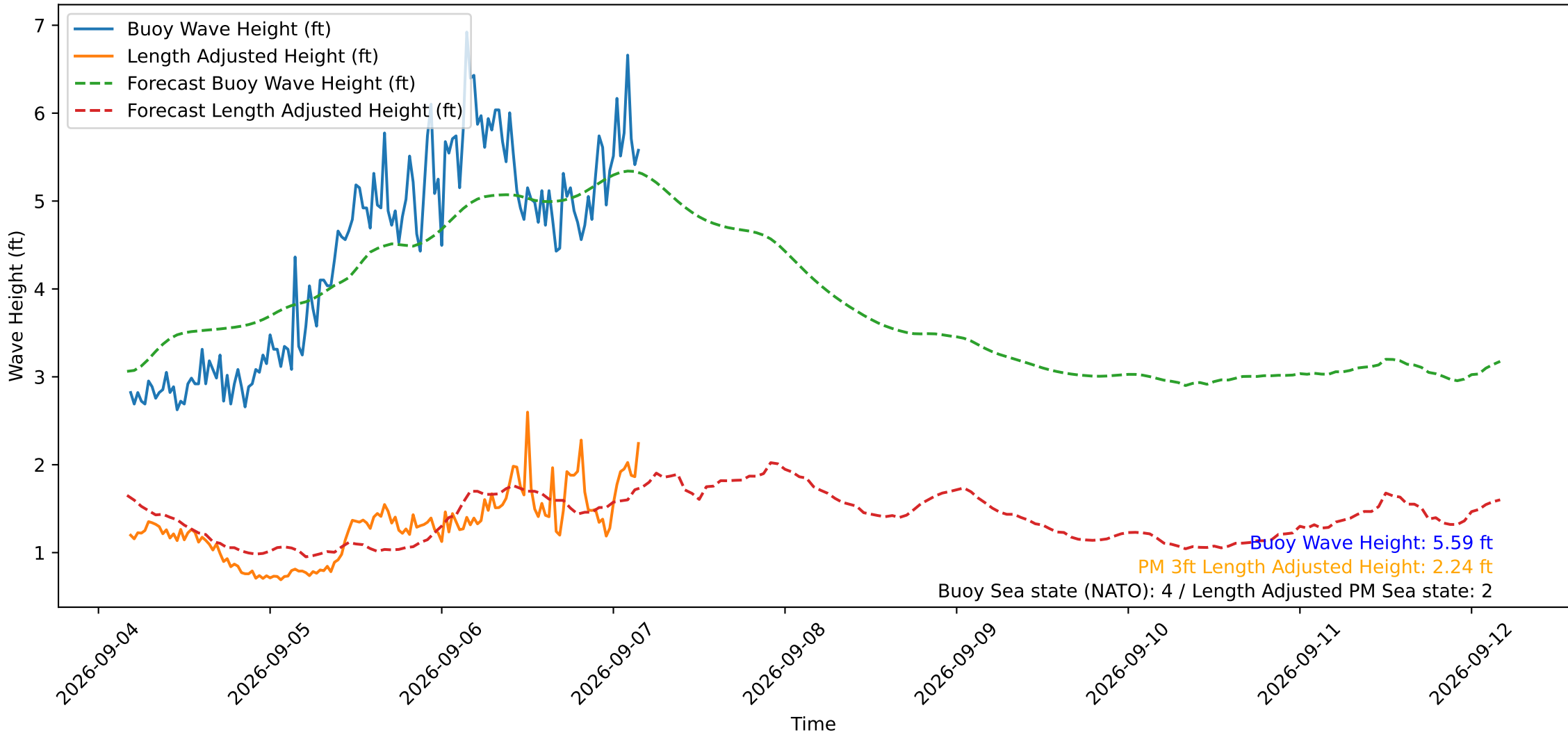
Wave Heights over Time for Red Beach at 2026-09-07 04:10:50
