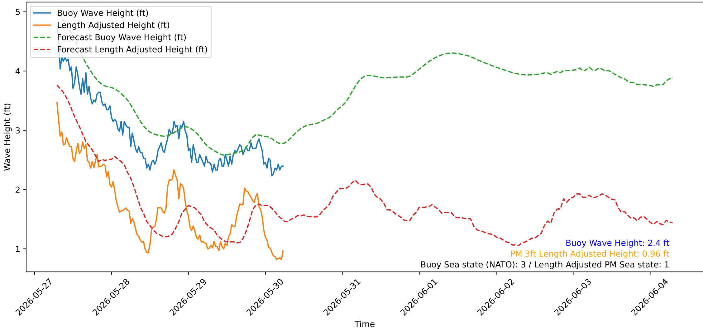
Wave Heights over Time for Red Beach at 2026-05-30 06:30:43
