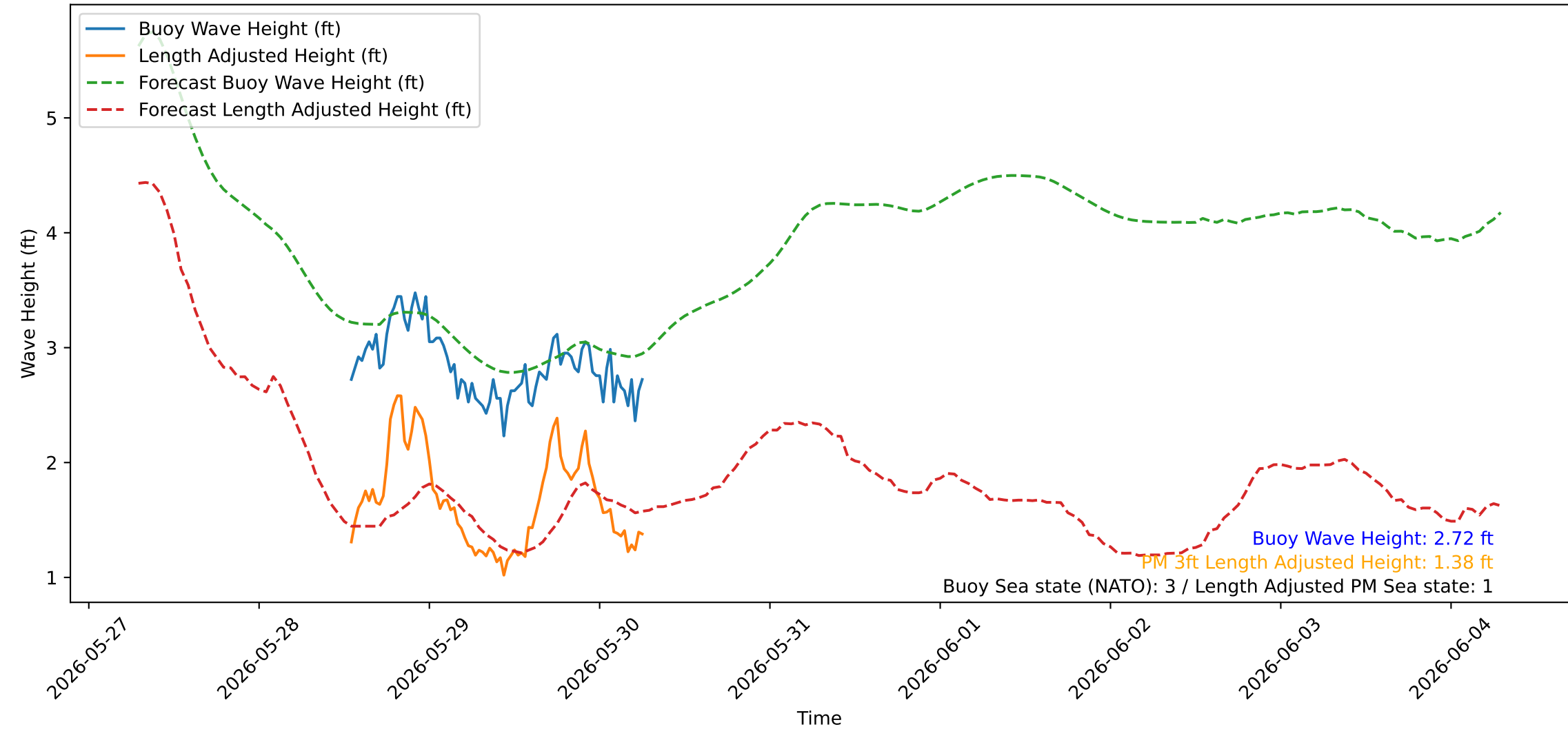
Wave Heights over Time for Oceanside Harbor at 2026-05-30 06:30:24
