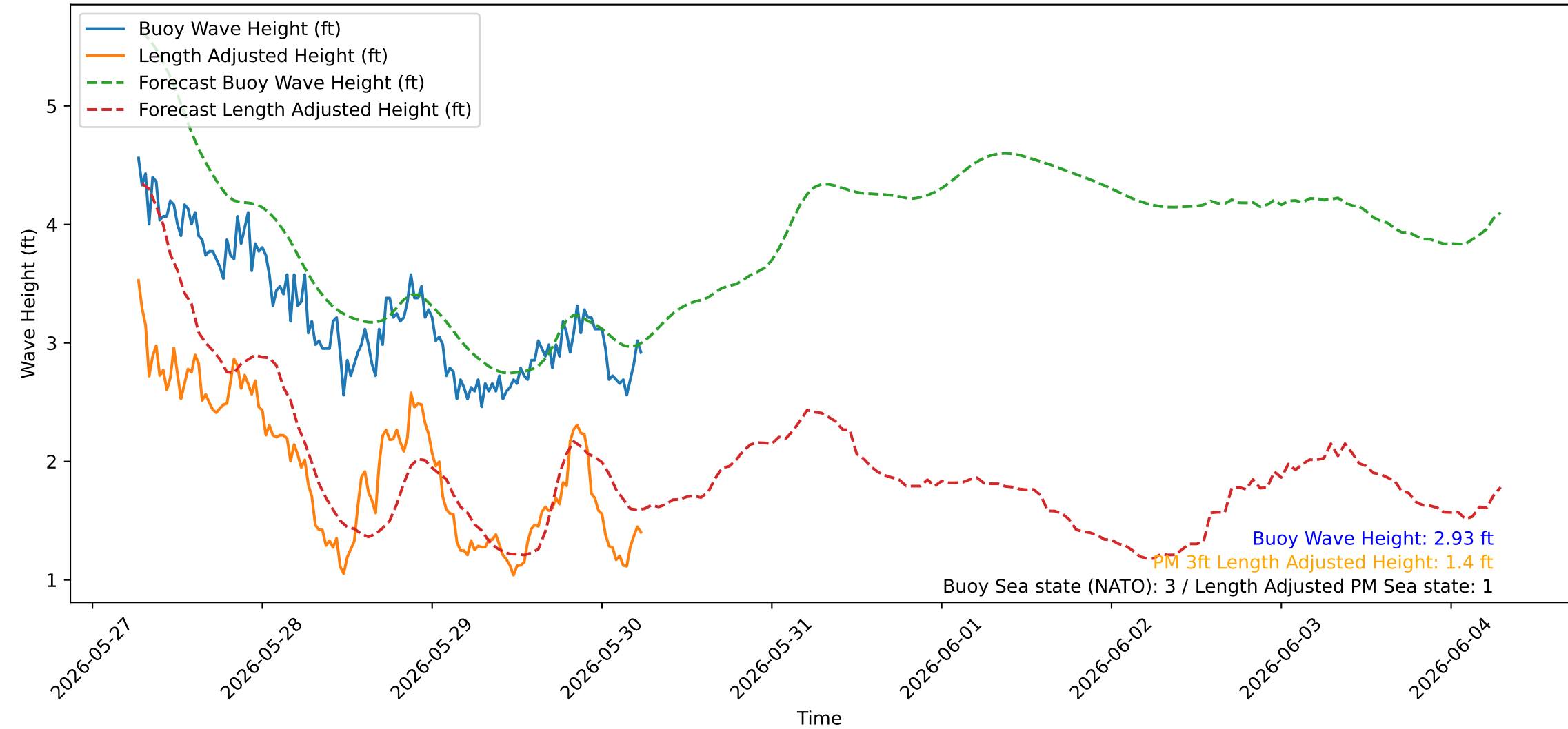
Wave Heights over Time for Green Beach at 2026-05-30 06:31:05
