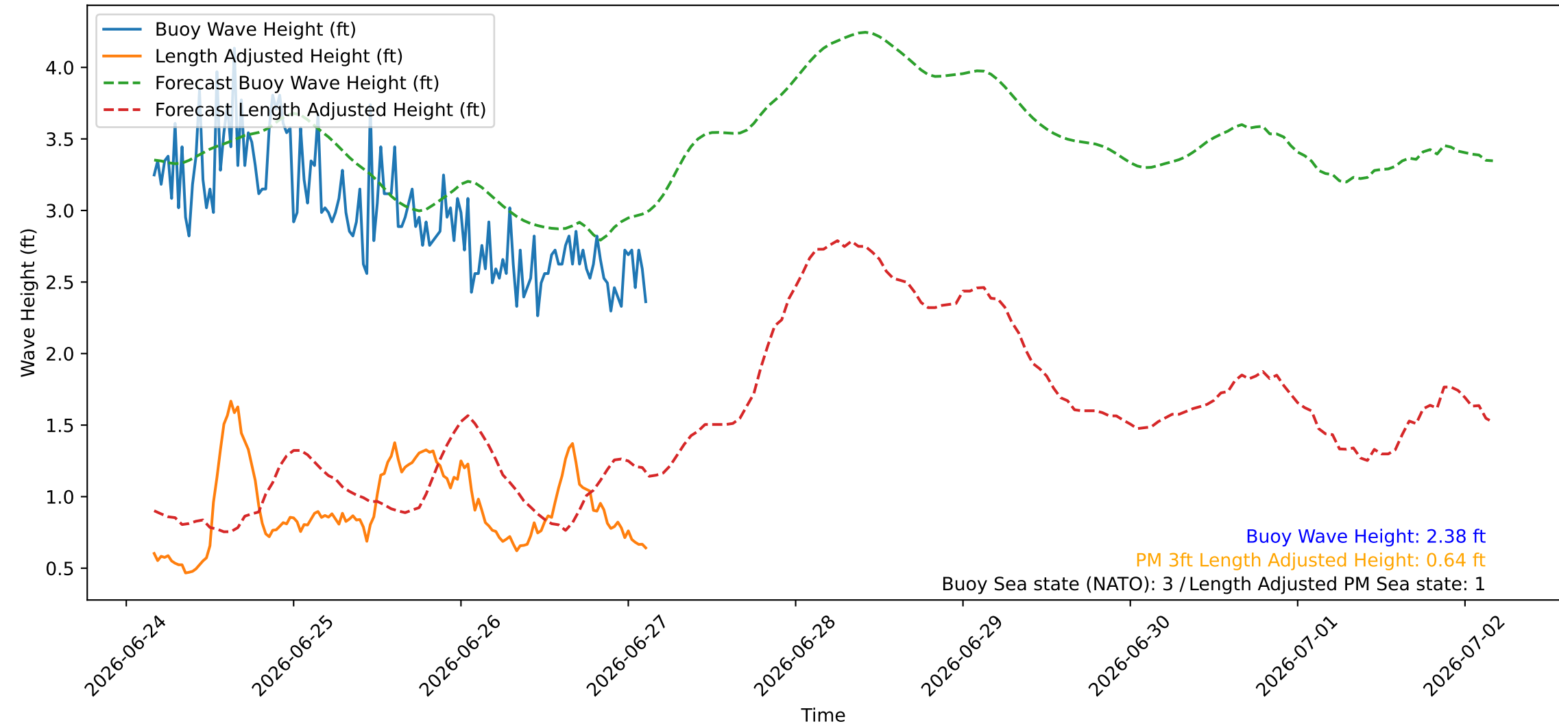
Wave Heights over Time for Red Beach at 2026-06-27 03:30:46
