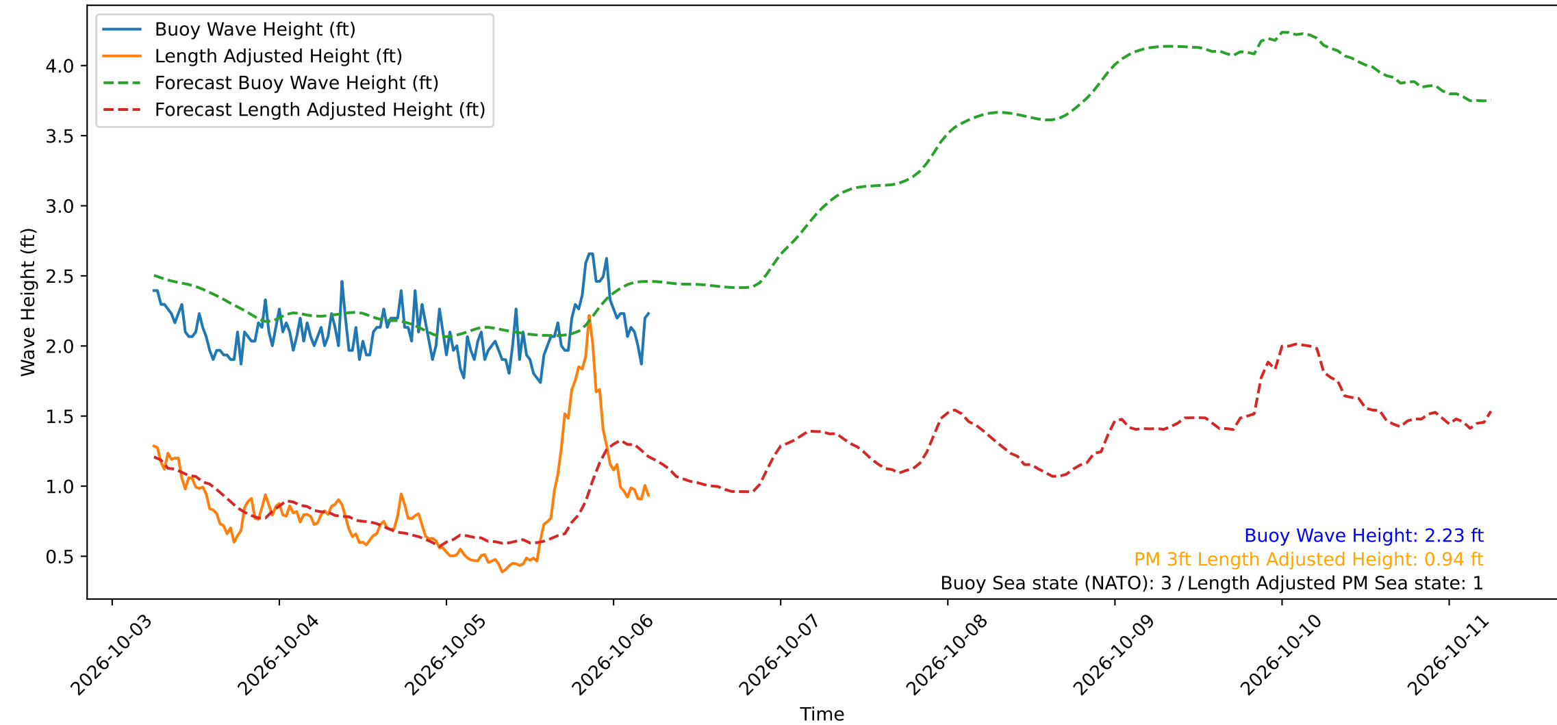
Wave Heights over Time for Red Beach at 2026-10-06 05:40:49
