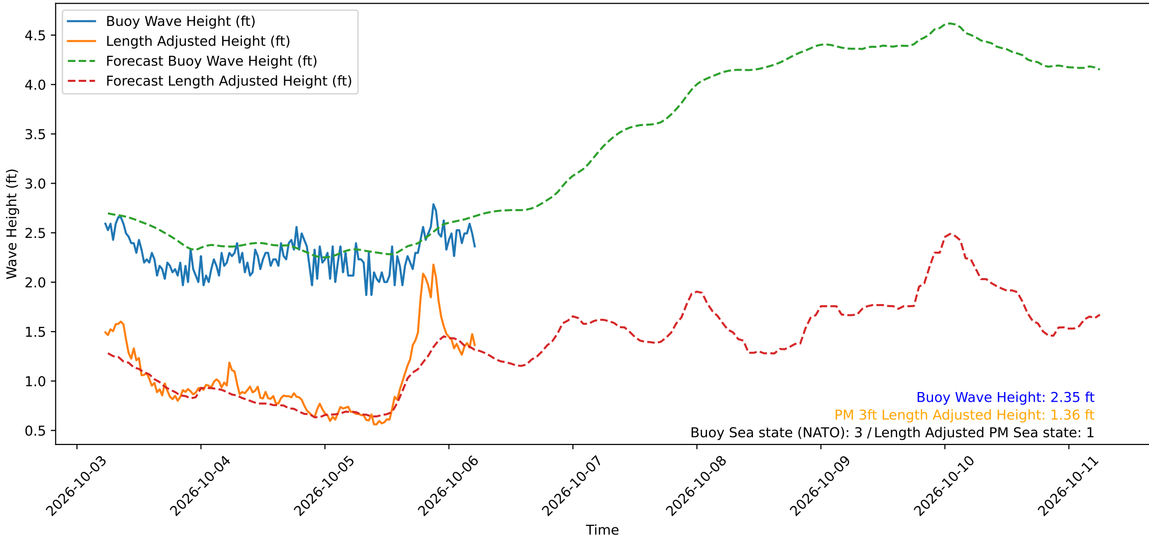
Wave Heights over Time for Oceanside Harbor at 2026-10-06 05:40:30
