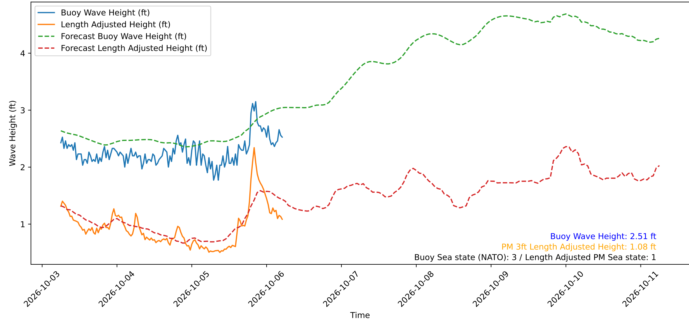
Wave Heights over Time for Green Beach at 2026-10-06 05:41:11
