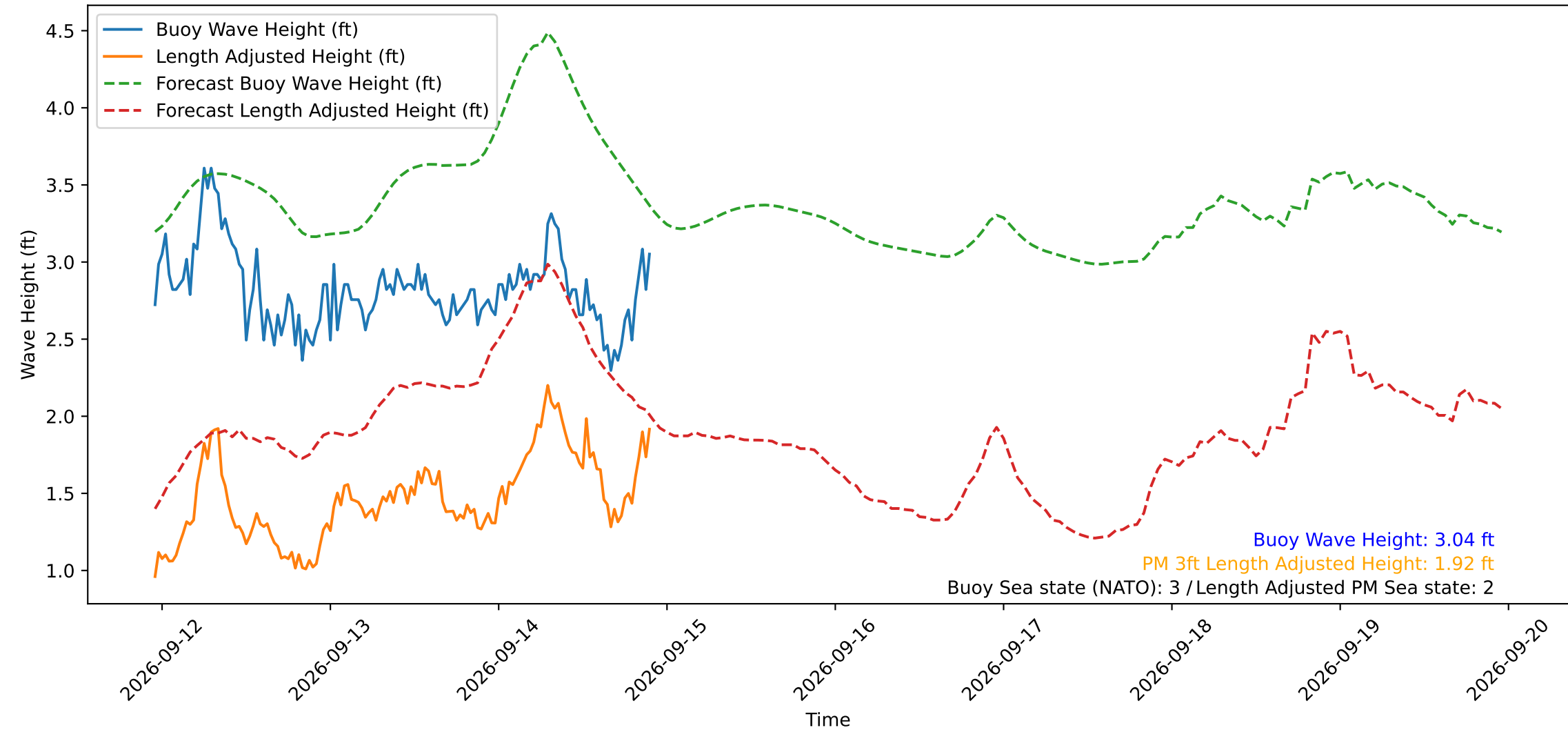
Wave Heights over Time for Green Beach at 2026-09-14 22:31:12
