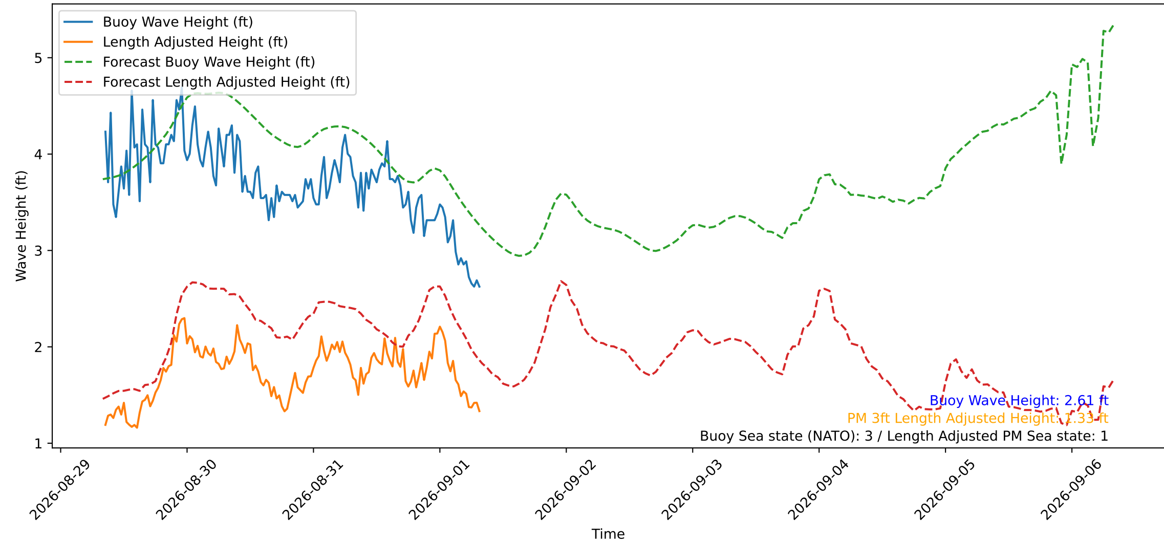
Wave Heights over Time for Red Beach at 2026-09-01 08:10:50
