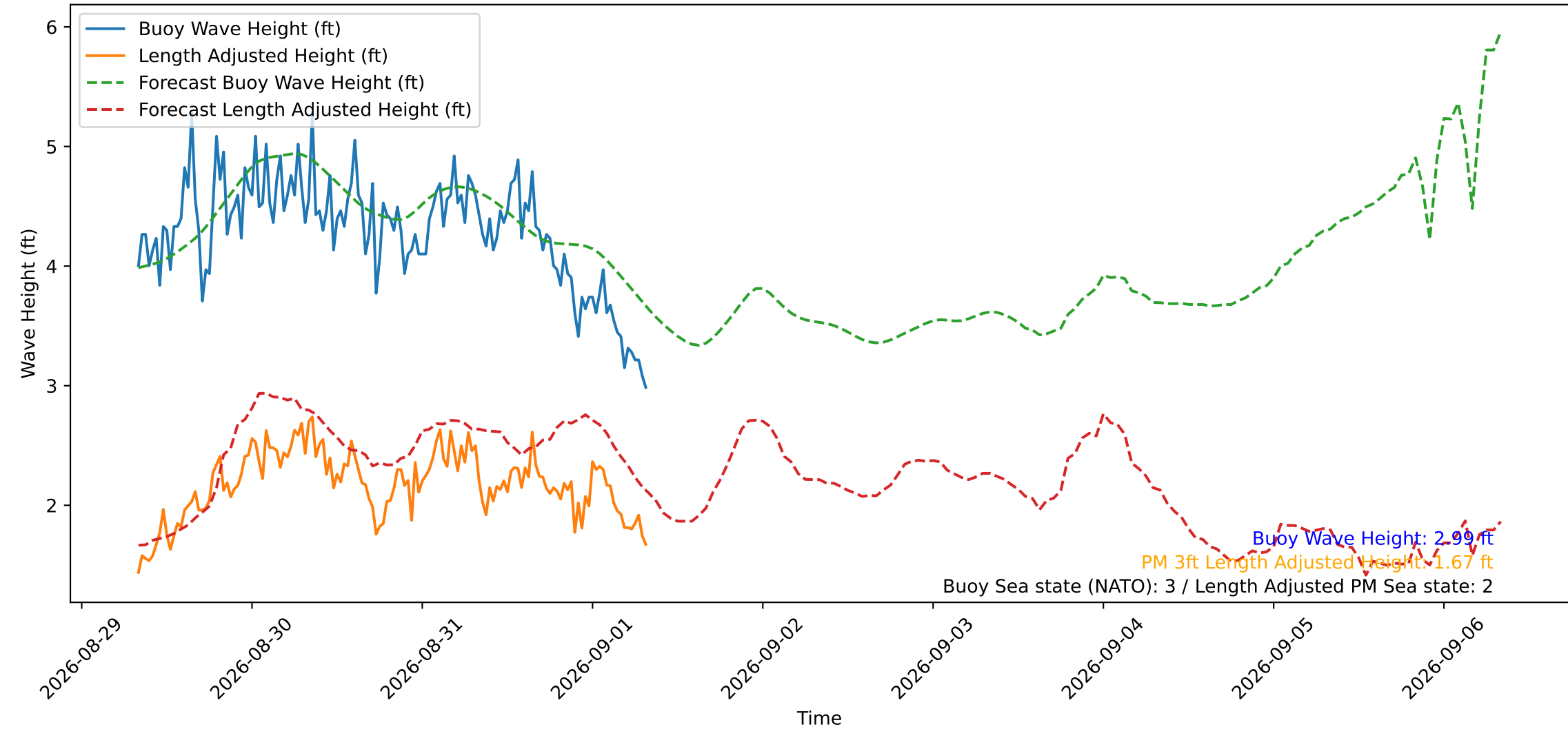
Wave Heights over Time for Oceanside Harbor at 2026-09-01 08:10:30
