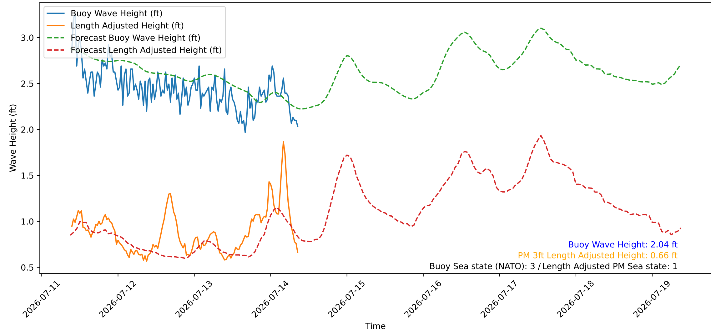
Wave Heights over Time for Red Beach at 2026-07-14 09:20:46
