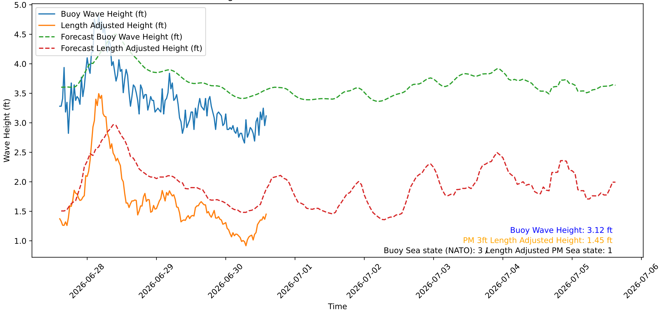
Wave Heights over Time for Green Beach at 2026-06-30 14:41:07
