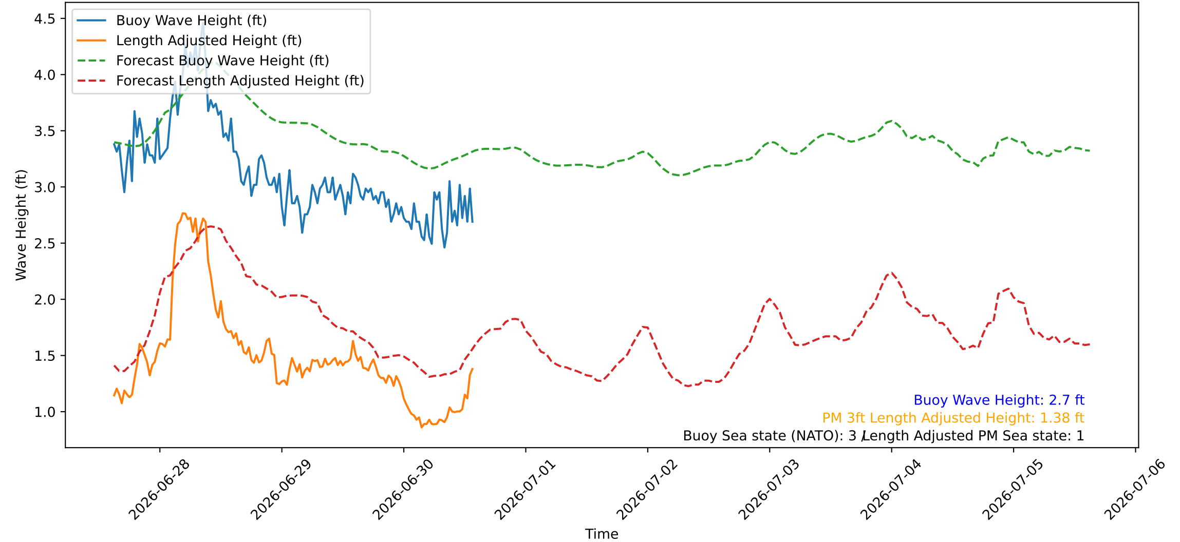
Wave Heights over Time for Red Beach at 2026-06-30 14:40:44
