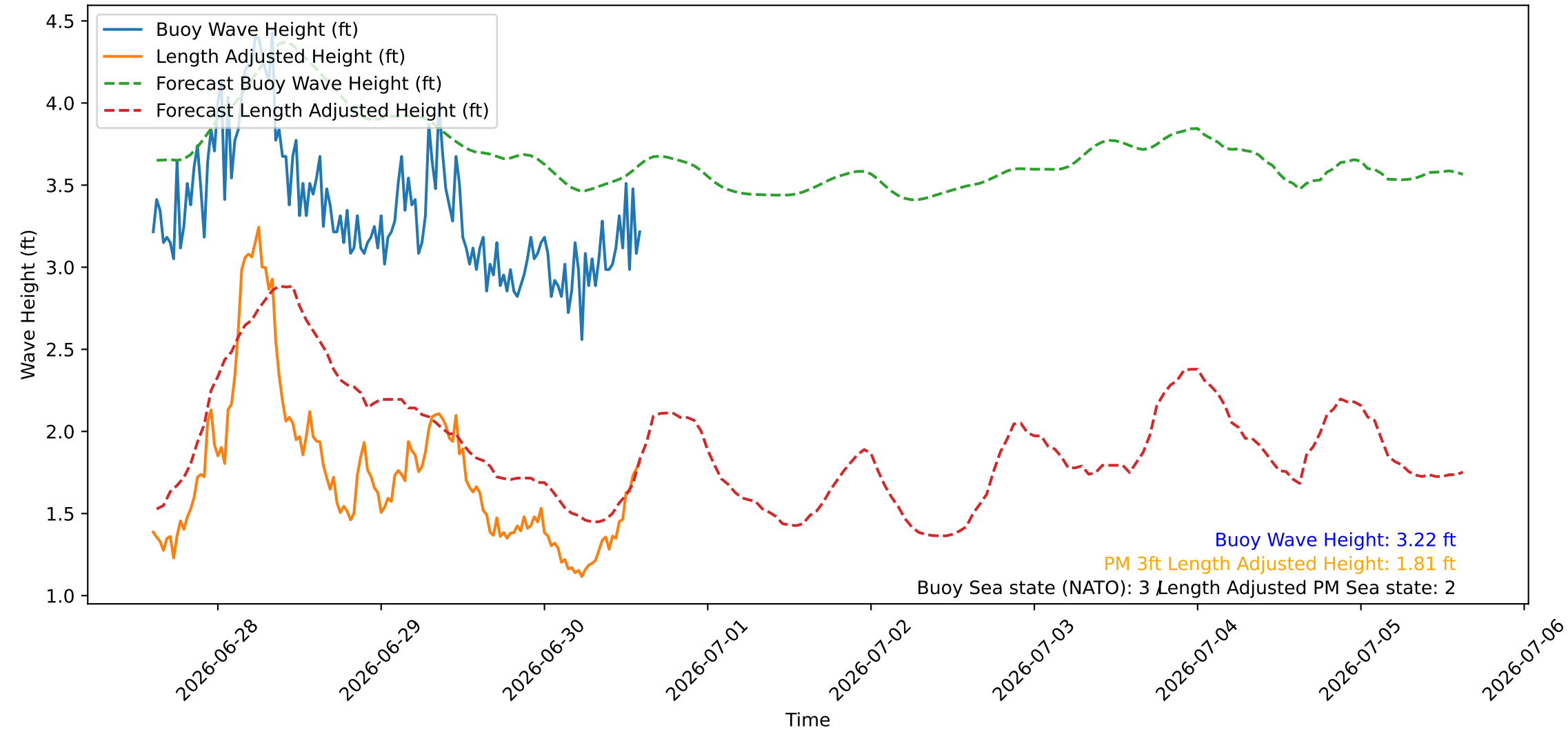
Wave Heights over Time for Oceanside Harbor at 2026-06-30 14:40:25
