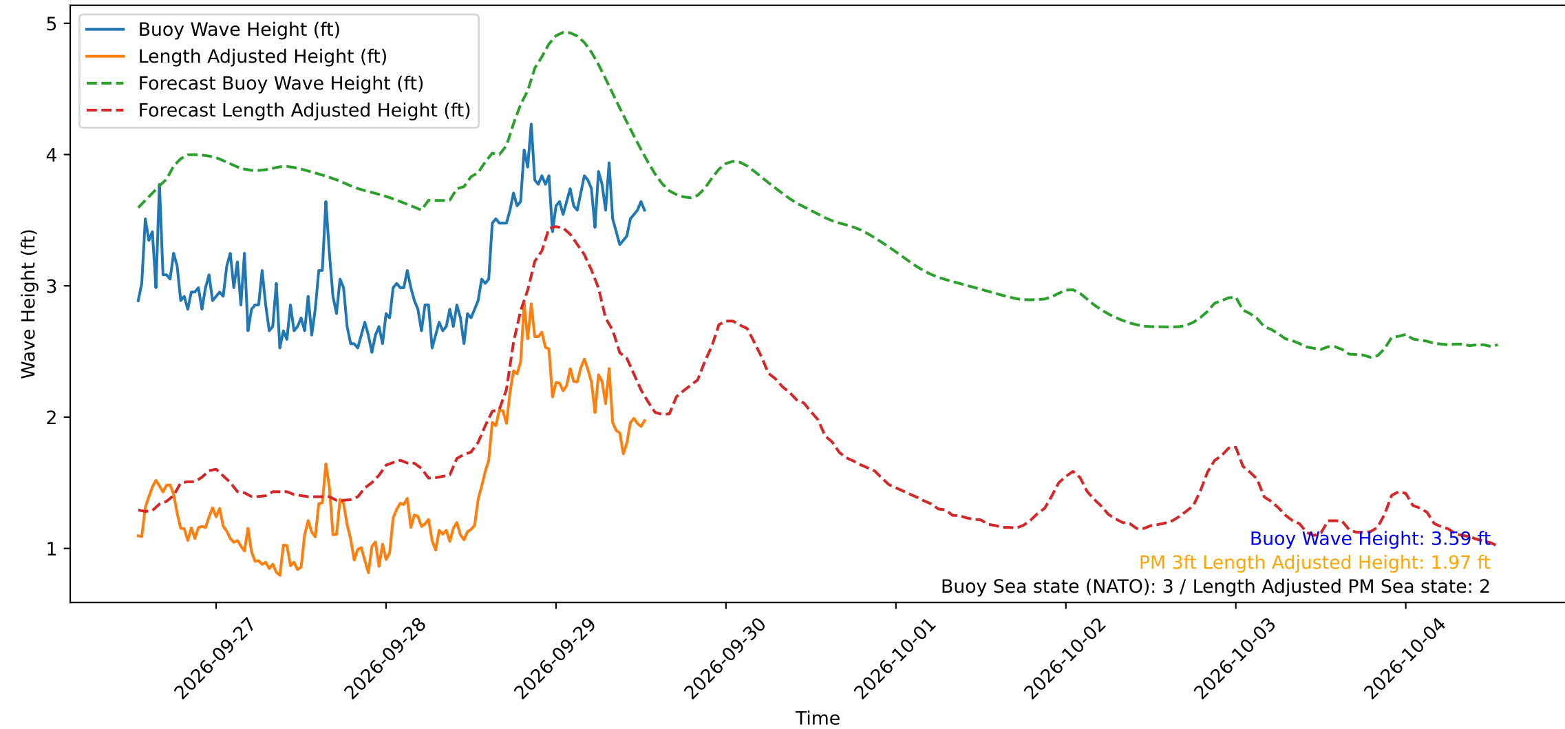
Wave Heights over Time for Oceanside Harbor at 2026-09-29 13:10:30
