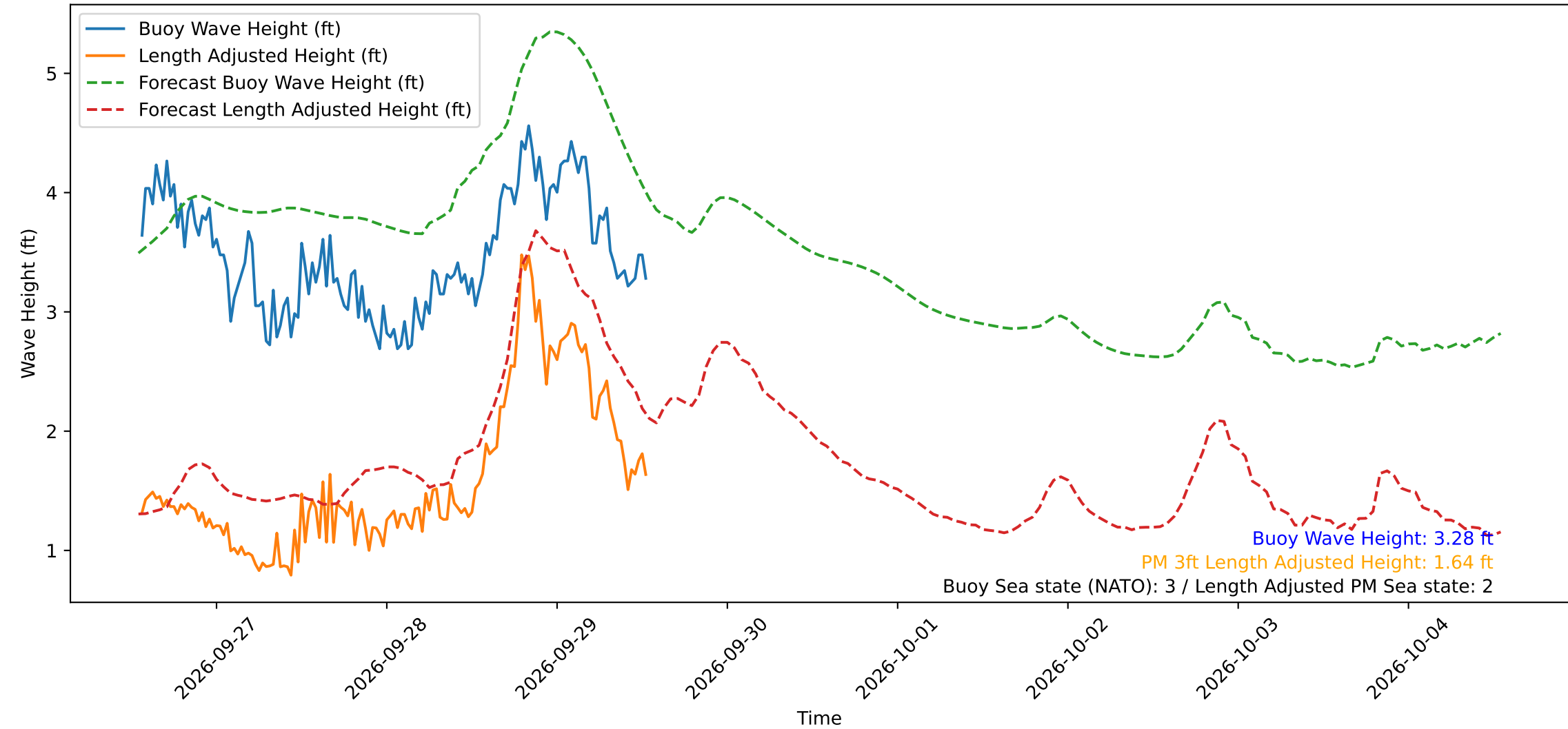
Wave Heights over Time for Green Beach at 2026-09-29 13:11:13
