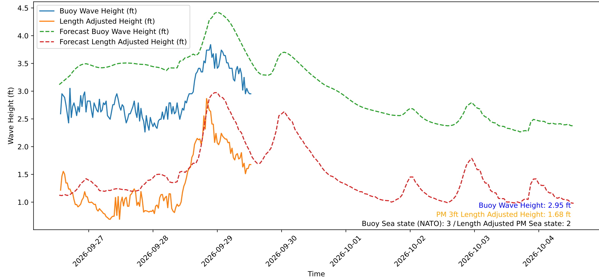
Wave Heights over Time for Red Beach at 2026-09-29 13:10:50
