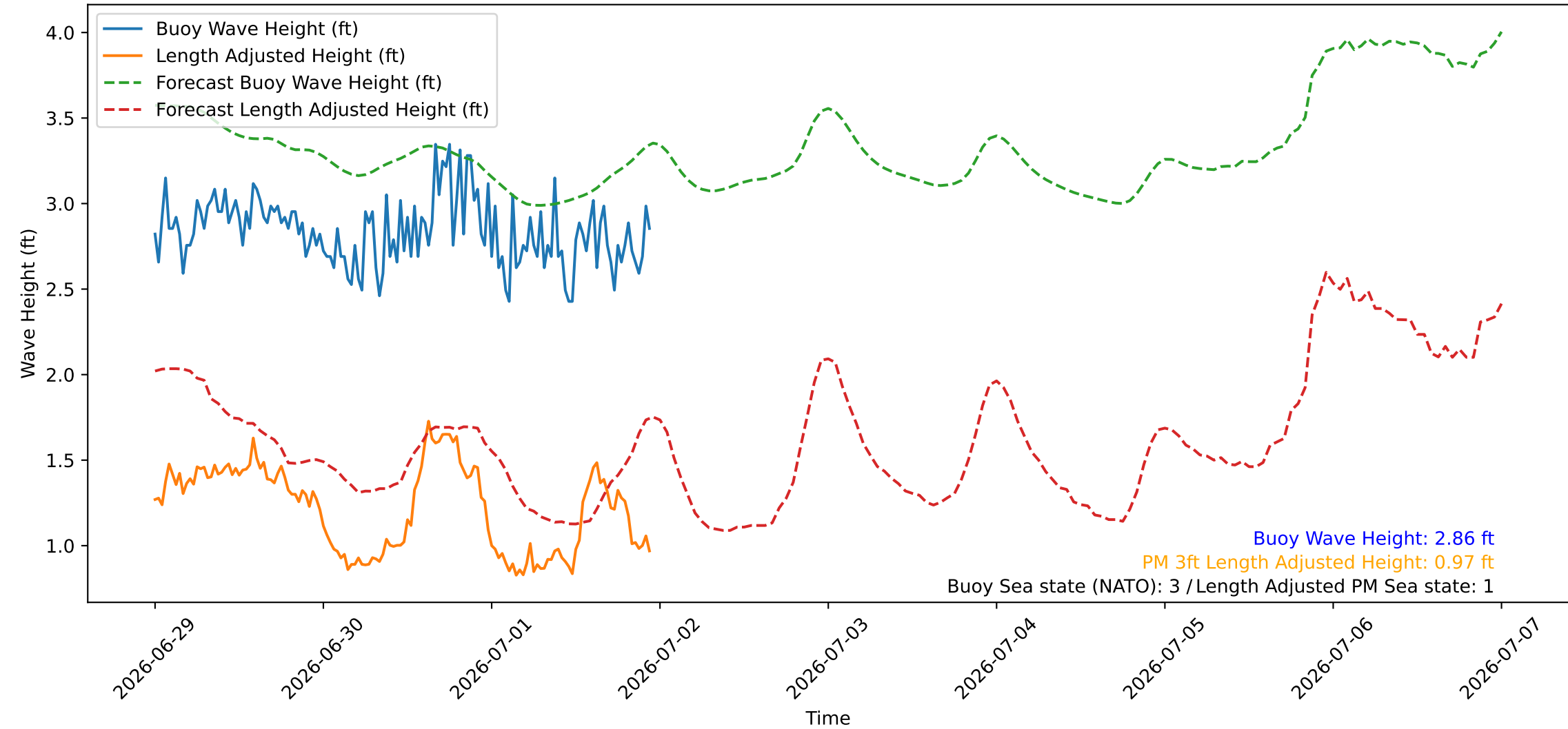
Wave Heights over Time for Red Beach at 2026-07-01 23:30:45
