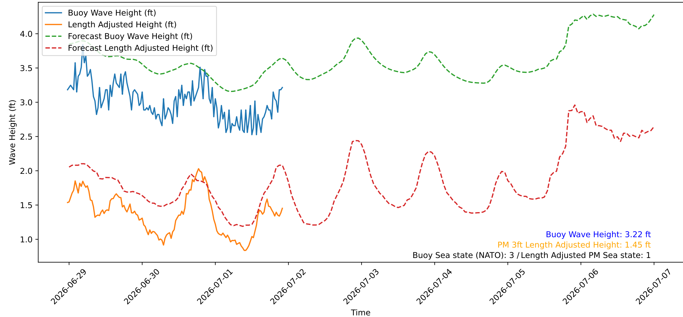
Wave Heights over Time for Green Beach at 2026-07-01 23:31:07
