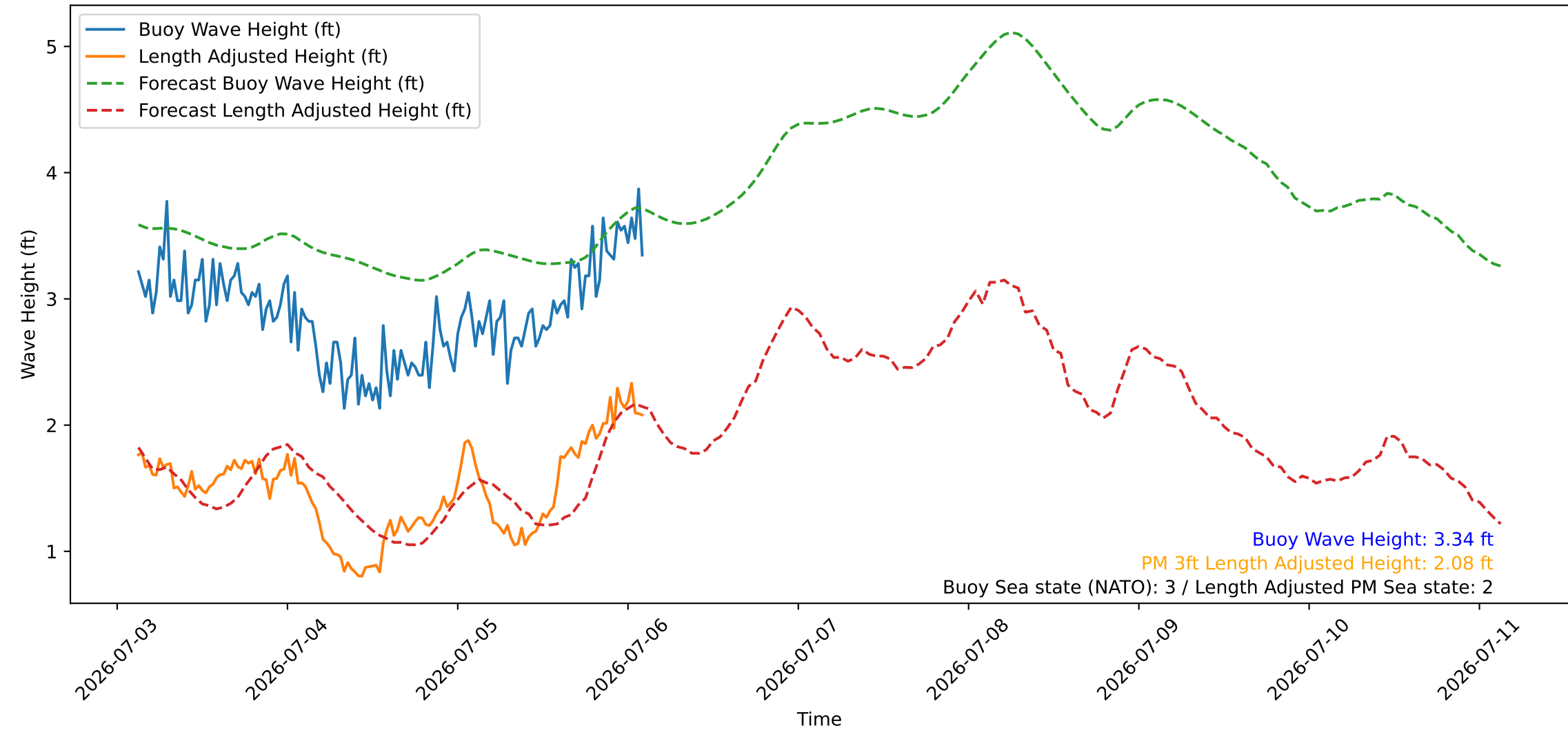
Wave Heights over Time for Oceanside Harbor at 2026-07-06 03:00:27
