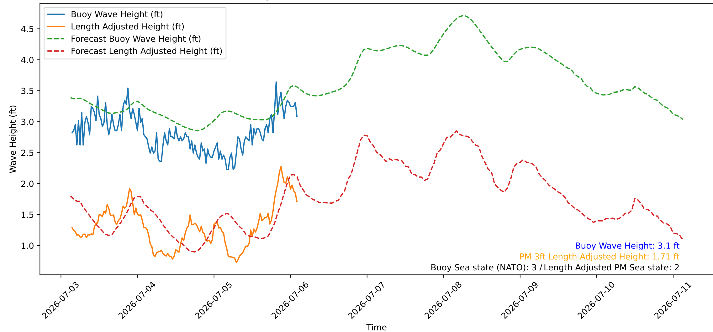
Wave Heights over Time for Red Beach at 2026-07-06 03:00:46
