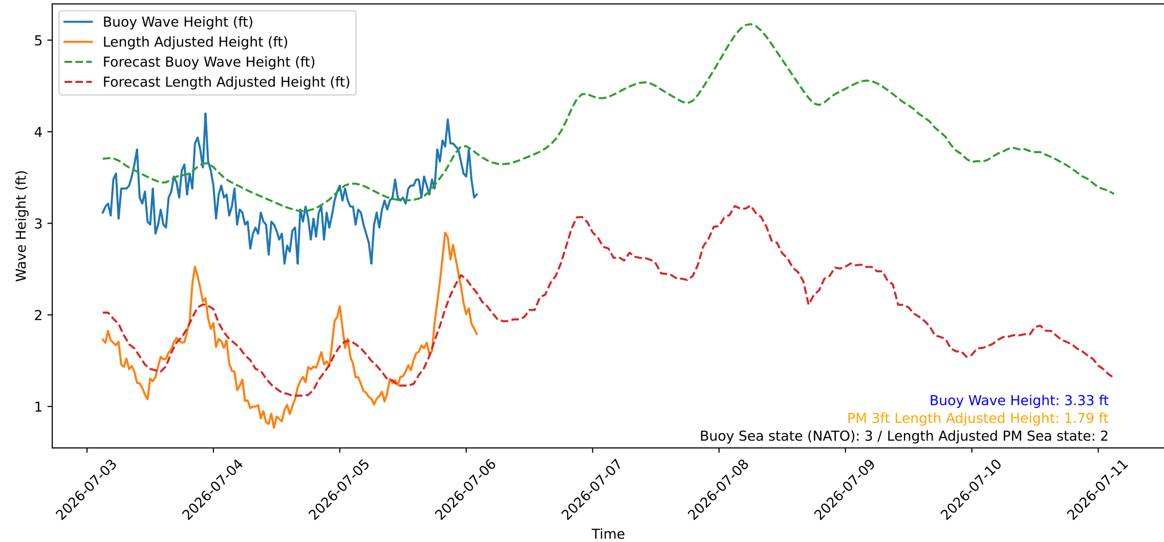
Wave Heights over Time for Green Beach at 2026-07-06 03:01:09
