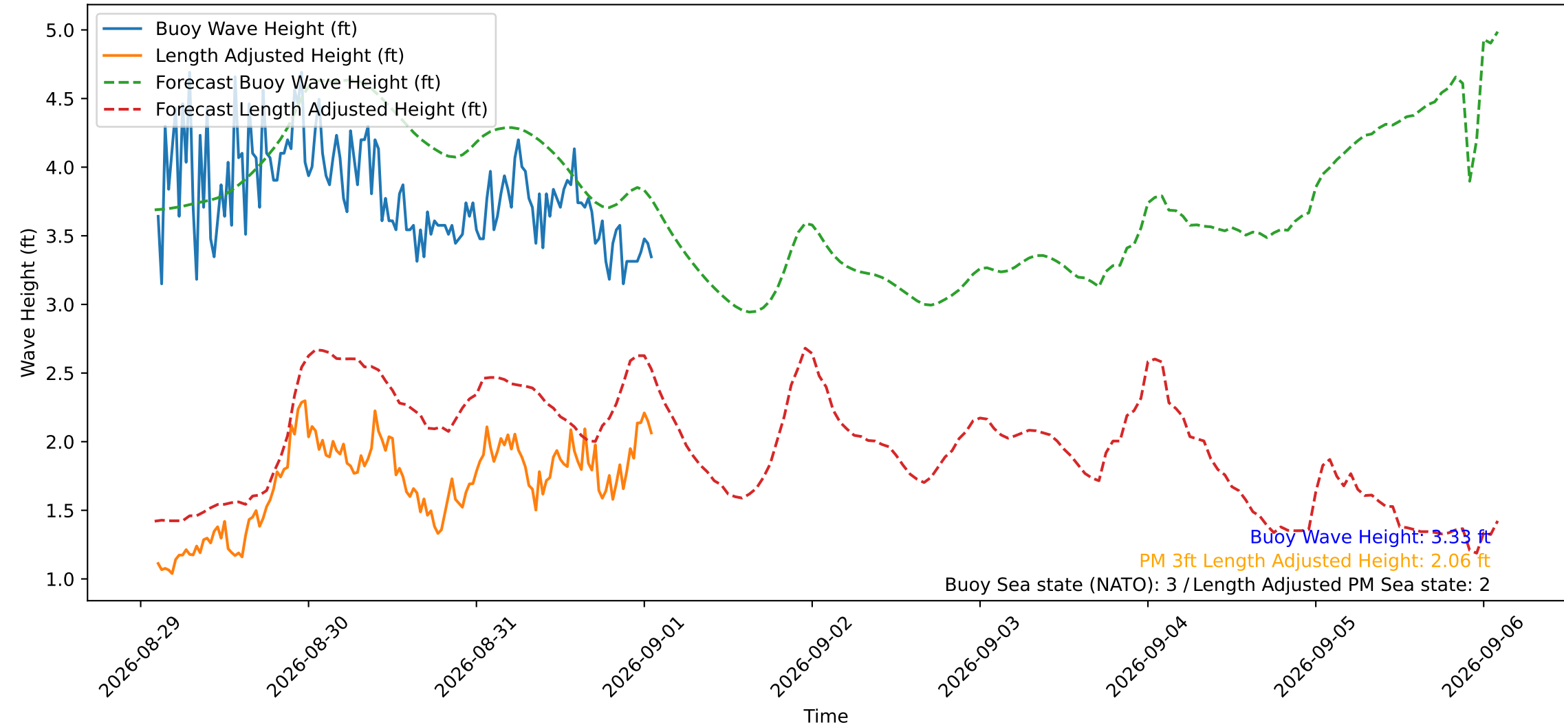
Wave Heights over Time for Red Beach at 2026-09-01 02:00:49
