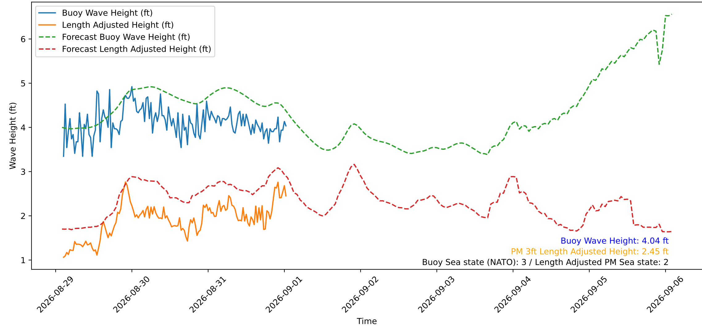
Wave Heights over Time for Green Beach at 2026-09-01 02:01:11
