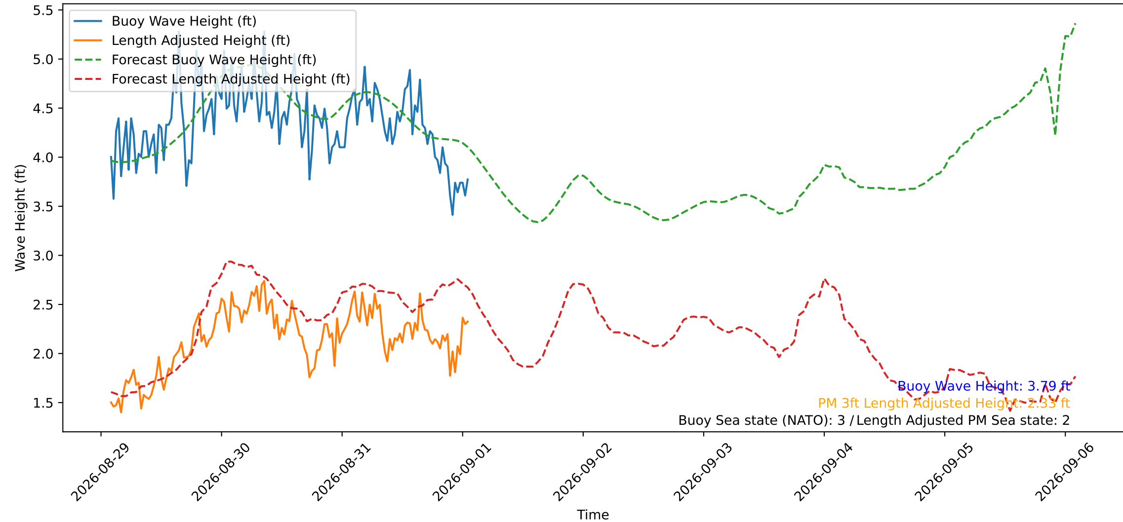
Wave Heights over Time for Oceanside Harbor at 2026-09-01 02:00:30
