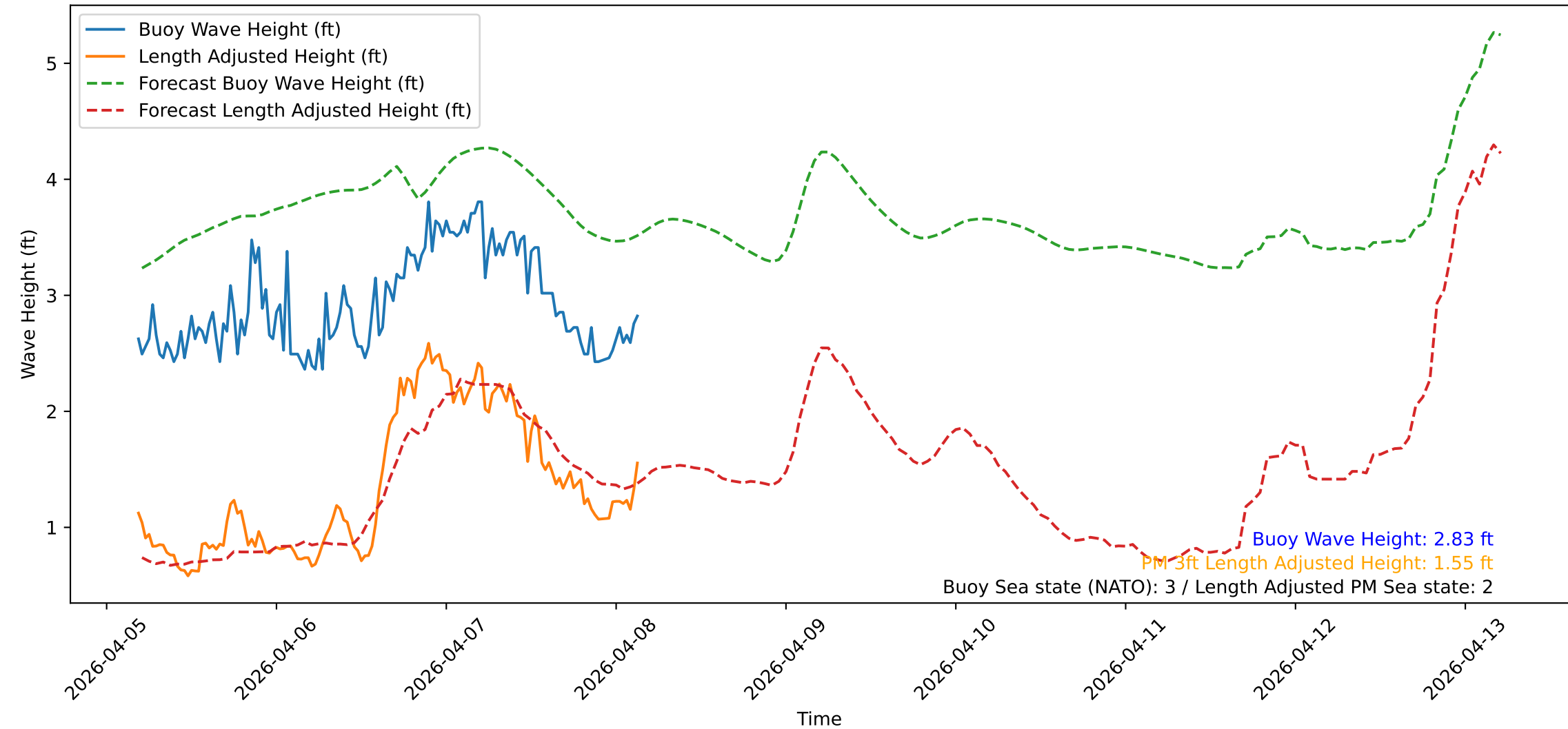
Wave Heights over Time for Green Beach at 2026-04-08 04:31:09
