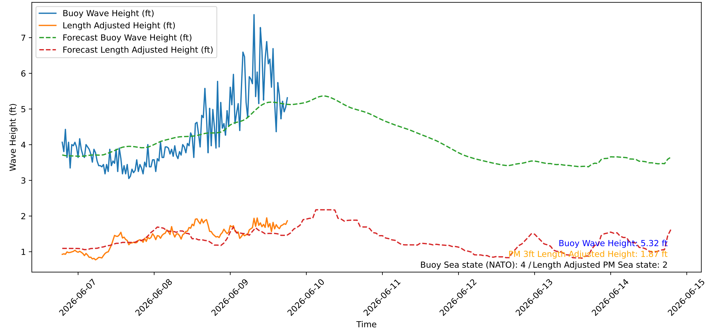
Wave Heights over Time for Red Beach at 2026-06-09 18:50:48
