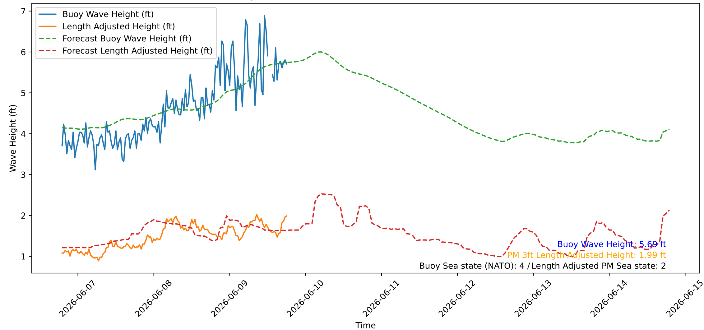
Wave Heights over Time for Green Beach at 2026-06-09 18:51:12
