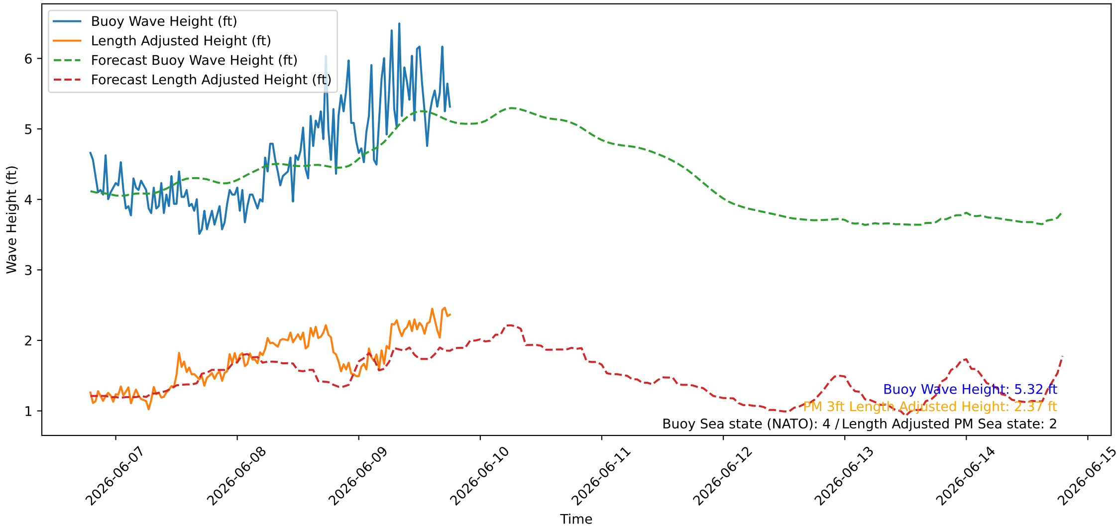
Wave Heights over Time for Oceanside Harbor at 2026-06-09 18:50:27
