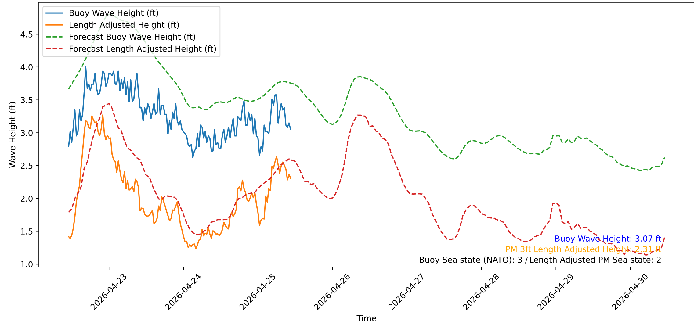
Wave Heights over Time for Green Beach at 2026-04-25 11:11:13
