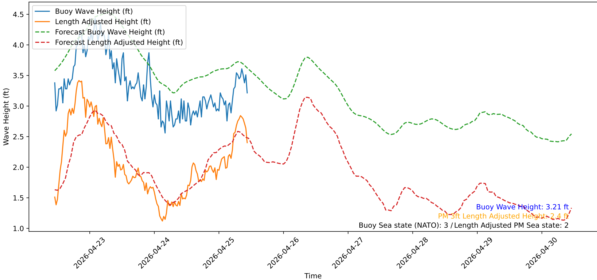
Wave Heights over Time for Oceanside Harbor at 2026-04-25 11:10:32
