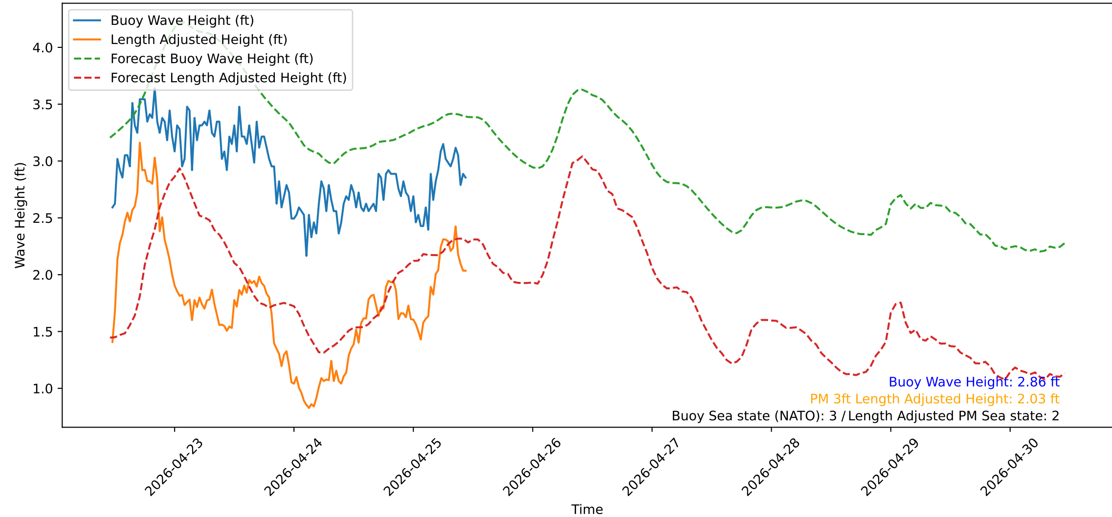
Wave Heights over Time for Red Beach at 2026-04-25 11:10:51
