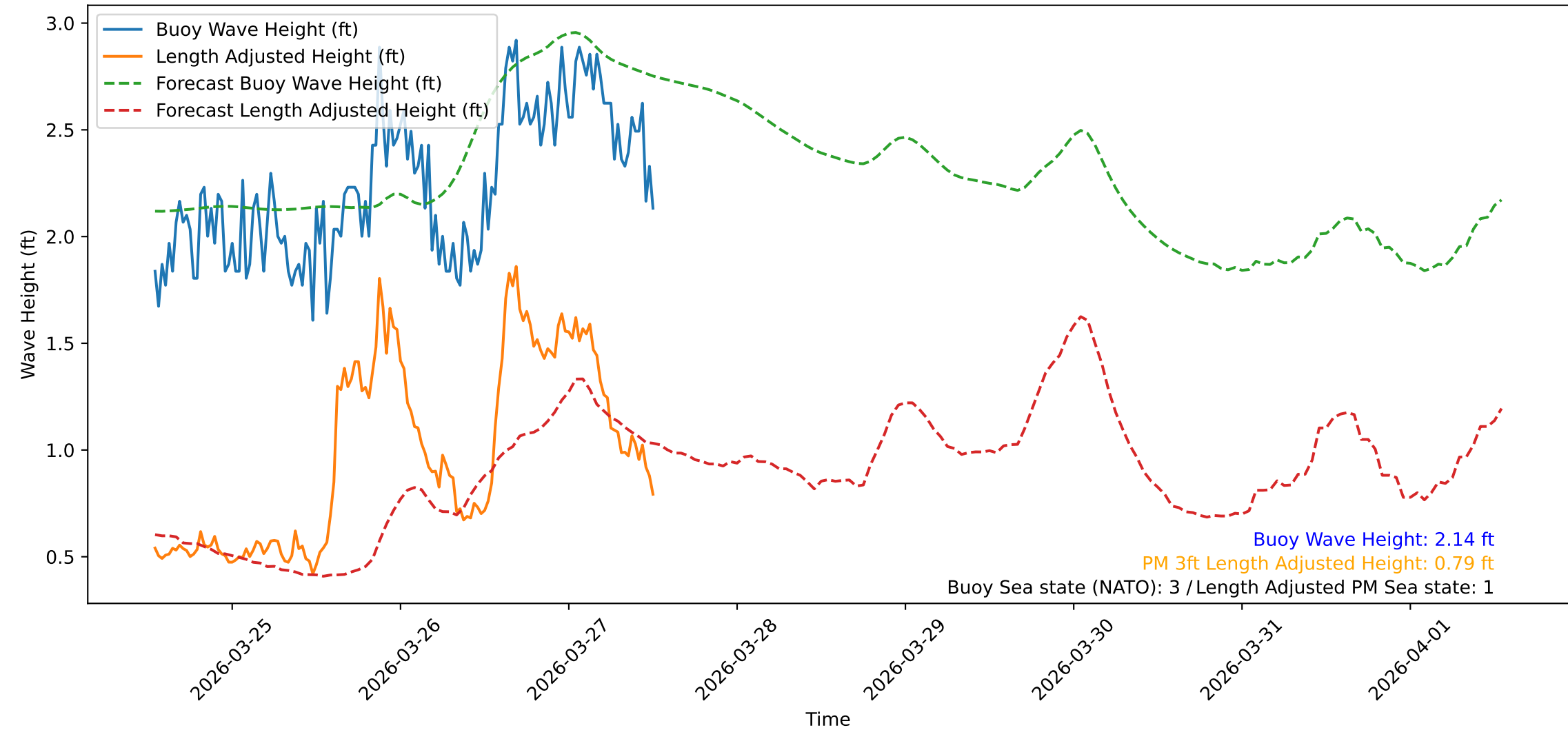
Wave Heights over Time for Oceanside Harbor at 2026-03-27 13:00:31
