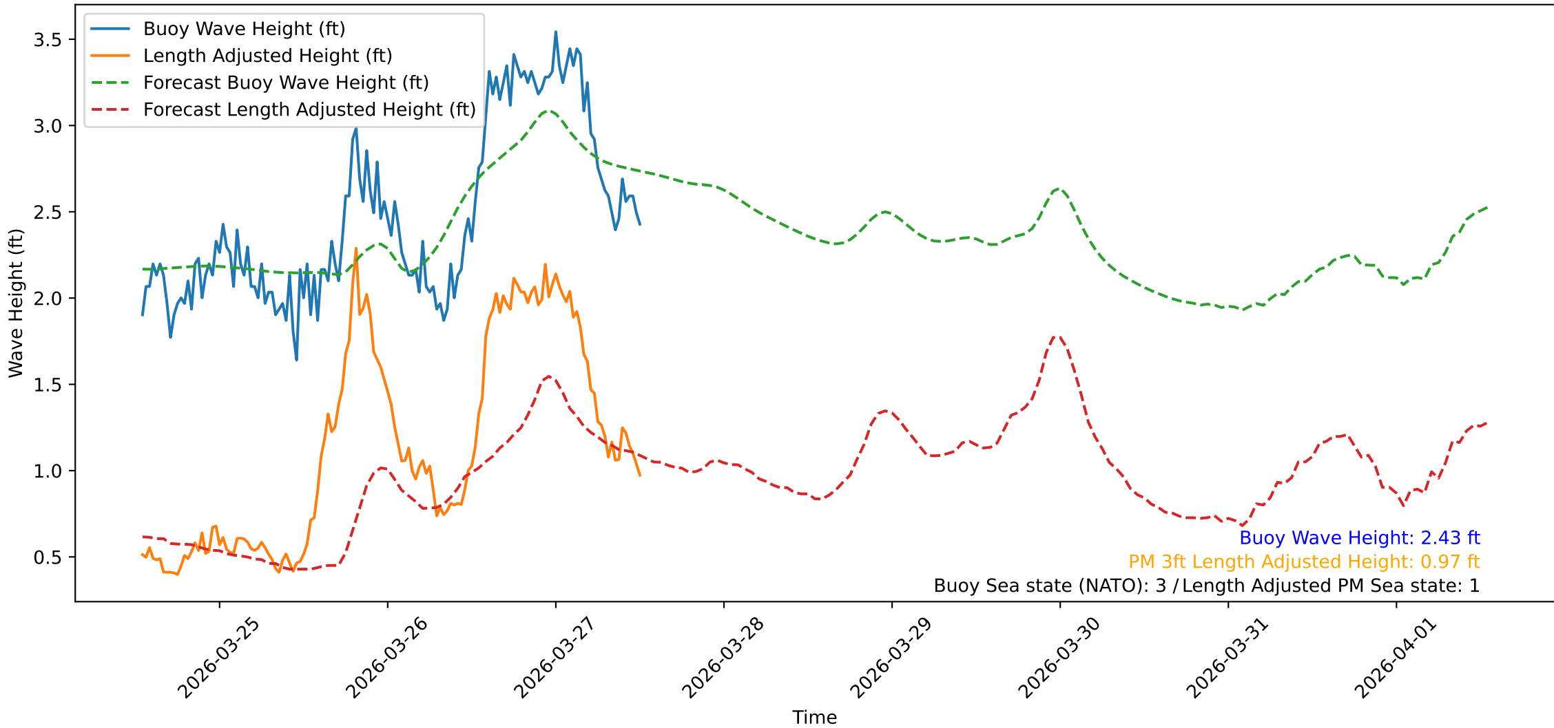
Wave Heights over Time for Green Beach at 2026-03-27 13:01:10
