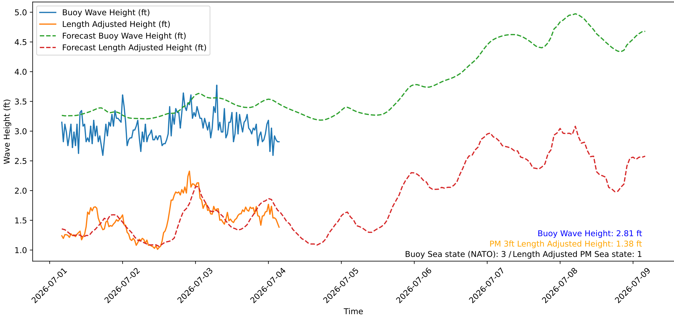
Wave Heights over Time for Oceanside Harbor at 2026-07-04 04:00:26
