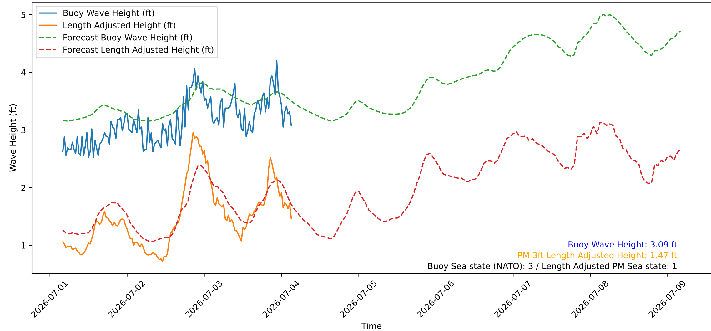
Wave Heights over Time for Green Beach at 2026-07-04 04:01:07
