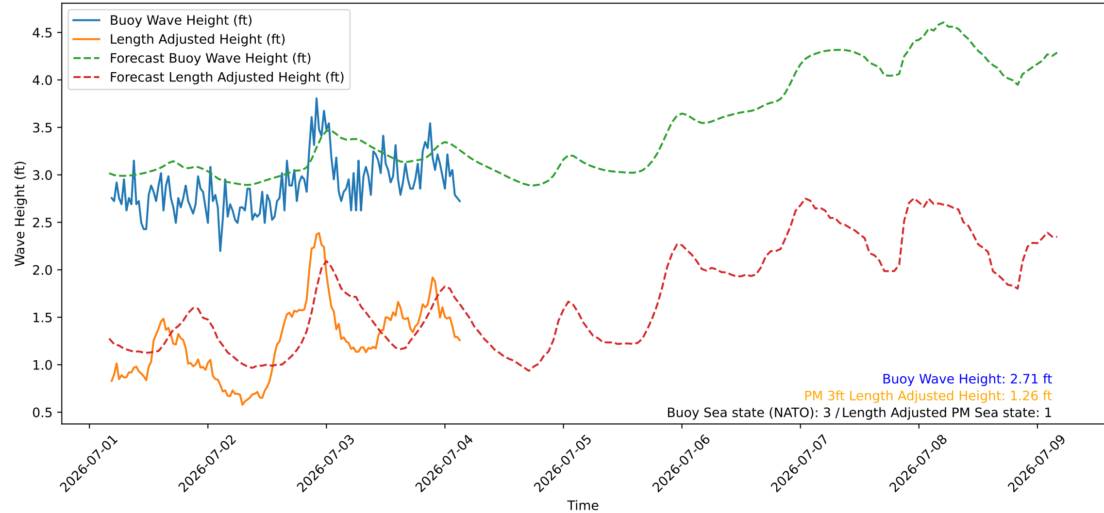
Wave Heights over Time for Red Beach at 2026-07-04 04:00:45
