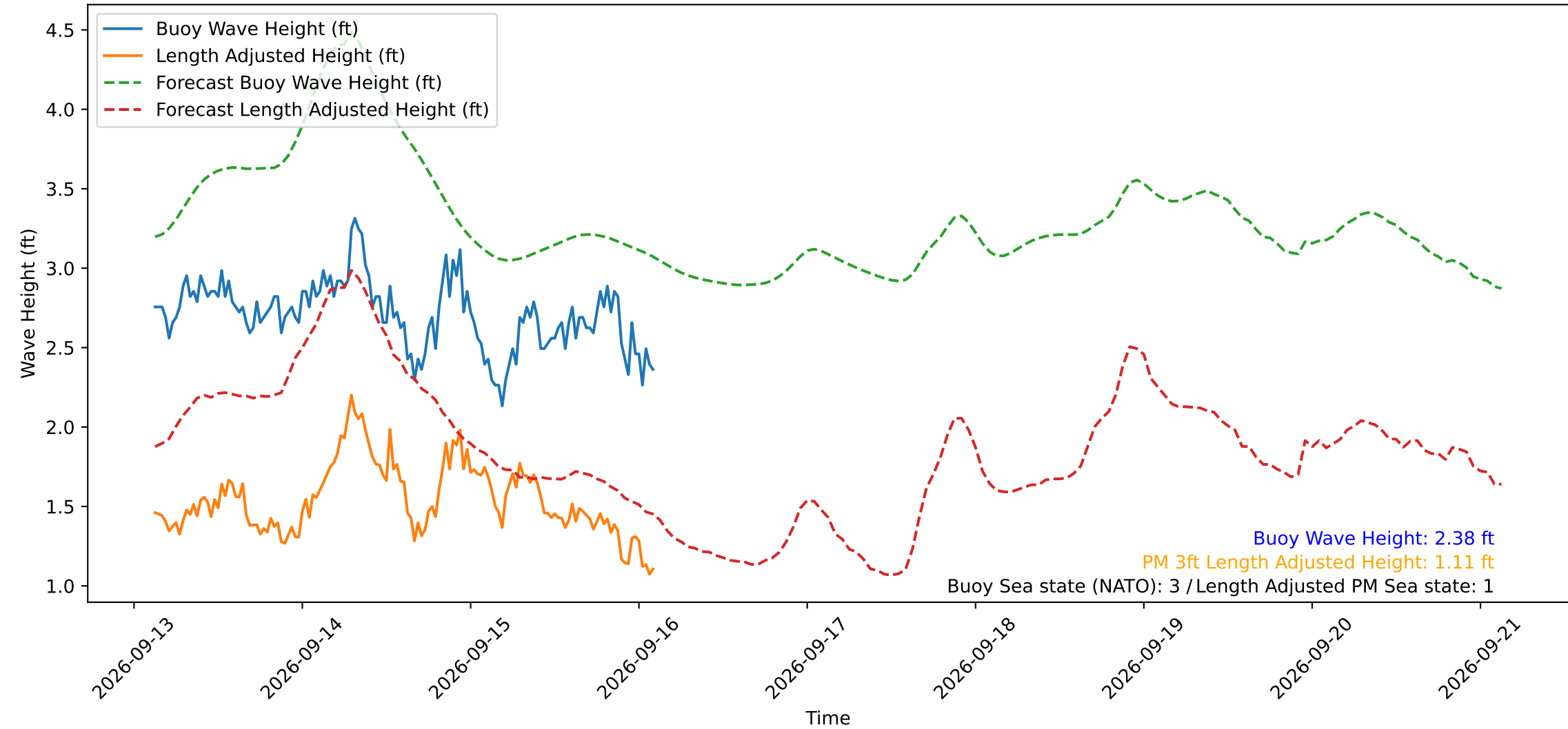
Wave Heights over Time for Green Beach at 2026-09-16 02:51:15
