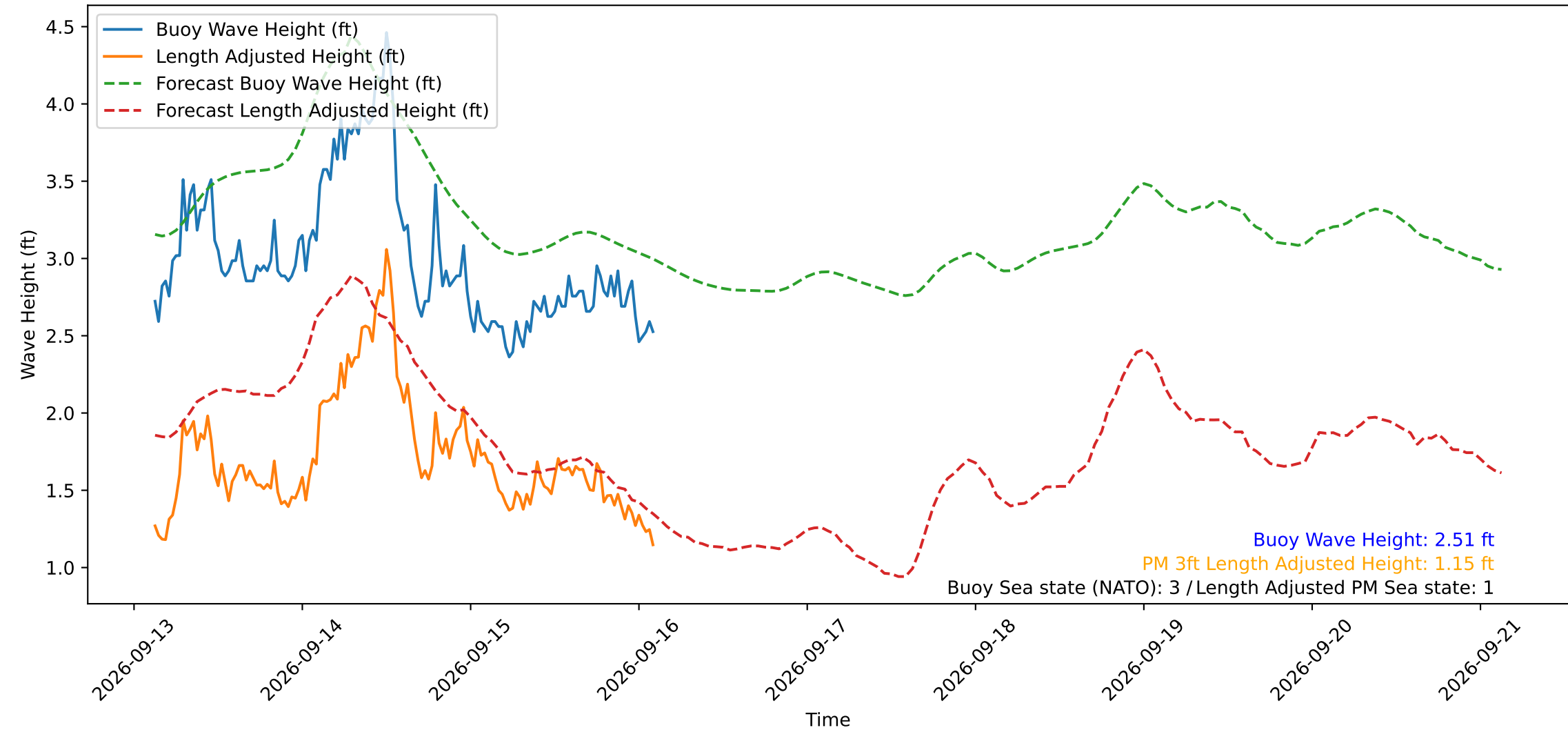
Wave Heights over Time for Oceanside Harbor at 2026-09-16 02:50:30
