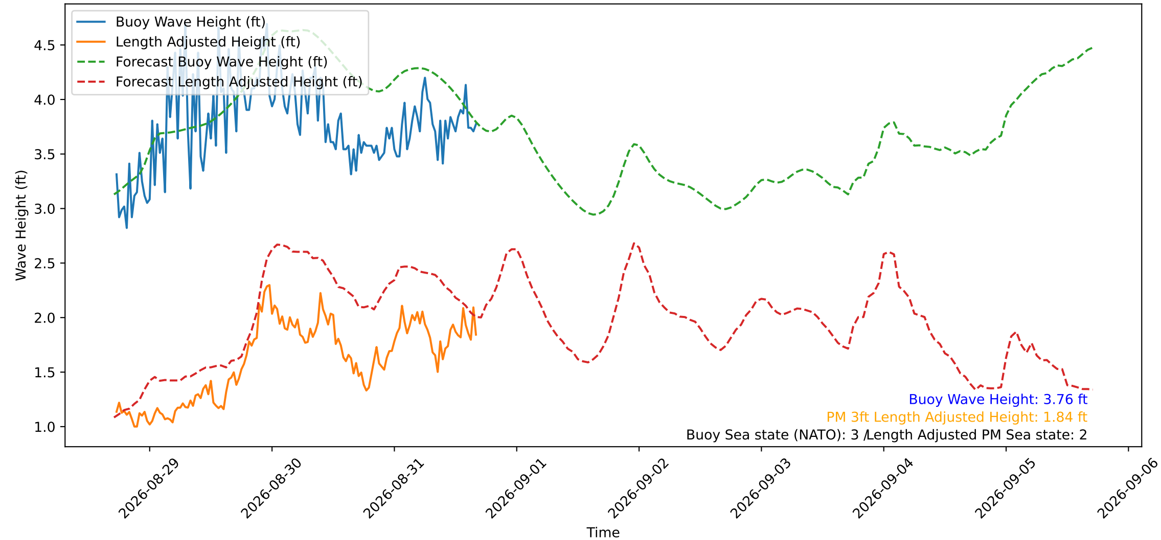
Wave Heights over Time for Red Beach at 2026-08-31 17:00:50
