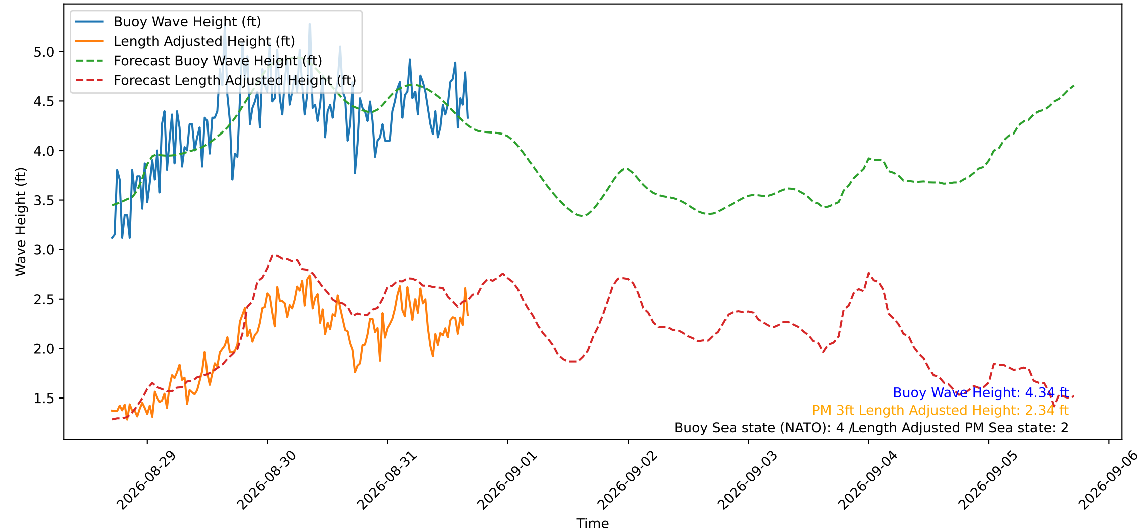
Wave Heights over Time for Oceanside Harbor at 2026-08-31 17:00:30
