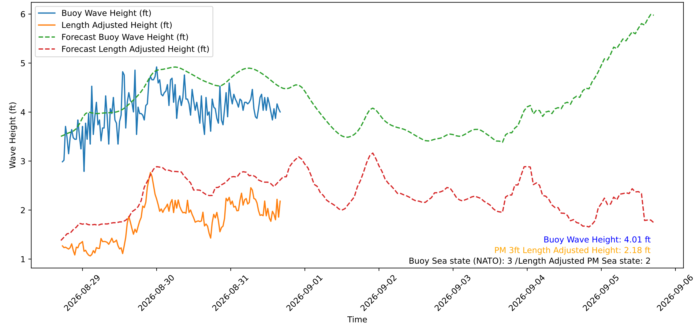
Wave Heights over Time for Green Beach at 2026-08-31 17:01:14
