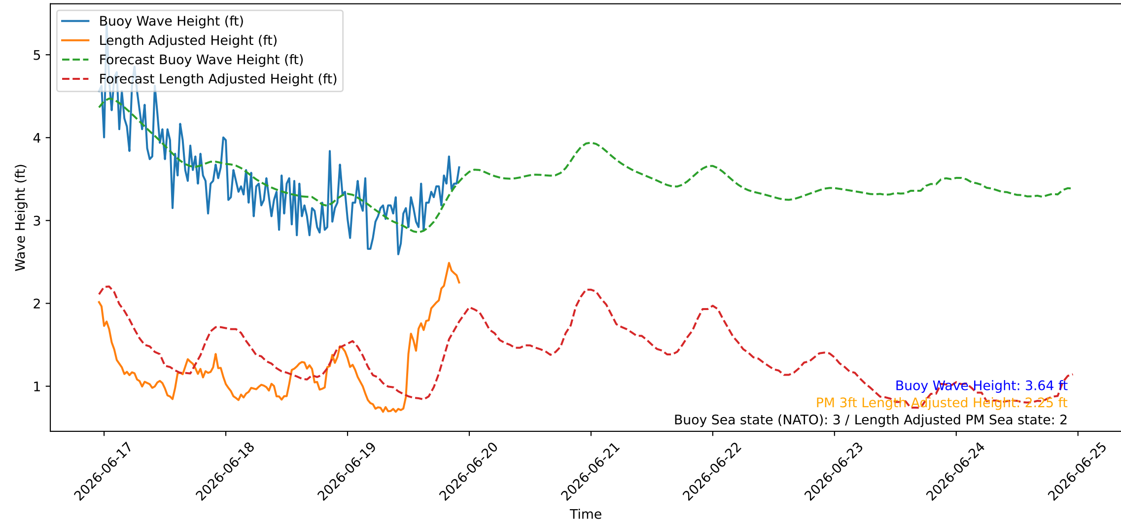
Wave Heights over Time for Red Beach at 2026-06-19 22:40:46
