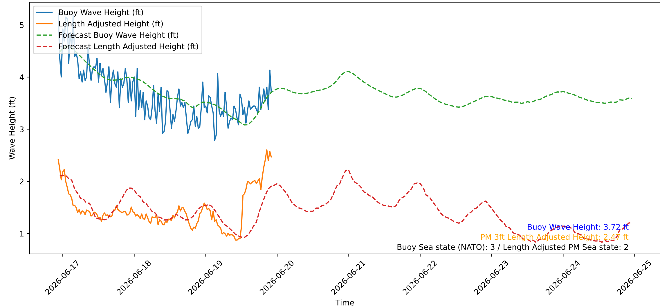
Wave Heights over Time for Oceanside Harbor at 2026-06-19 22:40:26
