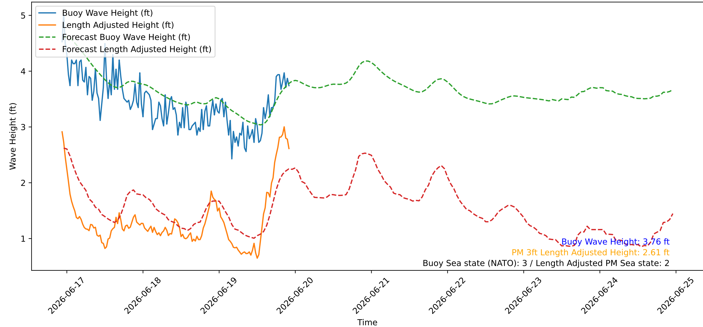
Wave Heights over Time for Green Beach at 2026-06-19 22:41:09
