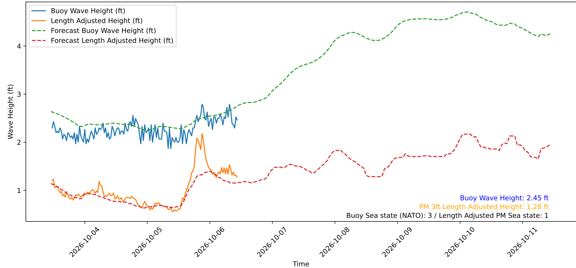
Wave Heights over Time for Oceanside Harbor at 2026-10-06 11:20:30
