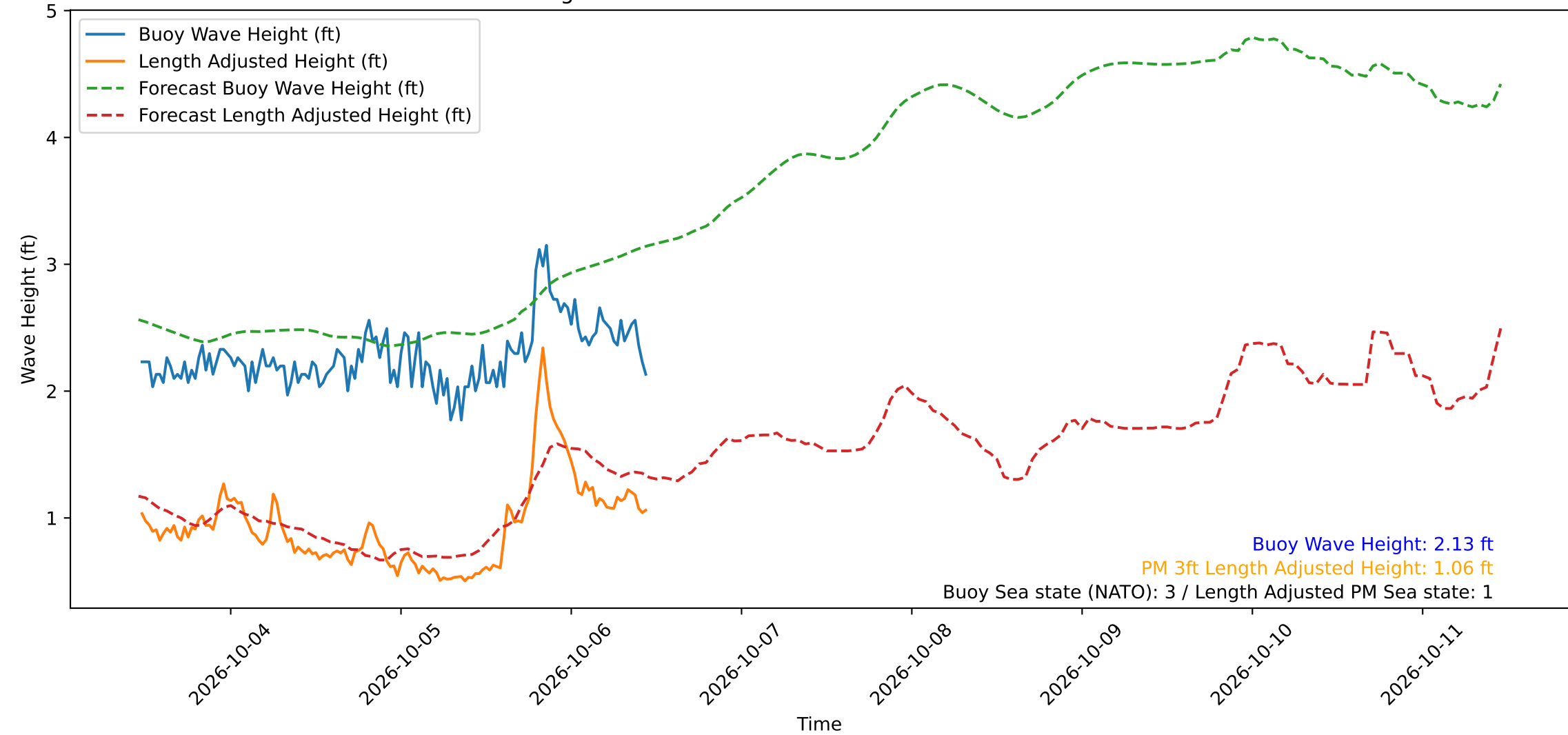
Wave Heights over Time for Green Beach at 2026-10-06 11:21:14
