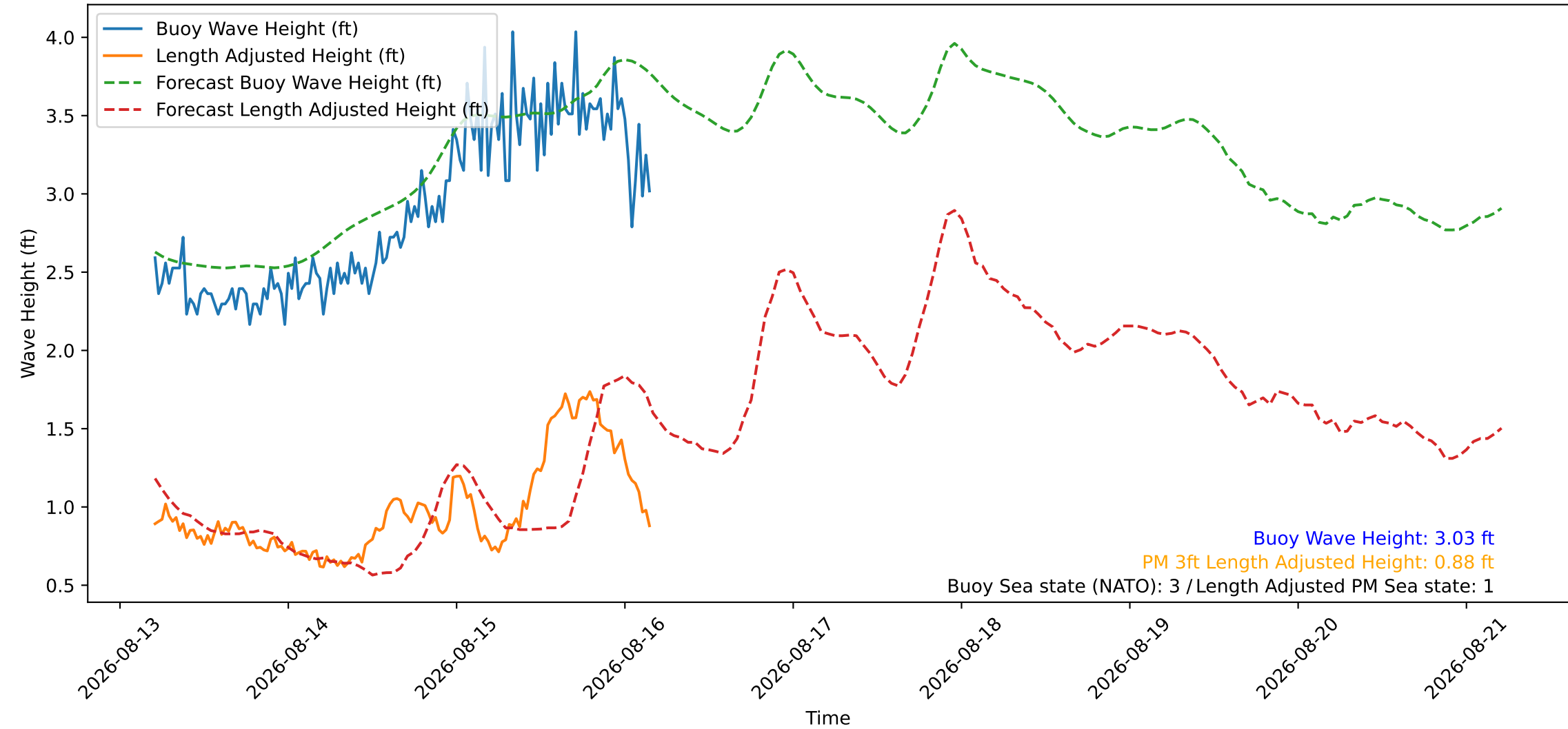
Wave Heights over Time for Red Beach at 2026-08-16 04:30:46
