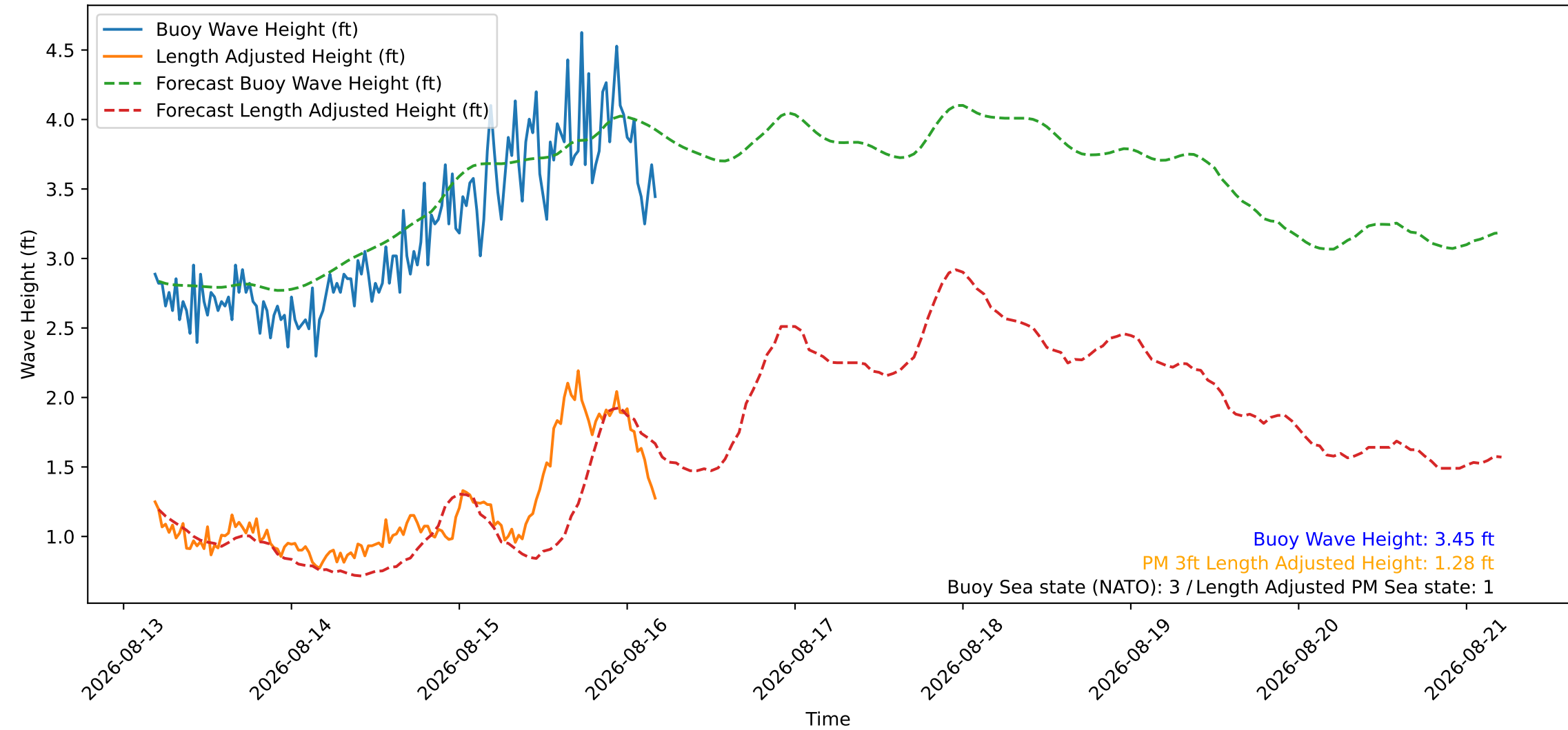
Wave Heights over Time for Oceanside Harbor at 2026-08-16 04:30:27
