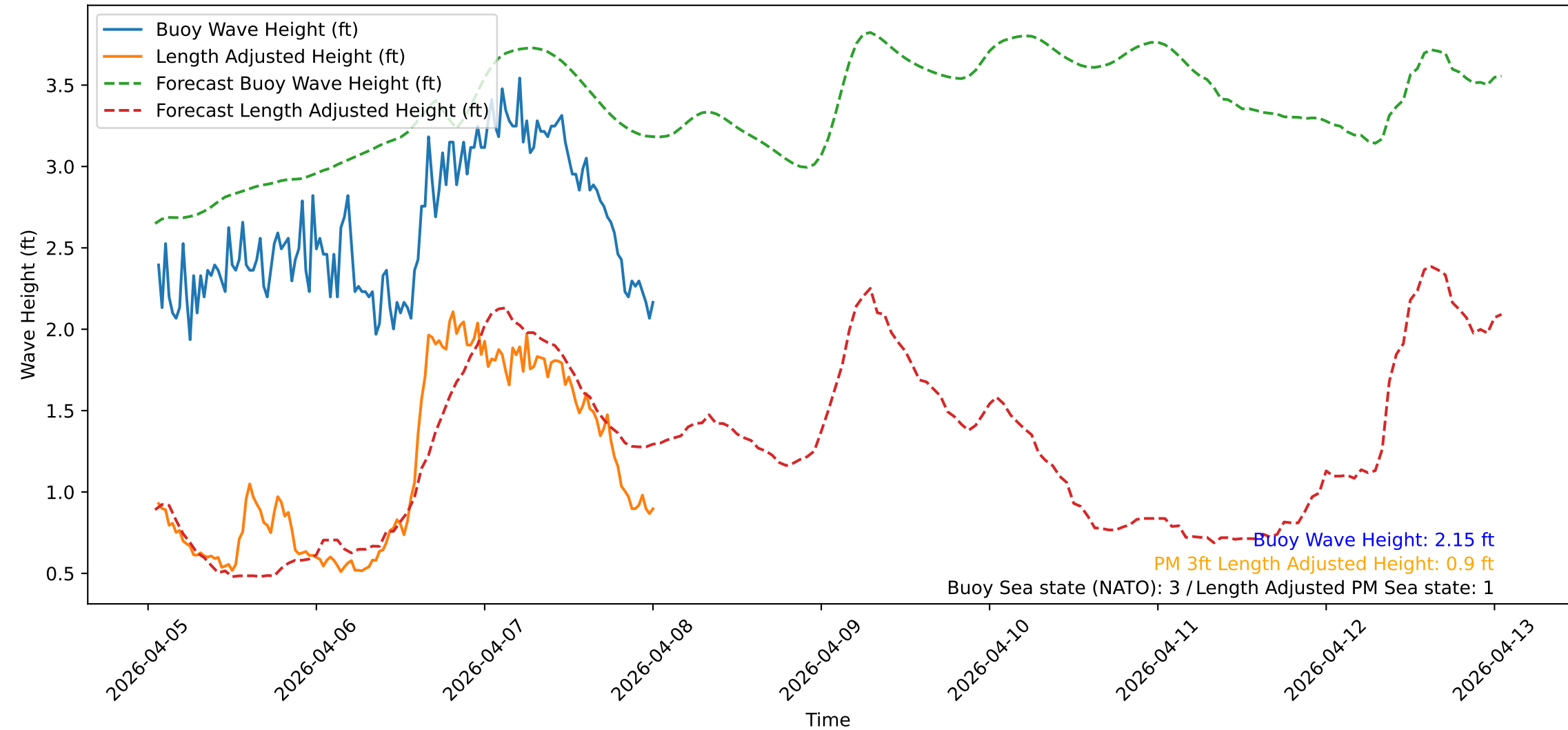
Wave Heights over Time for Red Beach at 2026-04-08 01:00:48
