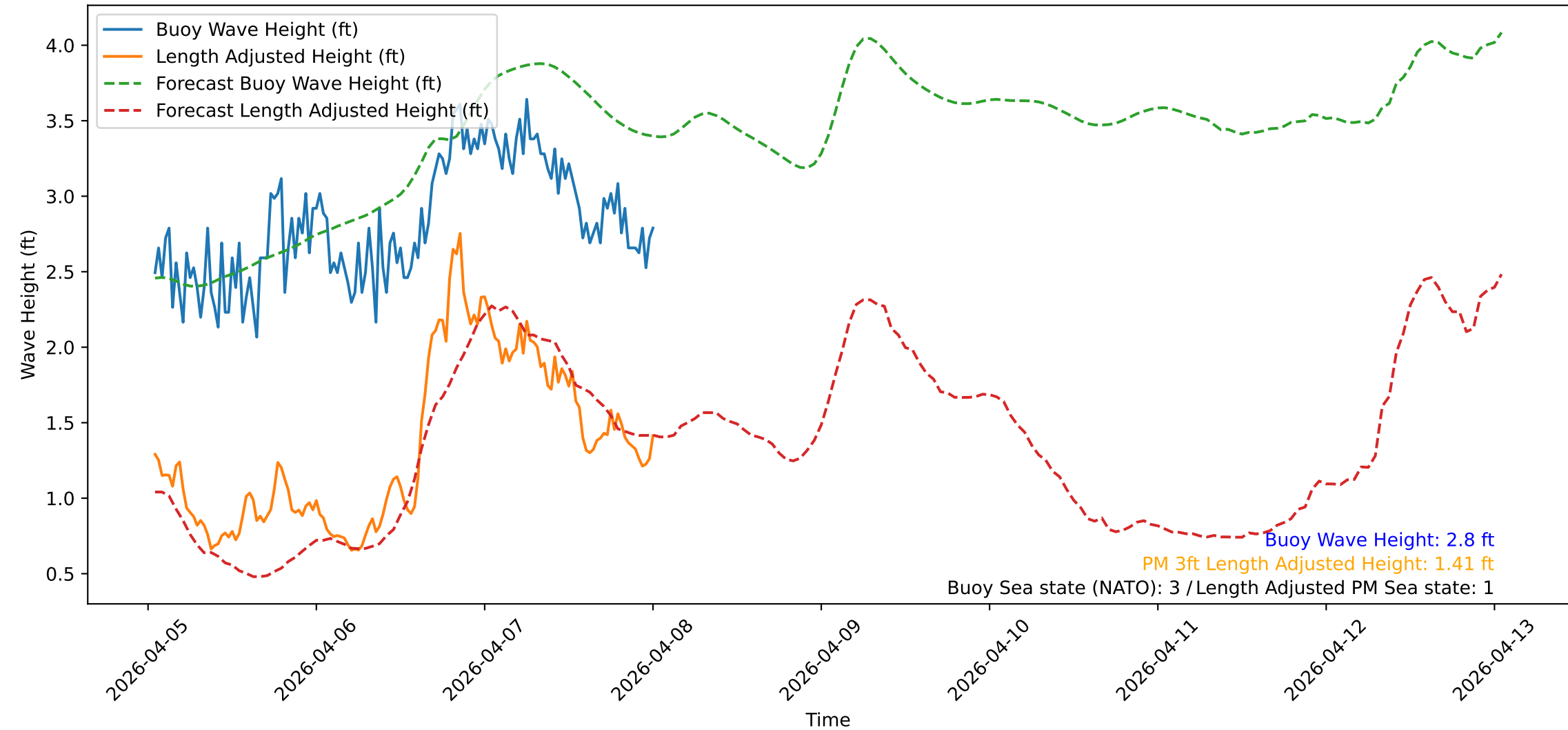
Wave Heights over Time for Oceanside Harbor at 2026-04-08 01:00:32
