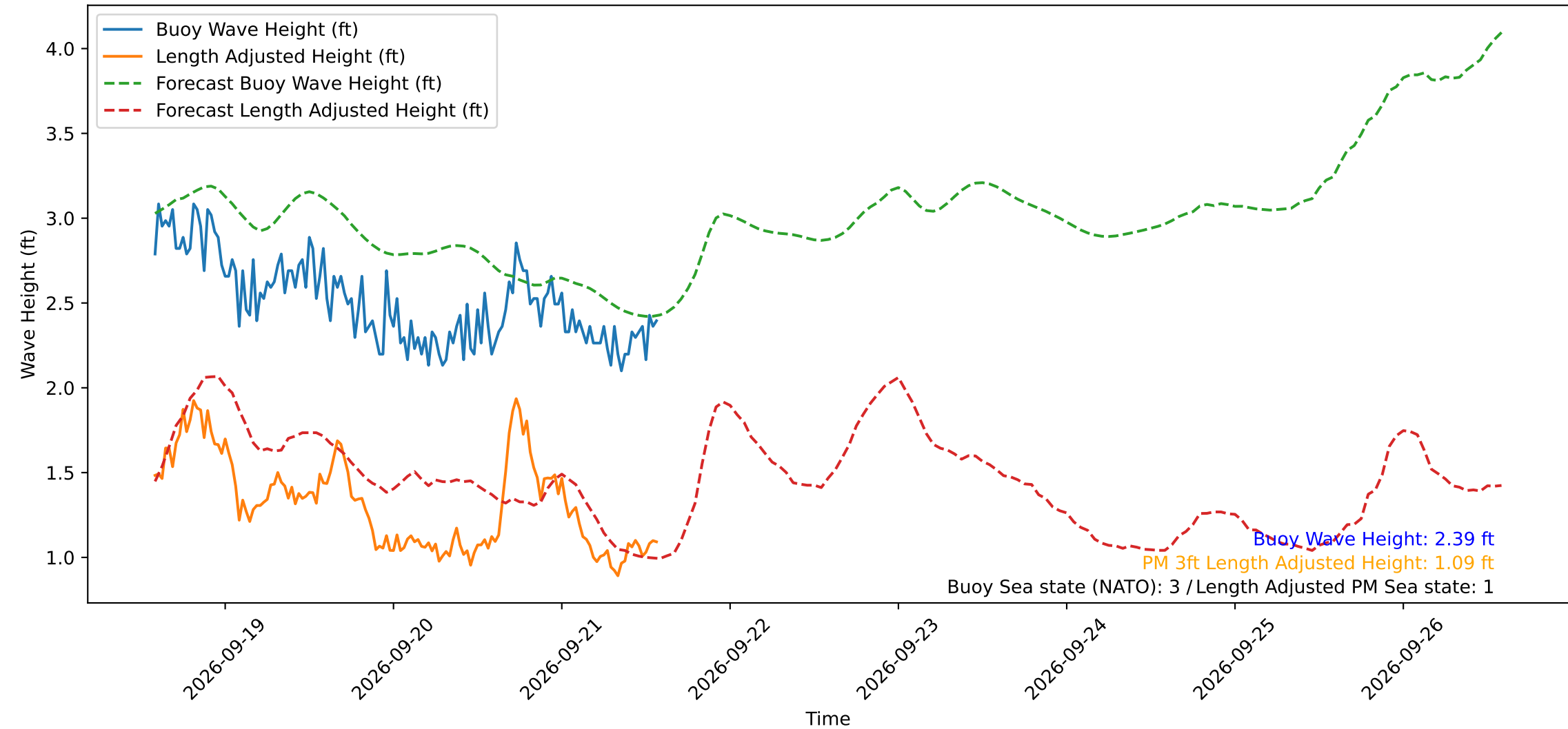
Wave Heights over Time for Oceanside Harbor at 2026-09-21 14:10:29
