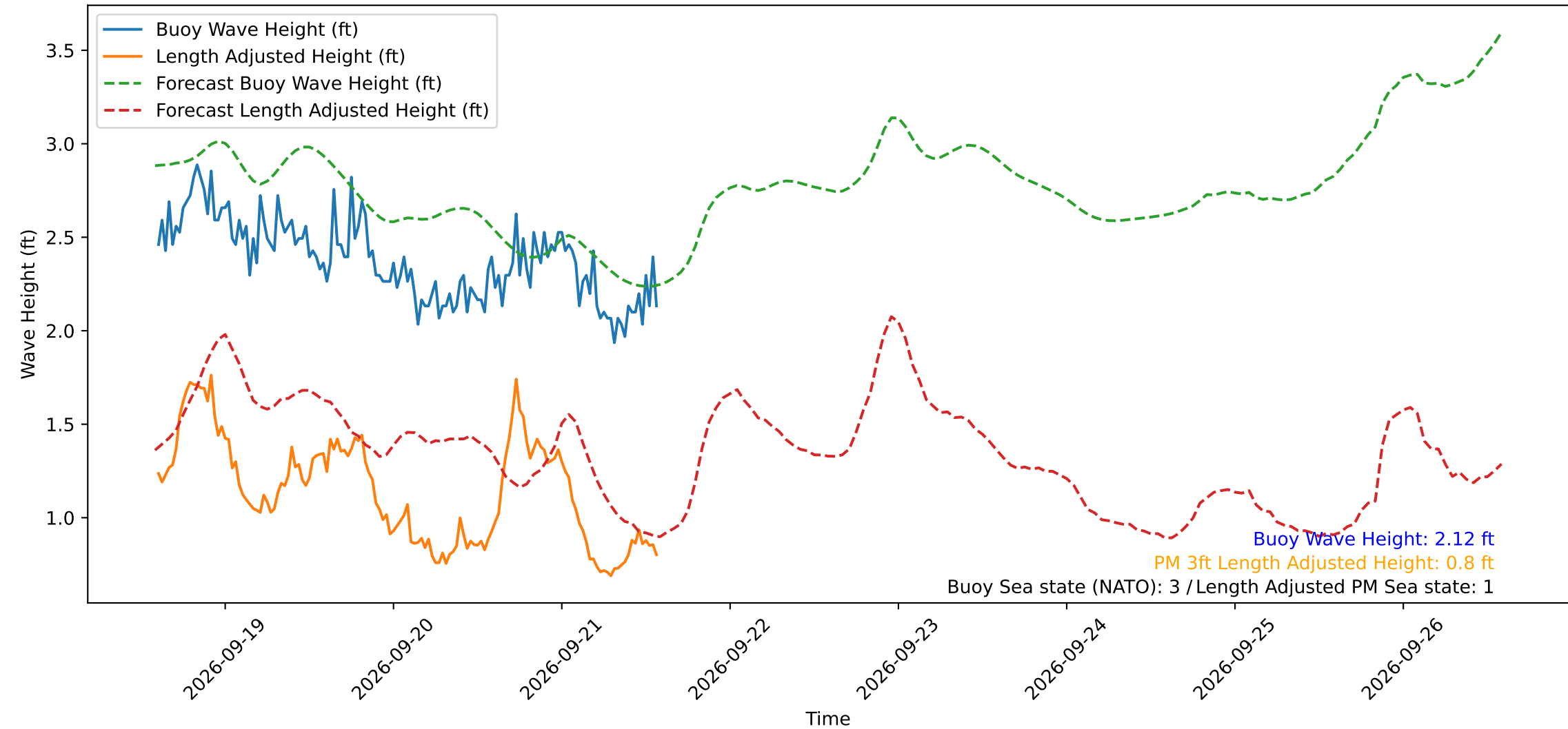
Wave Heights over Time for Red Beach at 2026-09-21 14:10:49
