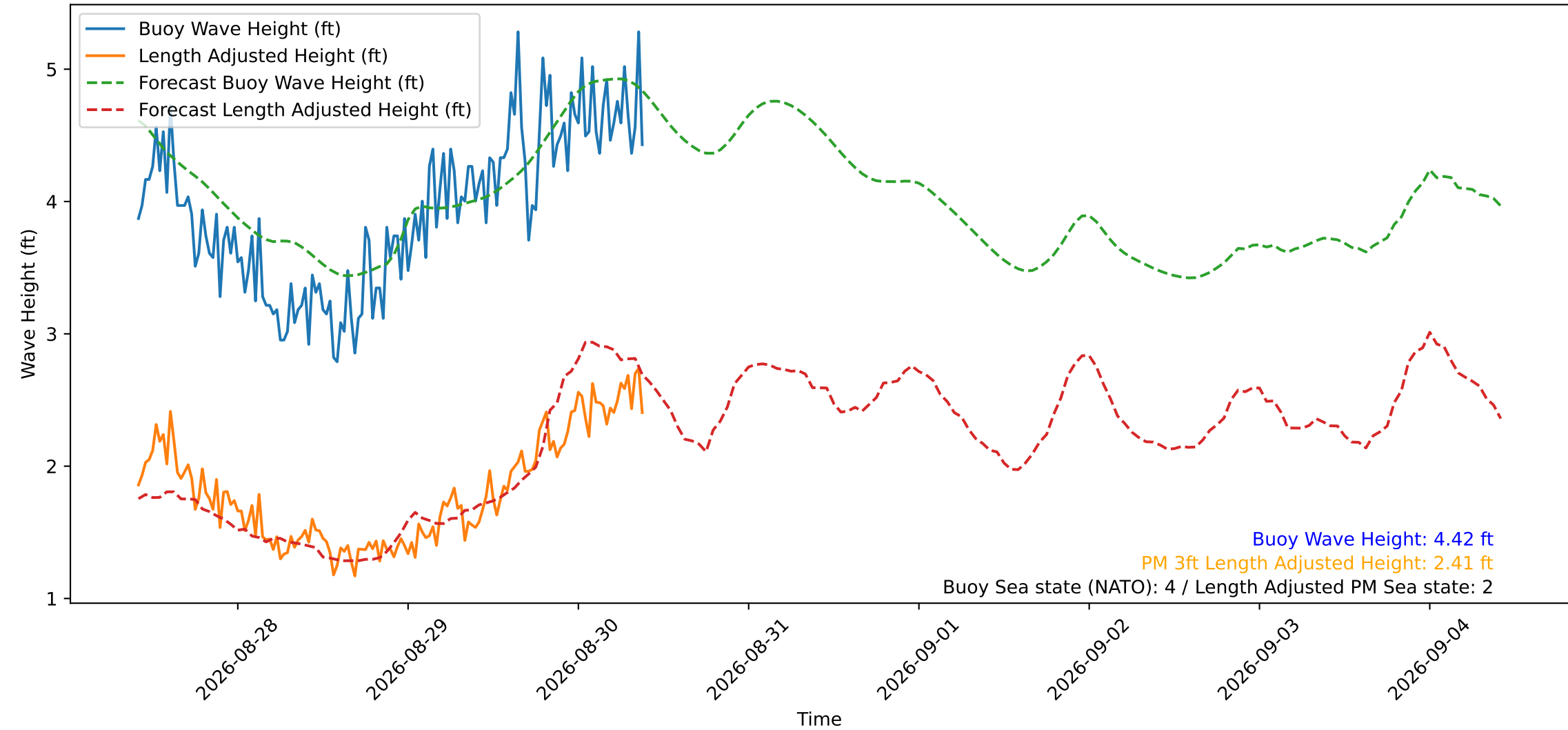
Wave Heights over Time for Oceanside Harbor at 2026-08-30 09:50:30
