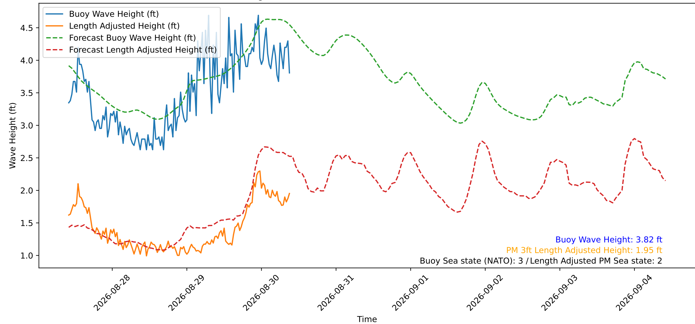
Wave Heights over Time for Red Beach at 2026-08-30 09:50:51
