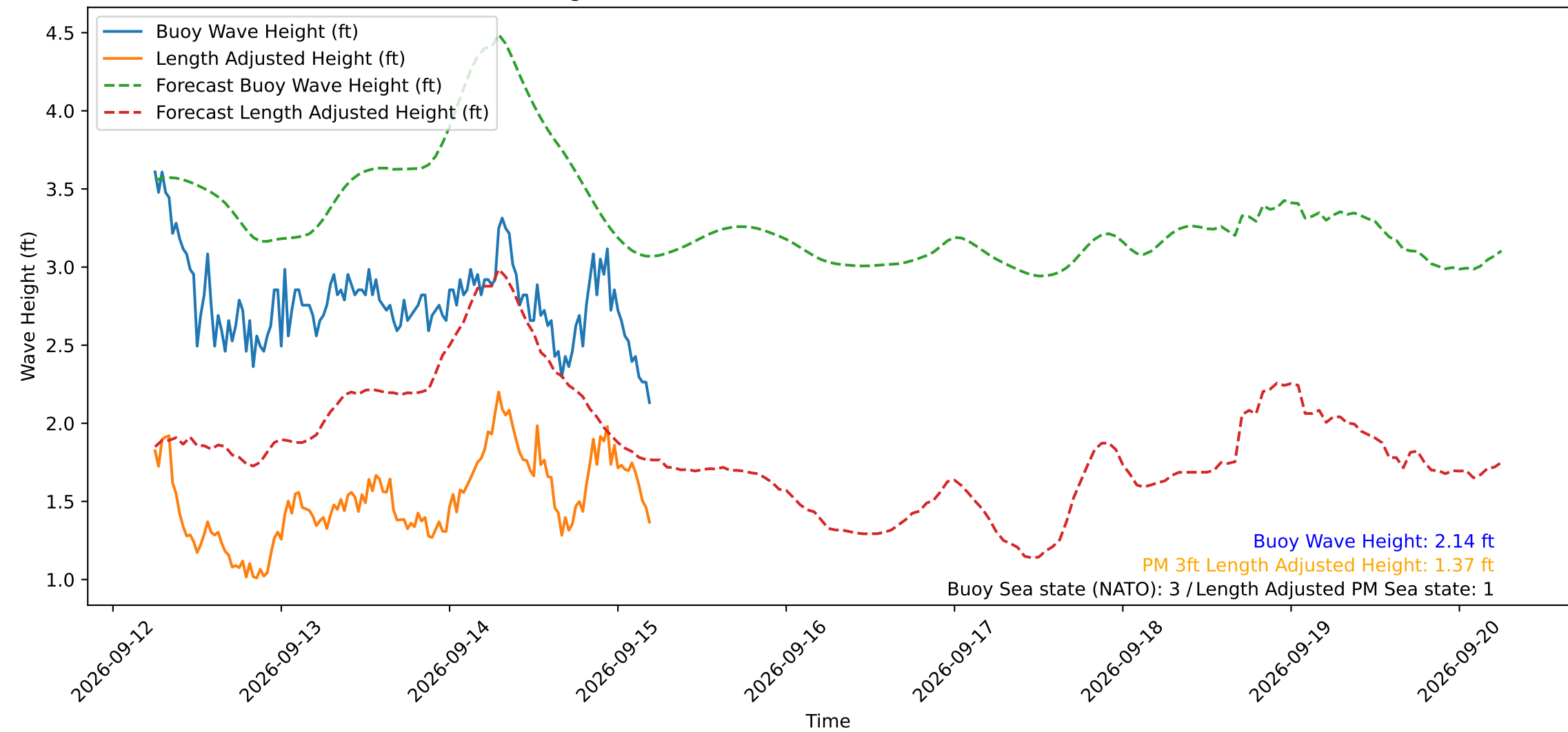
Wave Heights over Time for Green Beach at 2026-09-15 05:31:12
