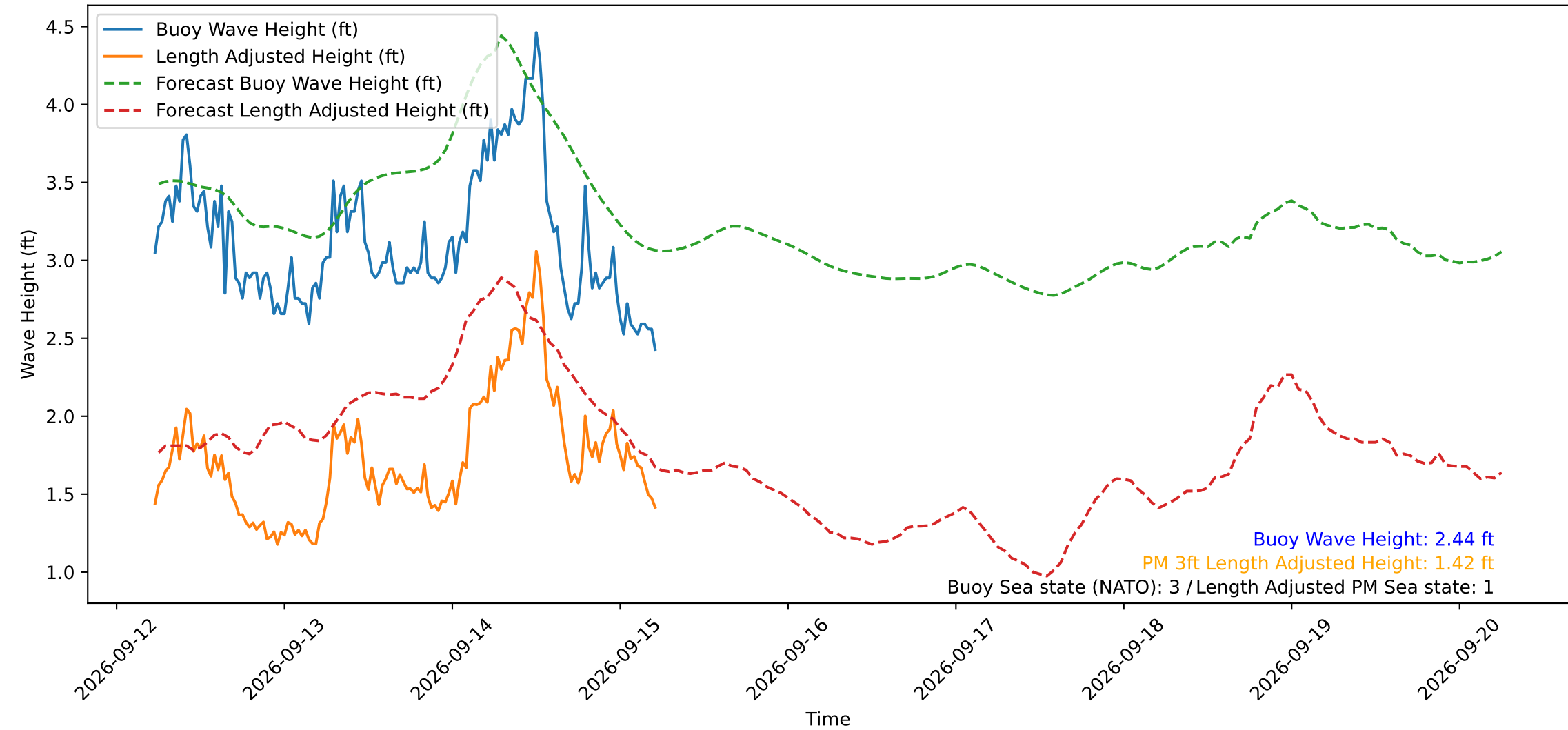
Wave Heights over Time for Oceanside Harbor at 2026-09-15 05:30:30
