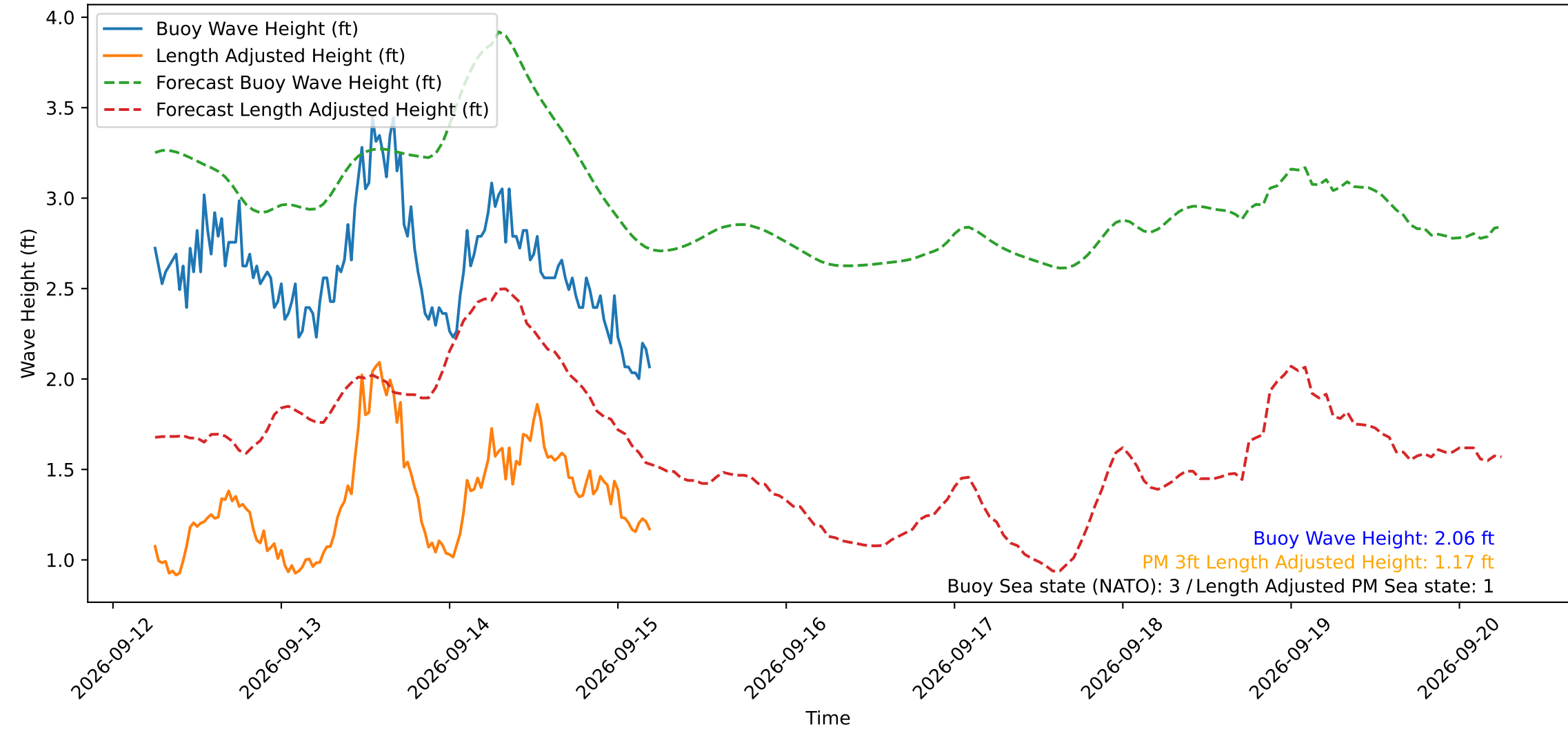
Wave Heights over Time for Red Beach at 2026-09-15 05:30:50
