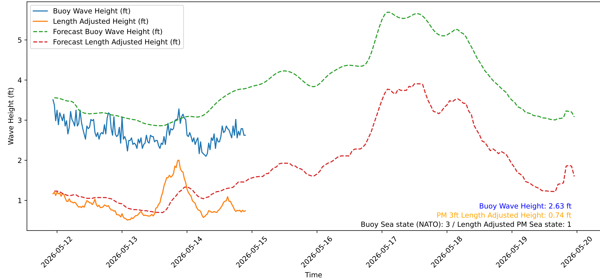
Wave Heights over Time for Green Beach at 2026-05-14 22:31:13
