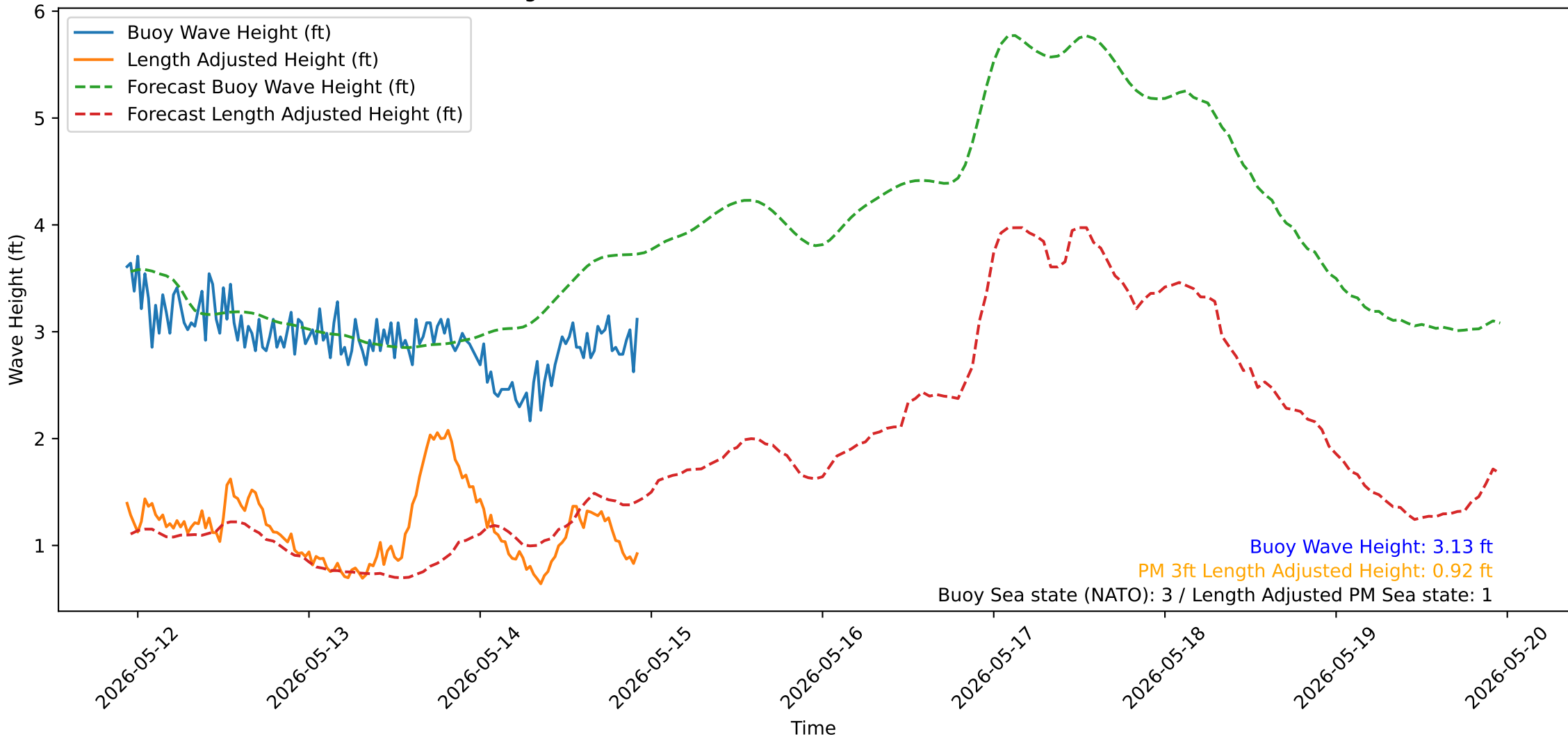
Wave Heights over Time for Oceanside Harbor at 2026-05-14 22:30:31
