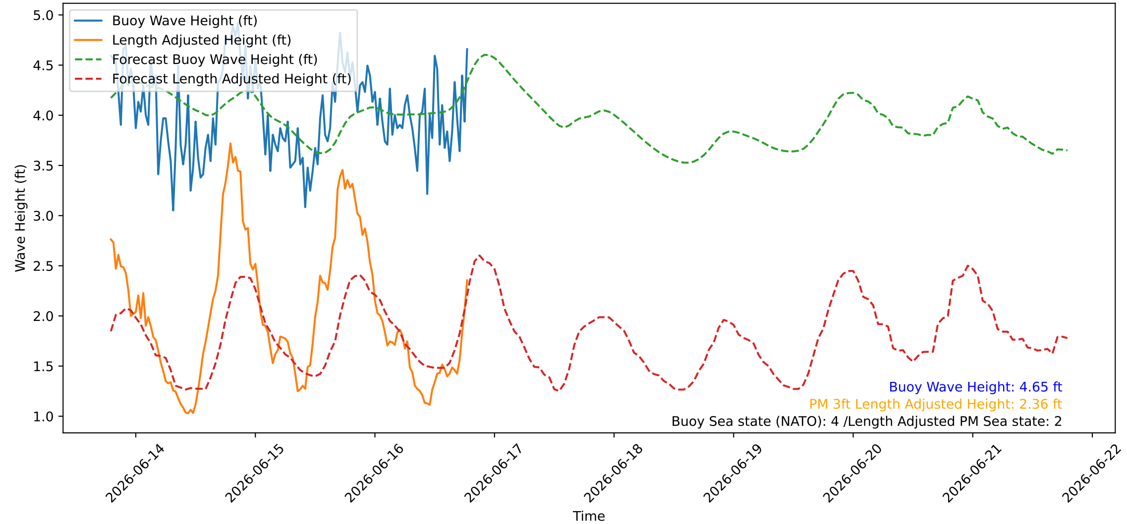
Wave Heights over Time for Green Beach at 2026-06-16 19:11:12
