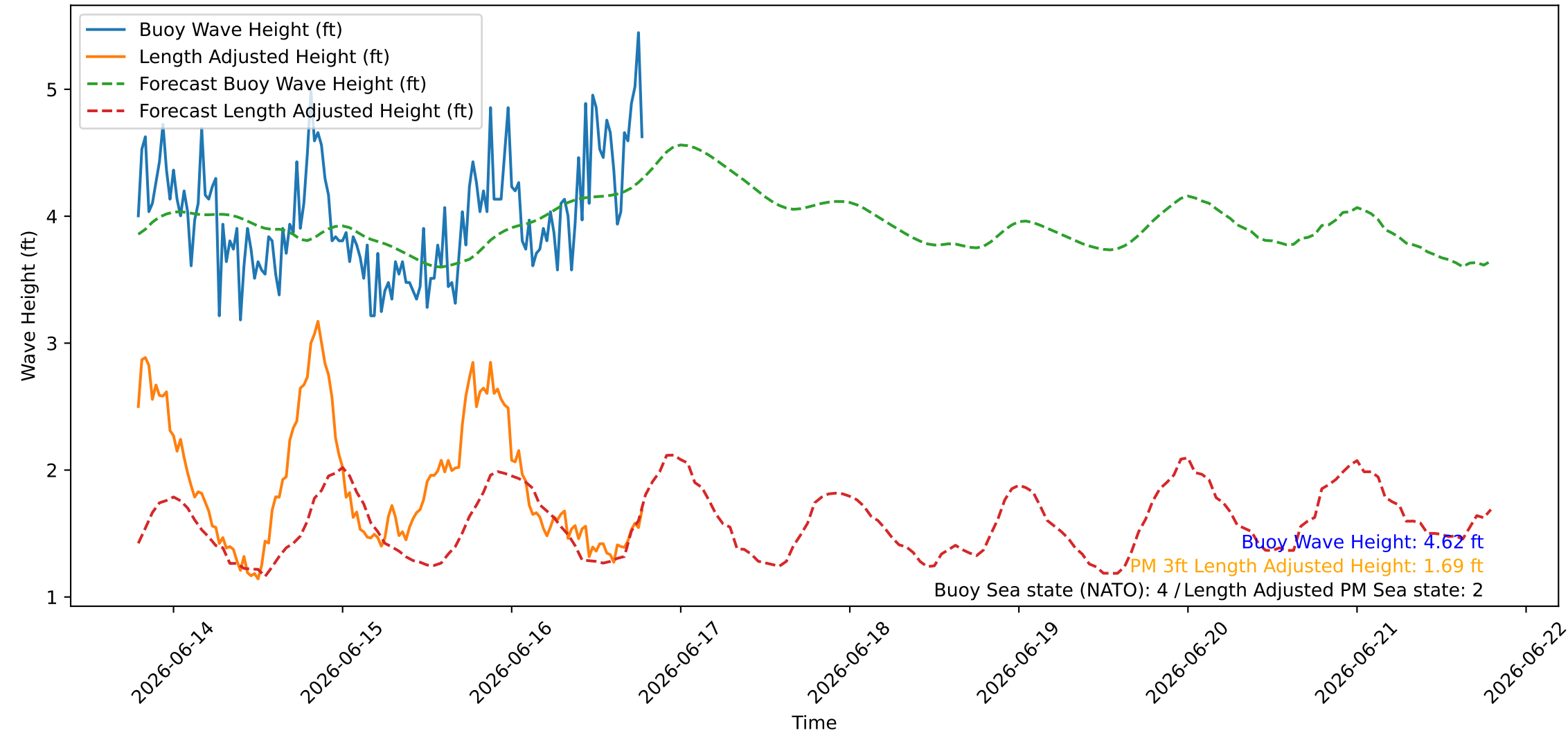
Wave Heights over Time for Oceanside Harbor at 2026-06-16 19:10:26
