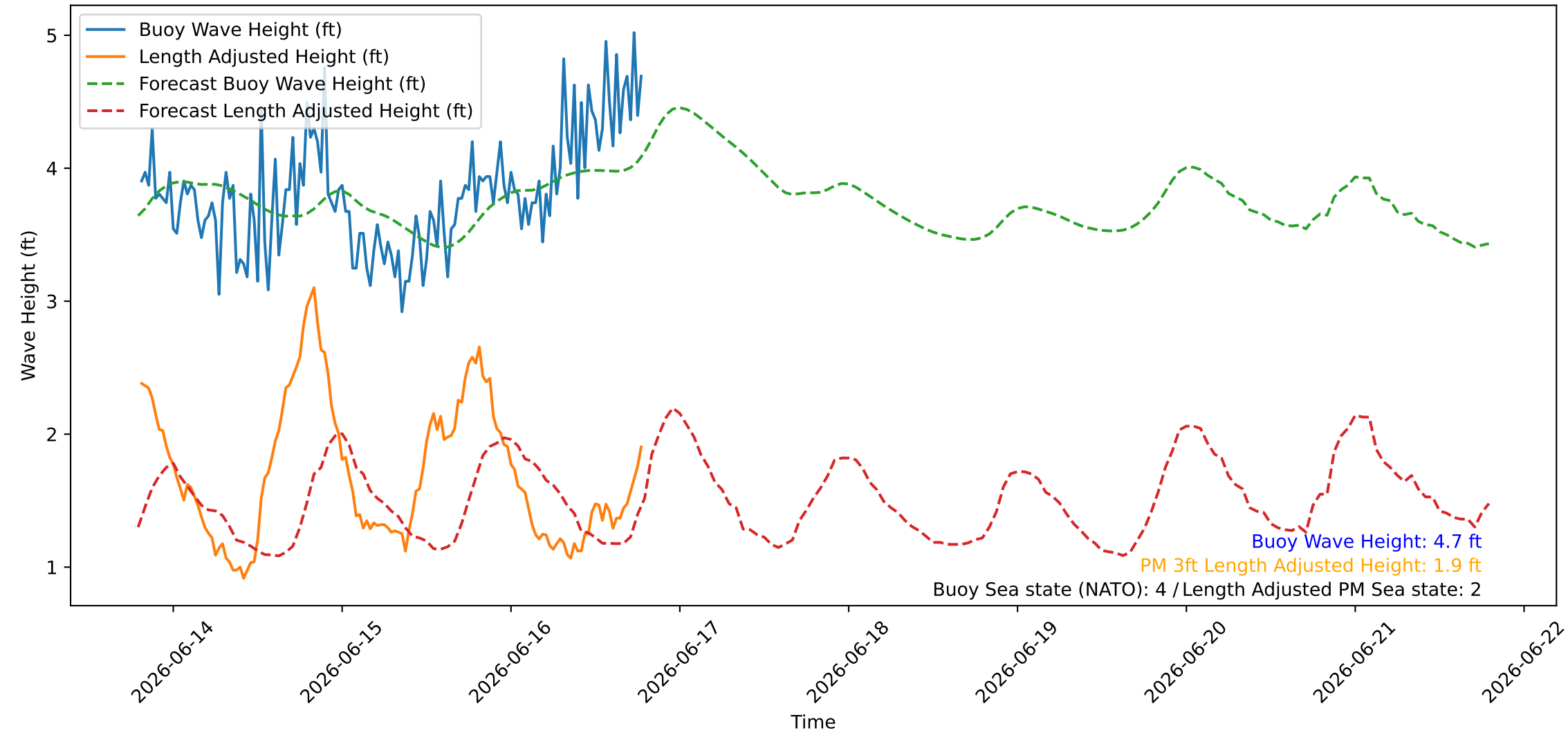
Wave Heights over Time for Red Beach at 2026-06-16 19:10:49
