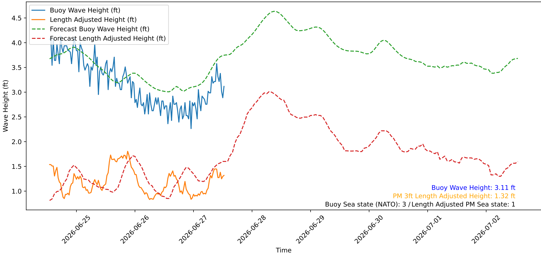
Wave Heights over Time for Green Beach at 2026-06-27 13:11:08
