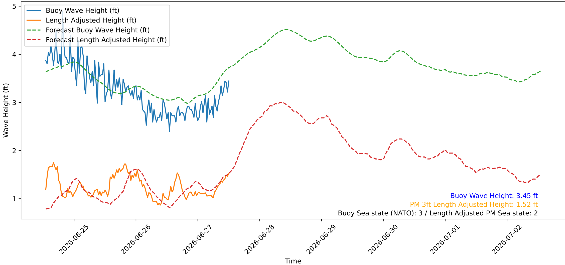
Wave Heights over Time for Oceanside Harbor at 2026-06-27 13:10:26
