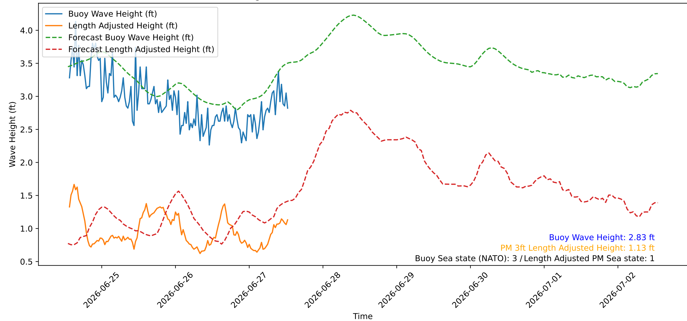
Wave Heights over Time for Red Beach at 2026-06-27 13:10:45
