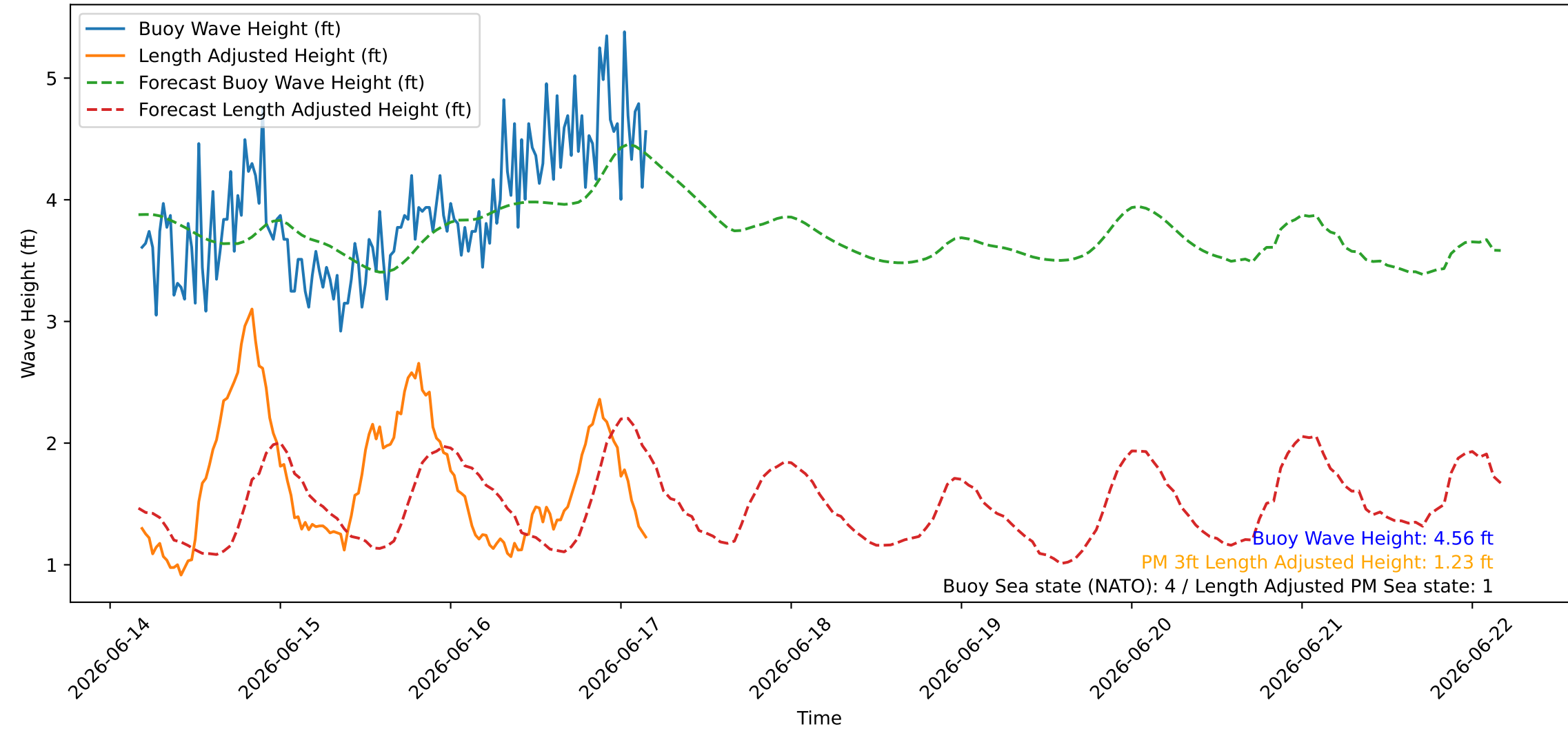
Wave Heights over Time for Red Beach at 2026-06-17 04:10:45
