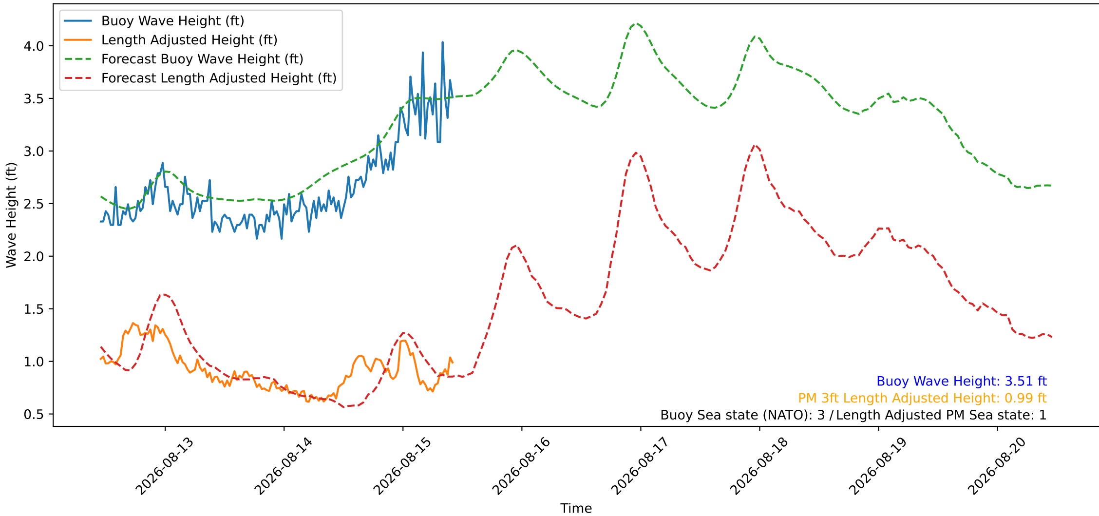
Wave Heights over Time for Red Beach at 2026-08-15 10:50:47
