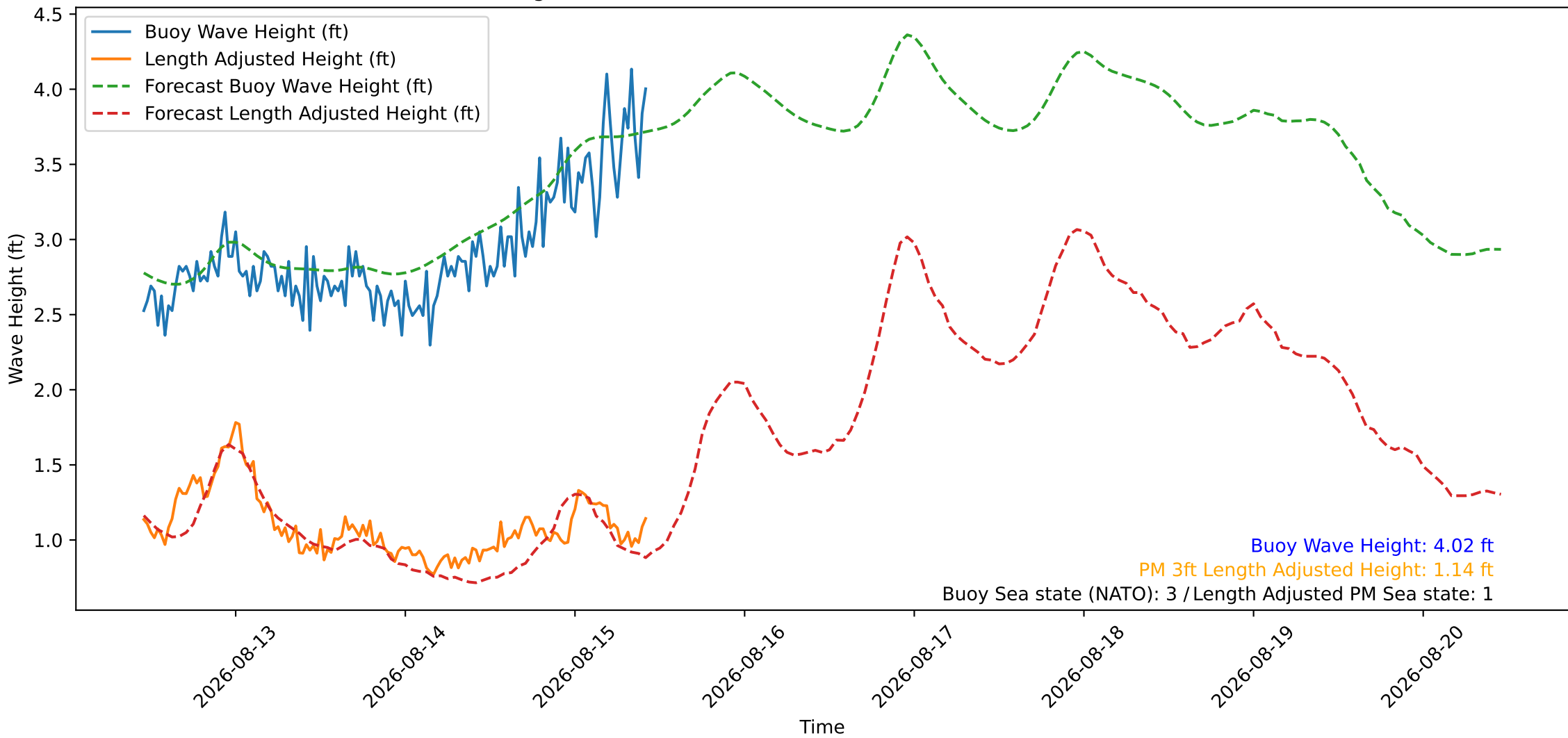
Wave Heights over Time for Oceanside Harbor at 2026-08-15 10:50:27
