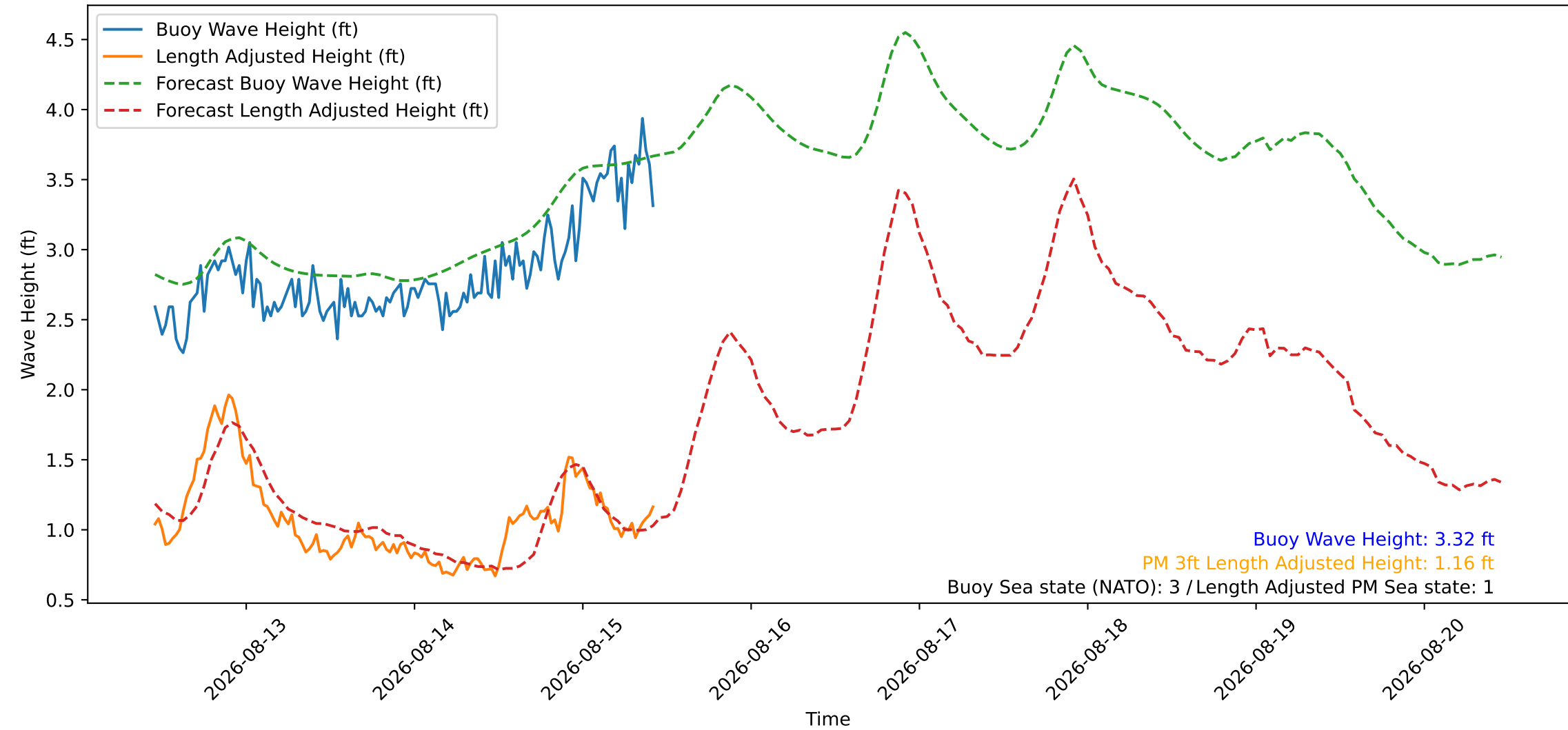
Wave Heights over Time for Green Beach at 2026-08-15 10:51:10
