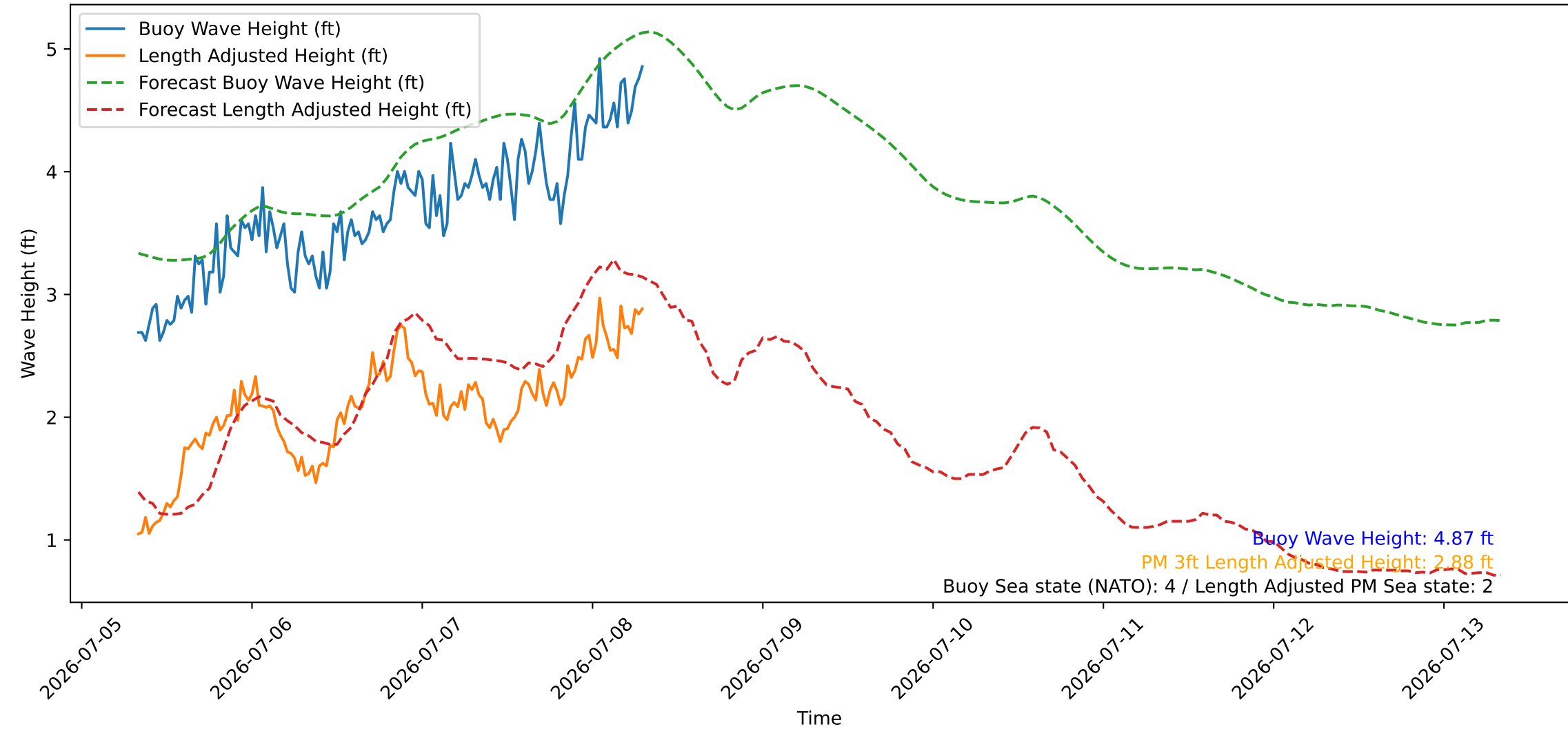
Wave Heights over Time for Oceanside Harbor at 2026-07-08 07:50:26
