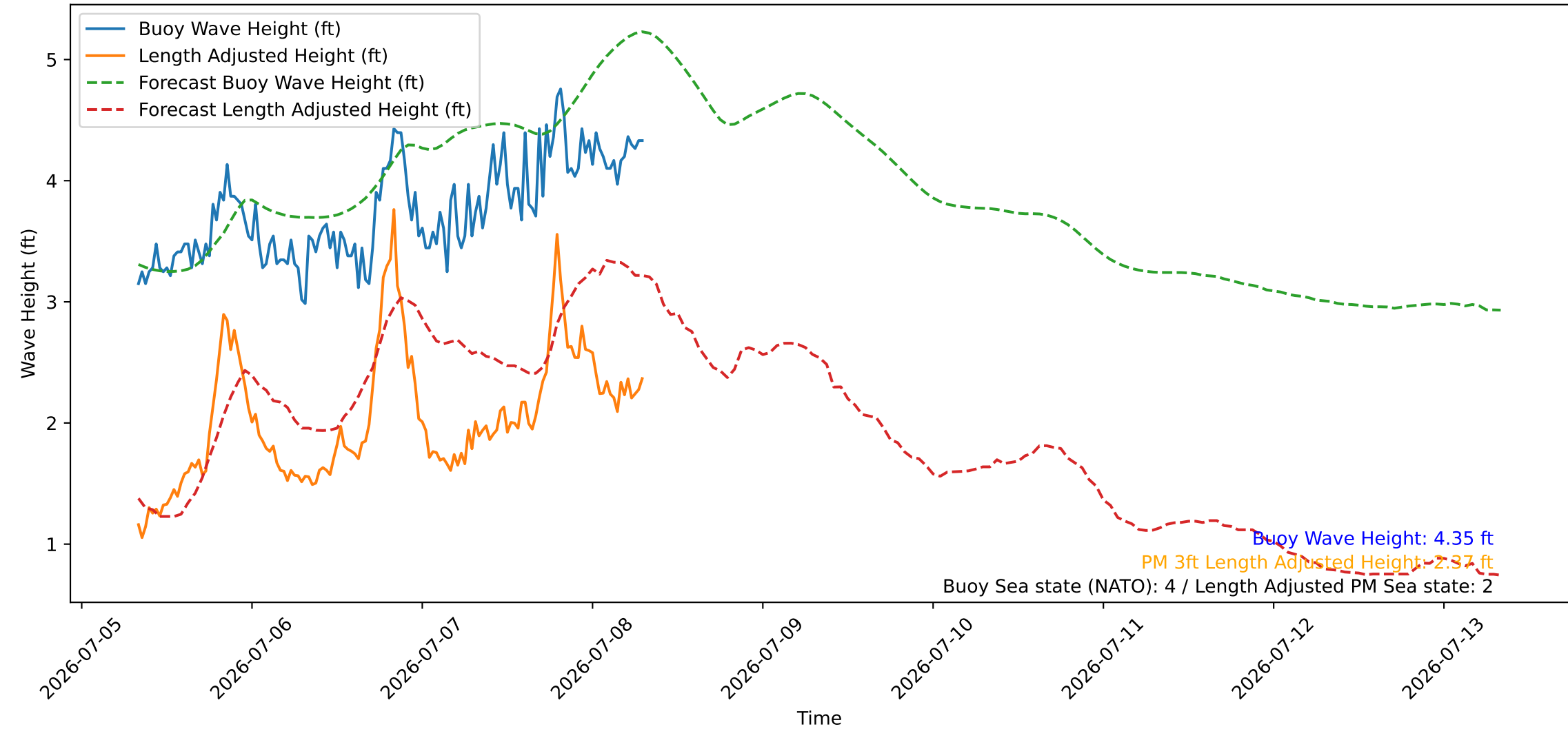
Wave Heights over Time for Green Beach at 2026-07-08 07:51:09
