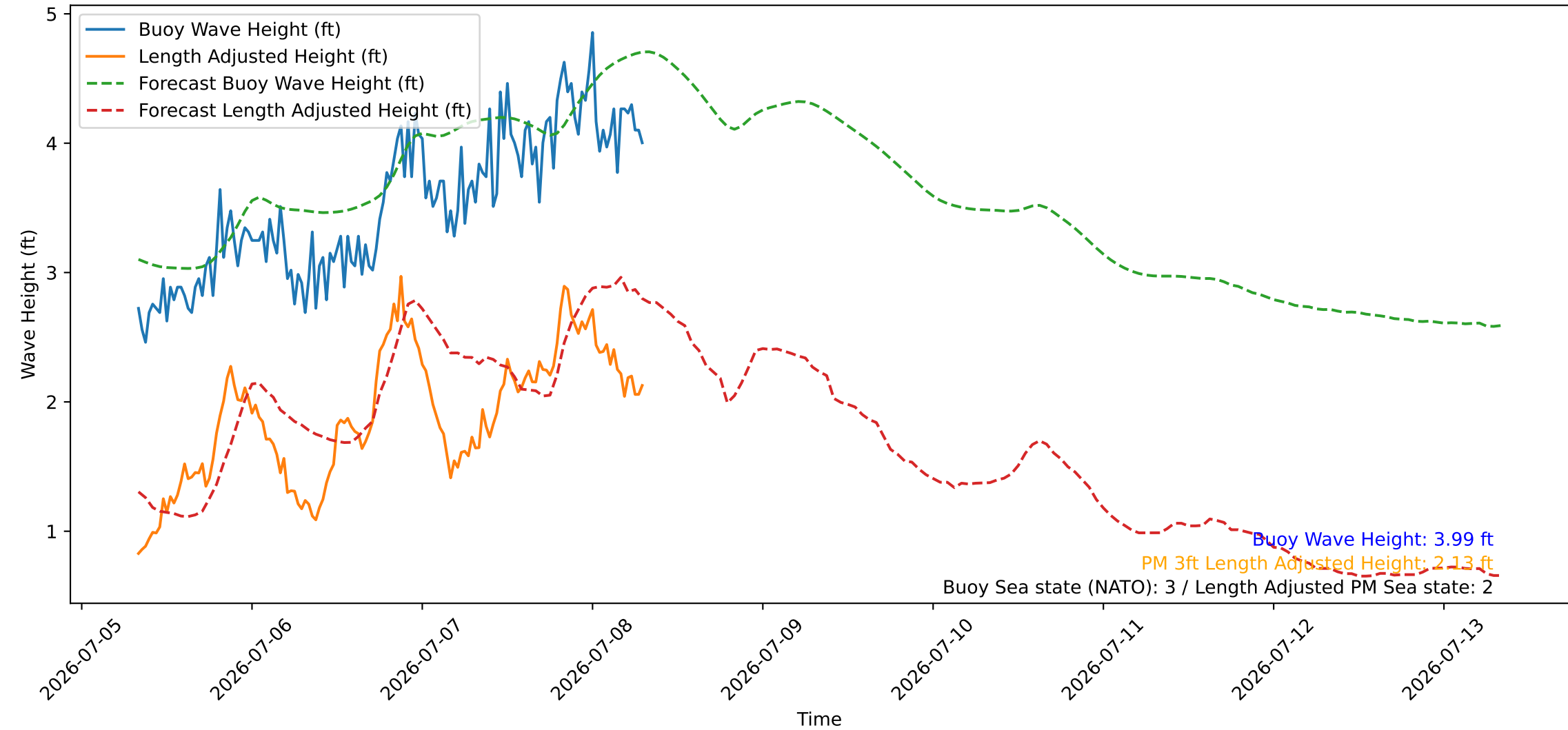
Wave Heights over Time for Red Beach at 2026-07-08 07:50:47
