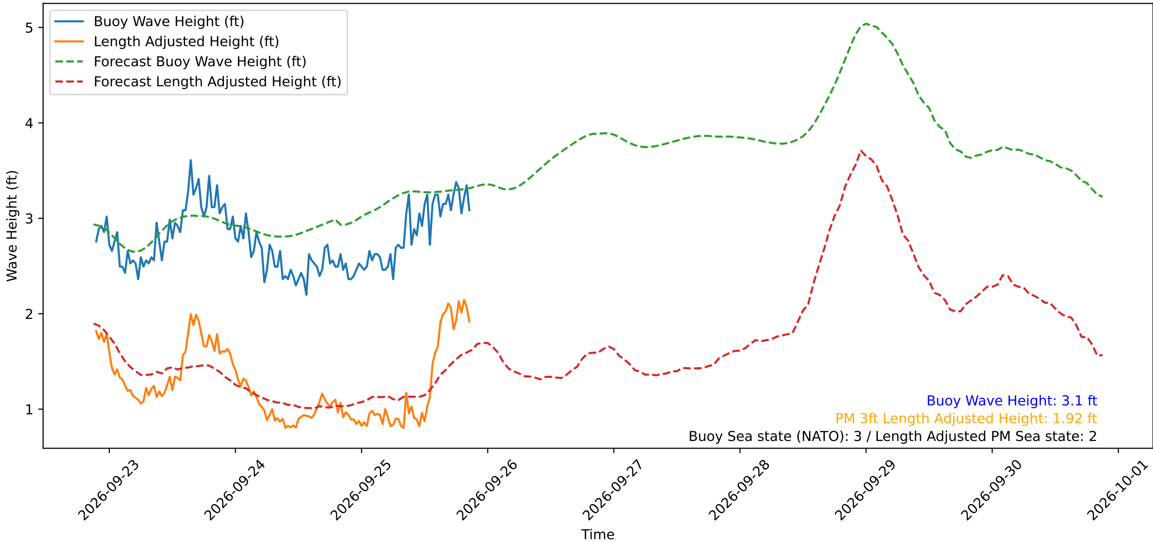
Wave Heights over Time for Oceanside Harbor at 2026-09-25 21:20:30
