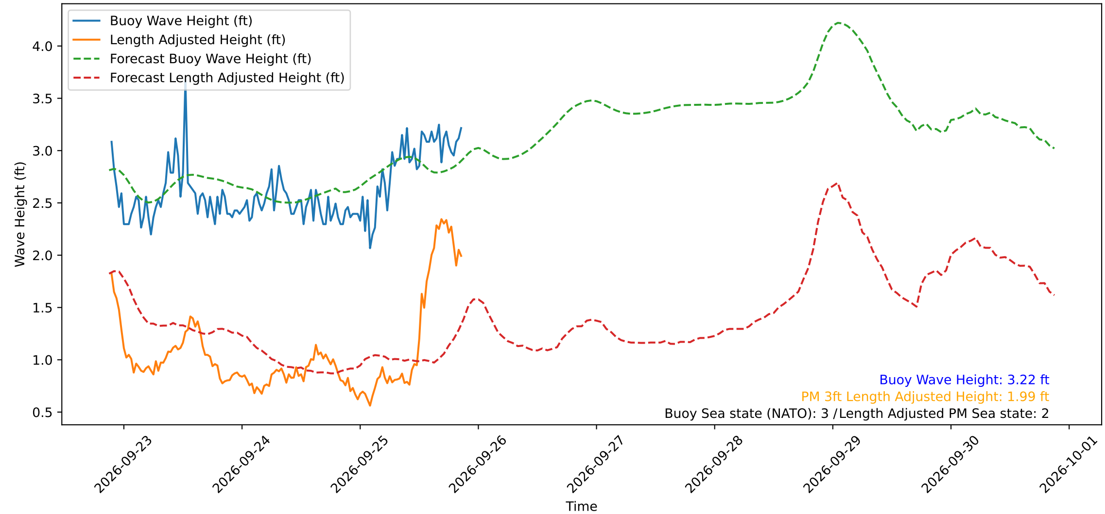
Wave Heights over Time for Red Beach at 2026-09-25 21:20:50
