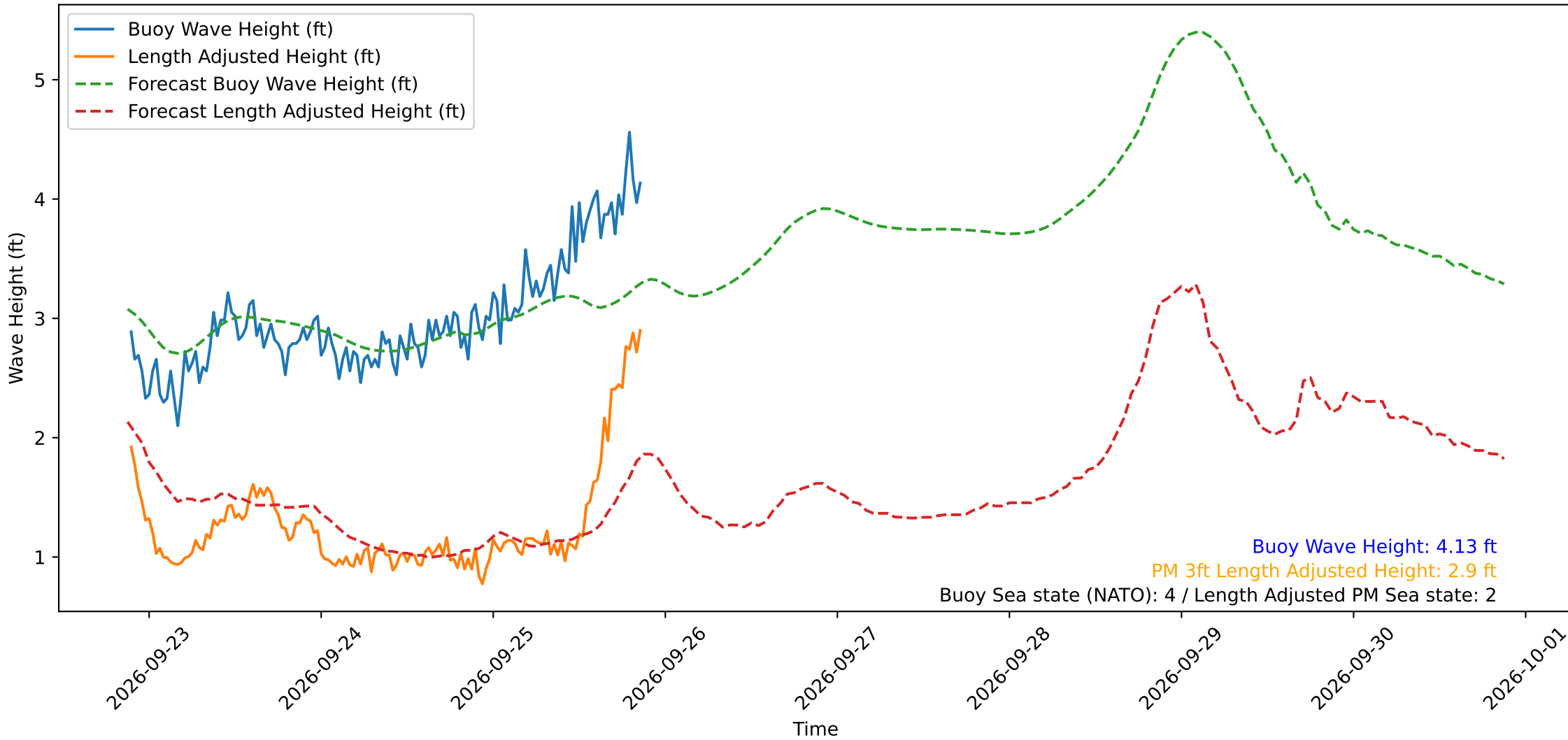
Wave Heights over Time for Green Beach at 2026-09-25 21:21:14
