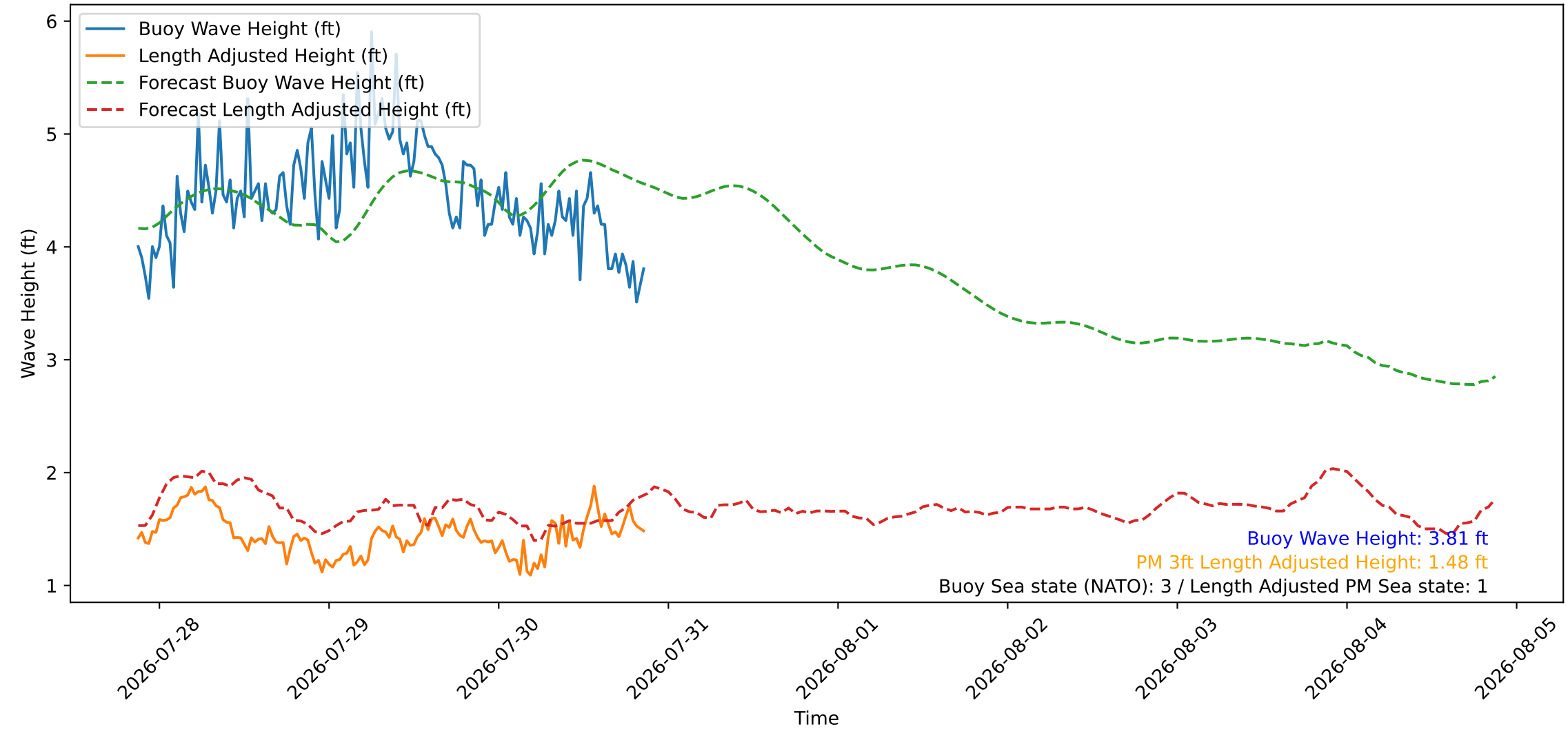
Wave Heights over Time for Oceanside Harbor at 2026-07-30 21:10:26
