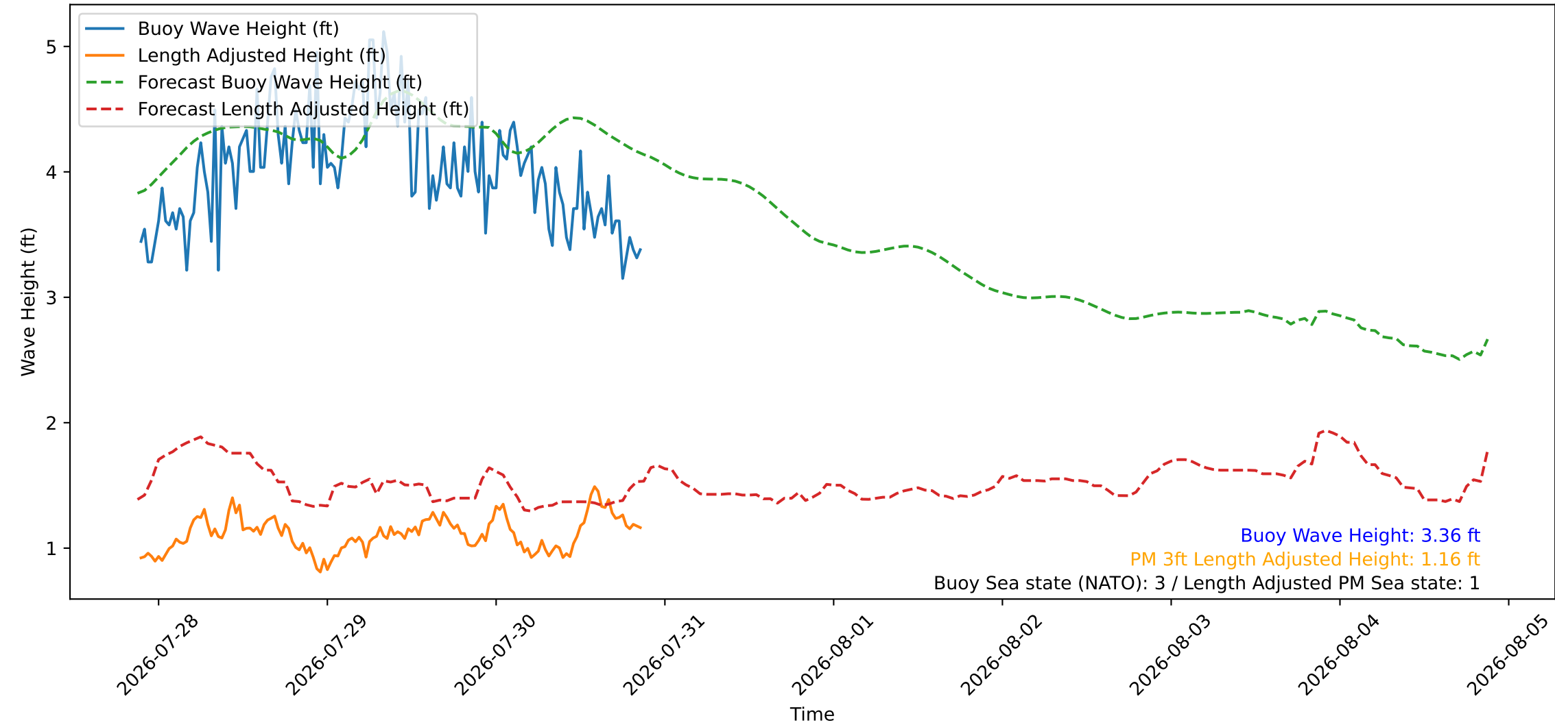
Wave Heights over Time for Red Beach at 2026-07-30 21:10:46
