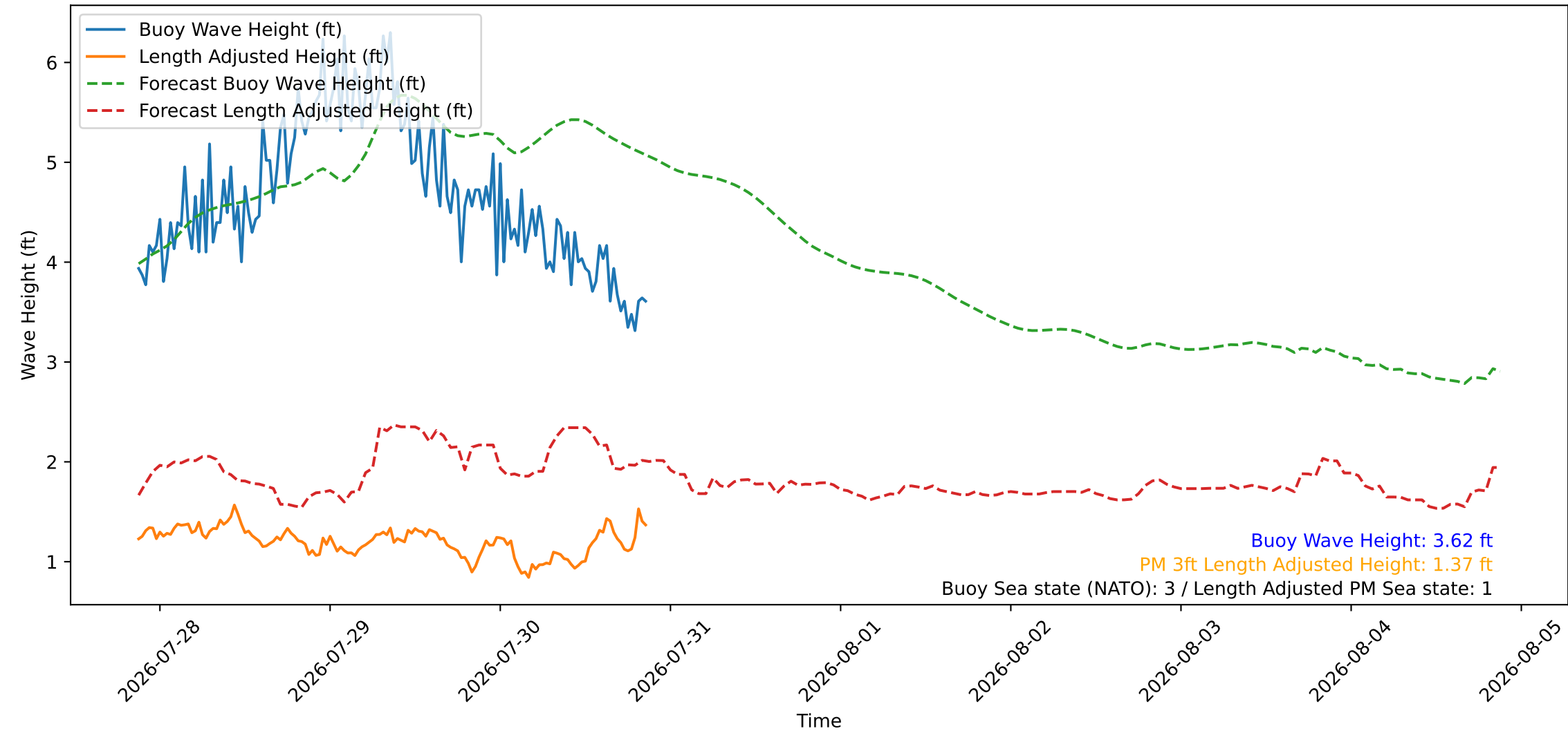
Wave Heights over Time for Green Beach at 2026-07-30 21:11:09
