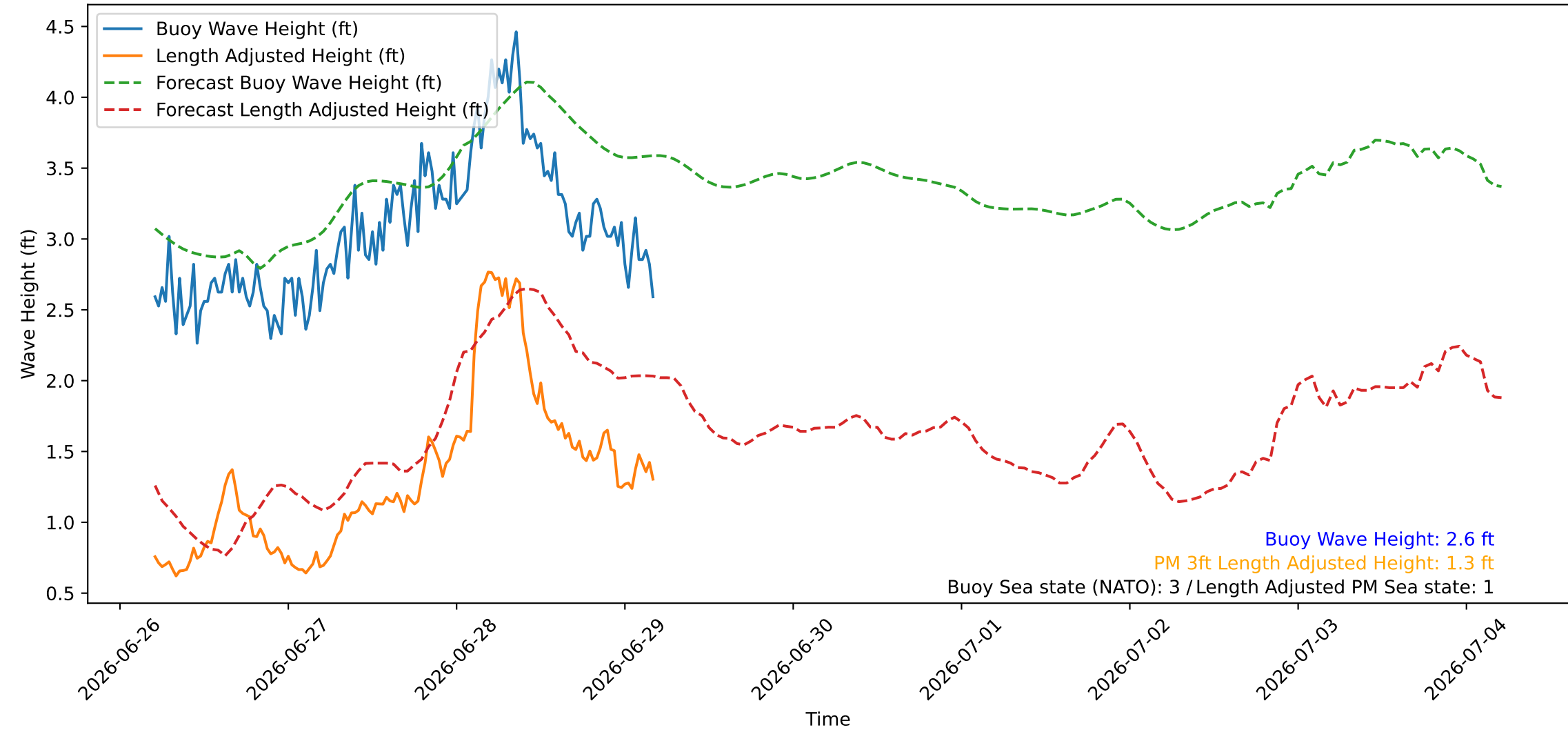
Wave Heights over Time for Red Beach at 2026-06-29 04:40:45
