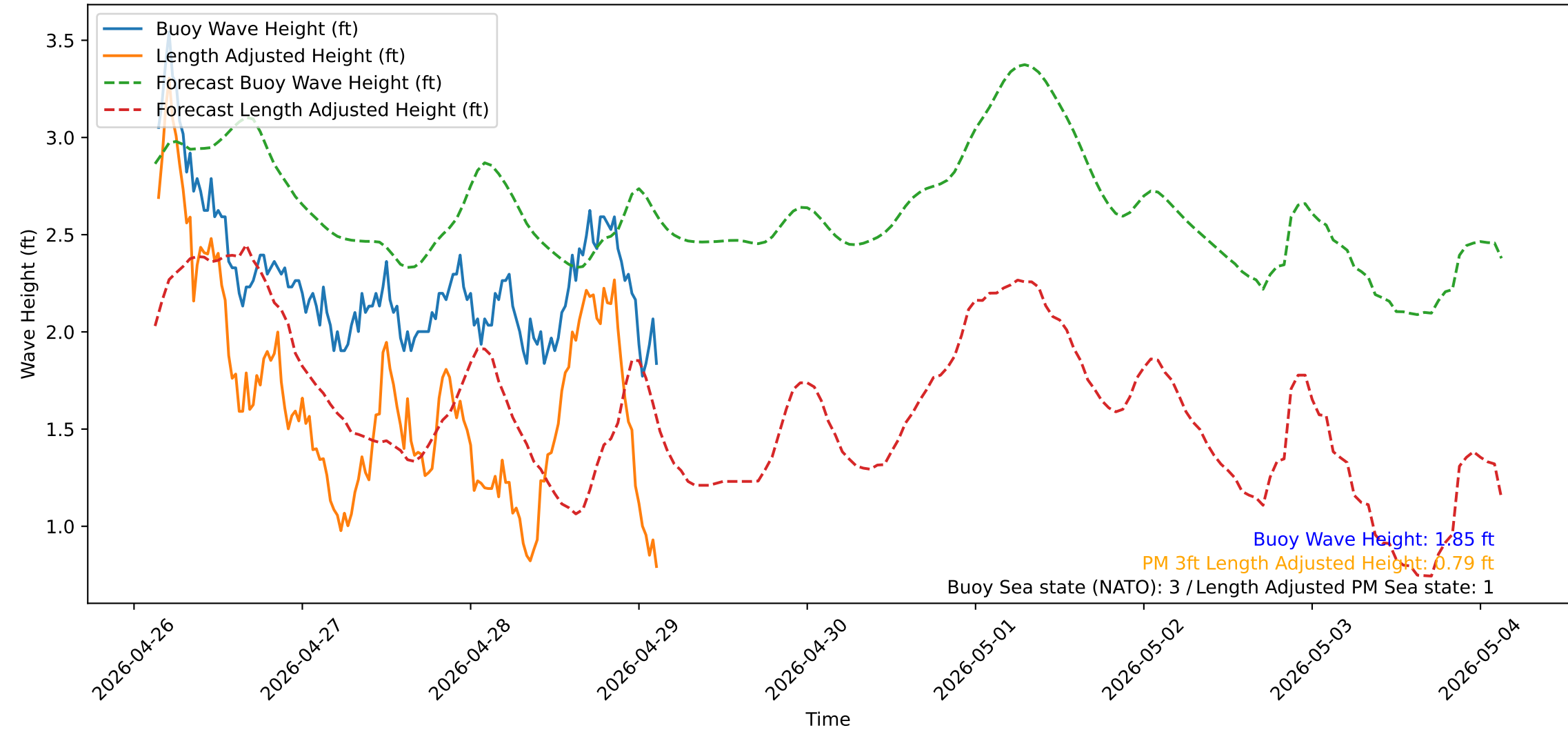
Wave Heights over Time for Red Beach at 2026-04-29 03:20:51
