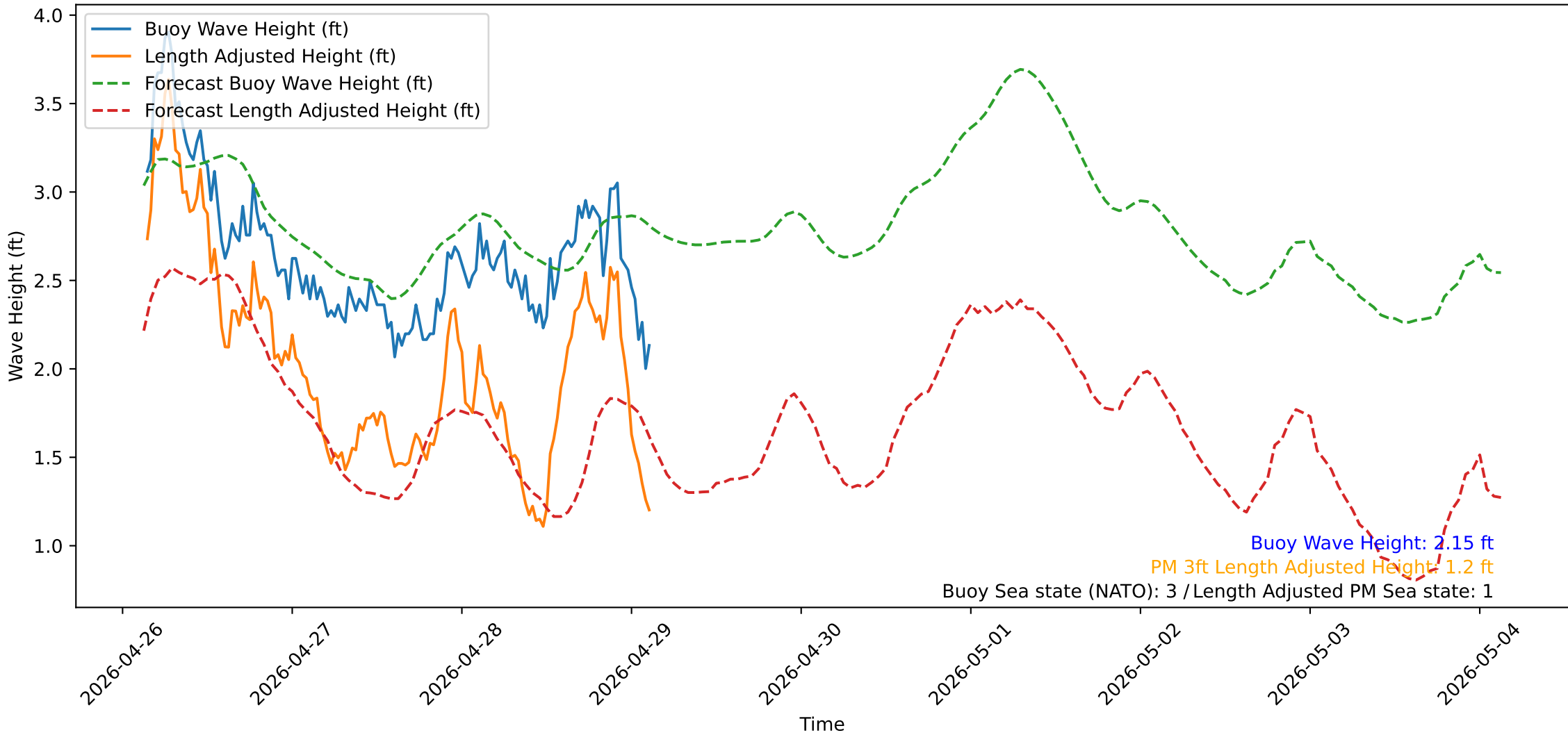
Wave Heights over Time for Oceanside Harbor at 2026-04-29 03:20:31
