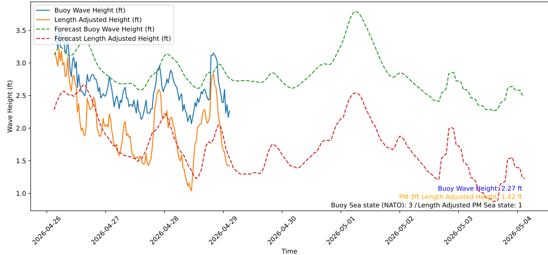
Wave Heights over Time for Green Beach at 2026-04-29 03:21:14
