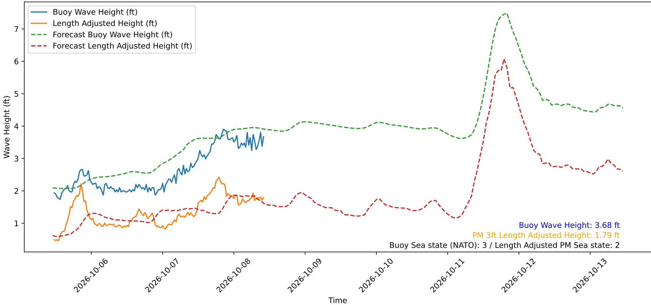
Wave Heights over Time for Red Beach at 2026-10-08 11:00:50
