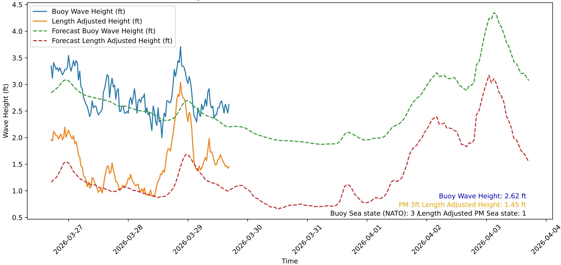
Wave Heights over Time for Green Beach at 2026-03-29 17:11:10
