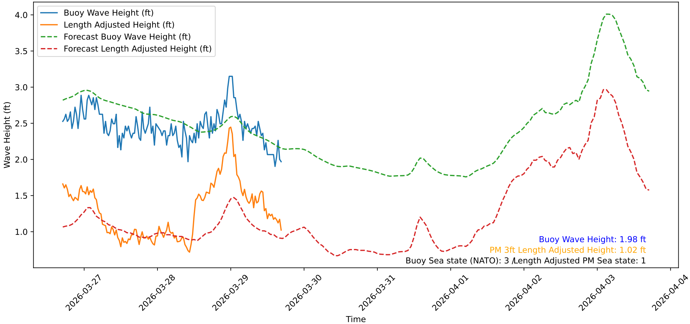
Wave Heights over Time for Oceanside Harbor at 2026-03-29 17:10:31
