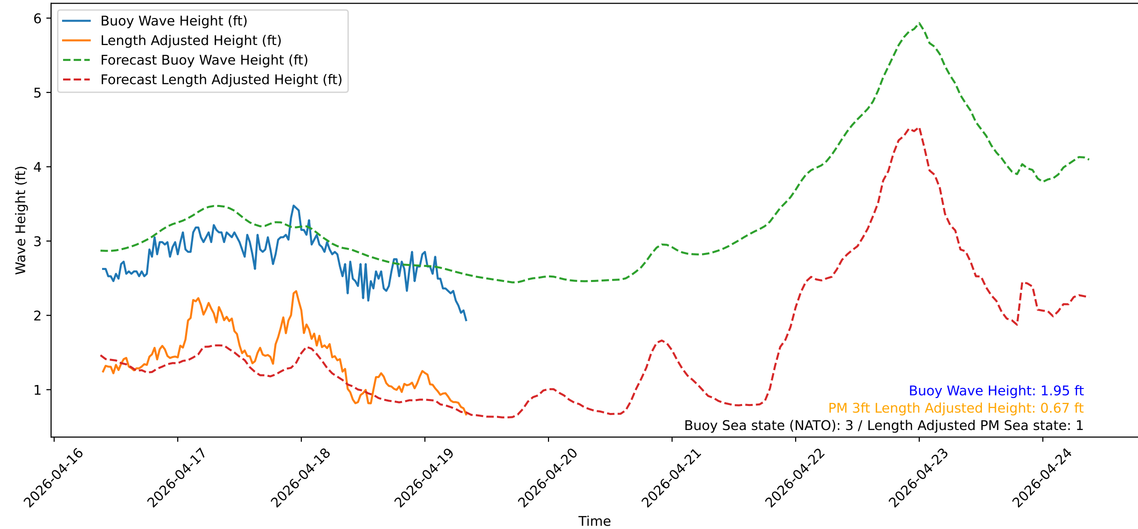
Wave Heights over Time for Green Beach at 2026-04-19 09:21:14
