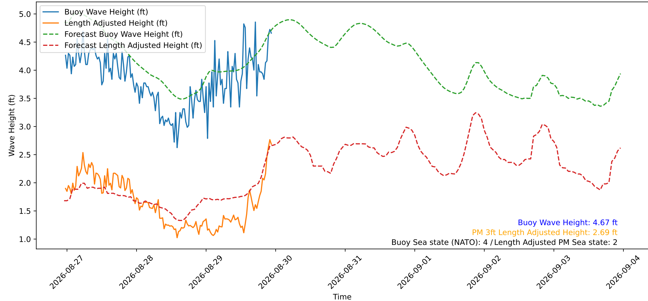
Wave Heights over Time for Green Beach at 2026-08-29 23:21:15
