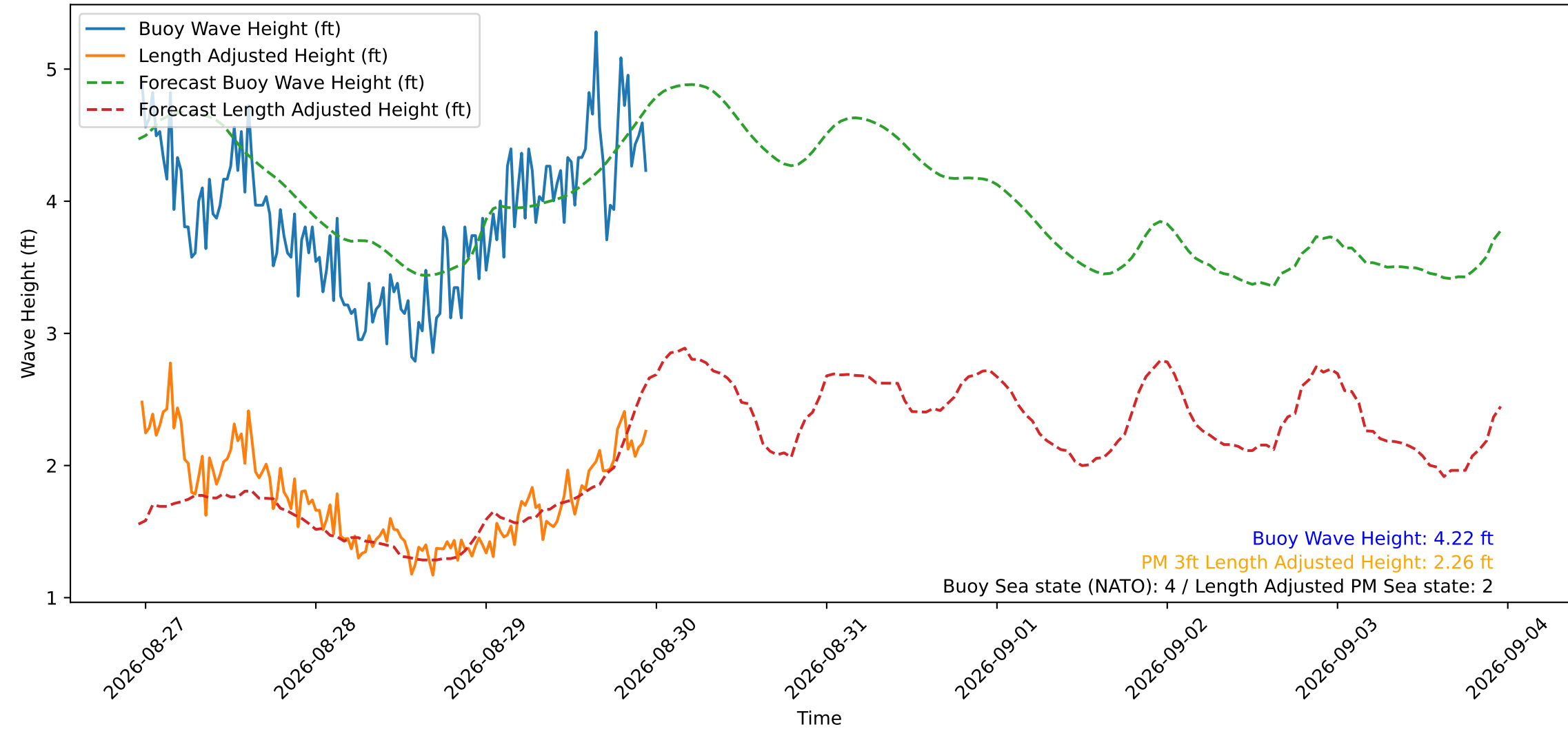
Wave Heights over Time for Oceanside Harbor at 2026-08-29 23:20:29
