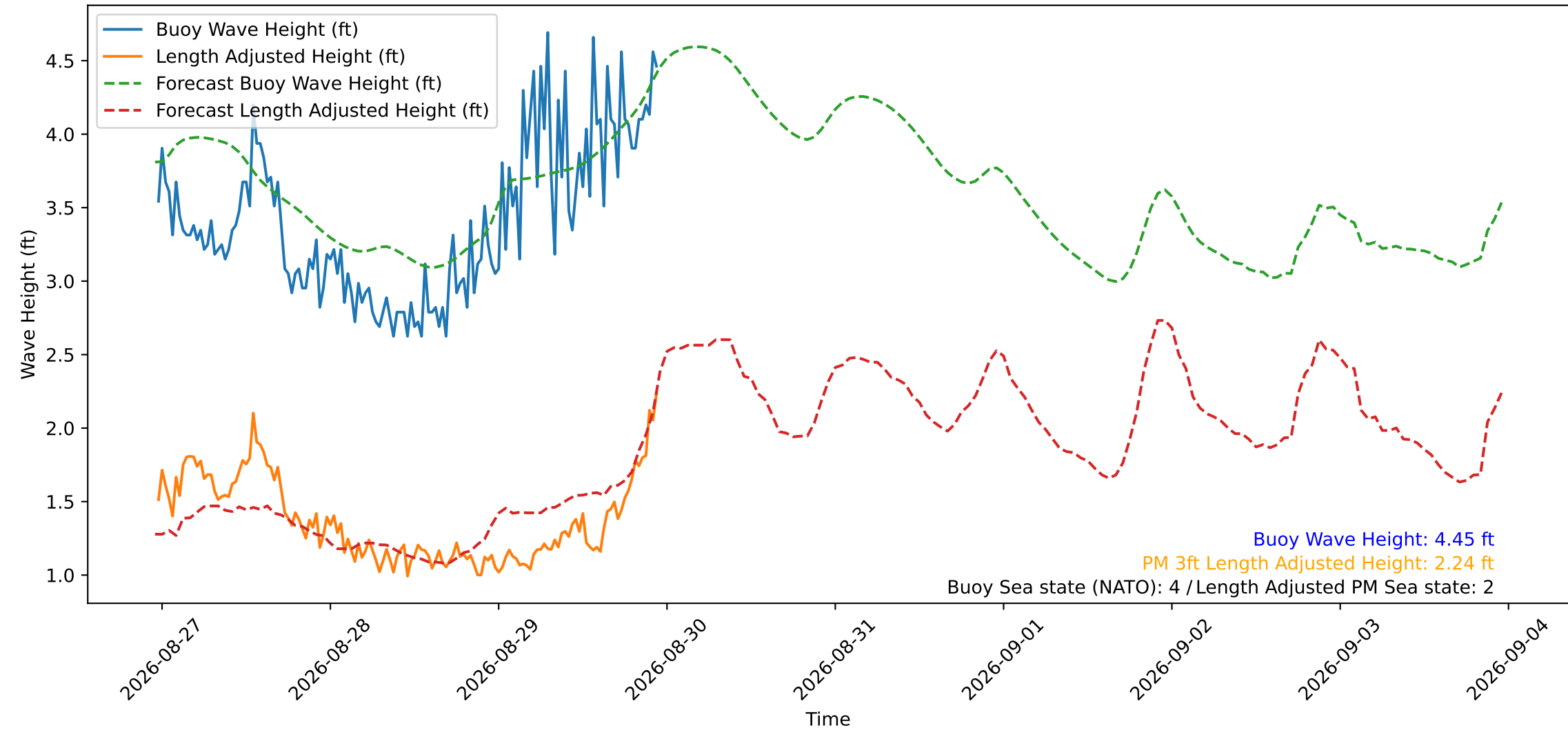
Wave Heights over Time for Red Beach at 2026-08-29 23:20:51
